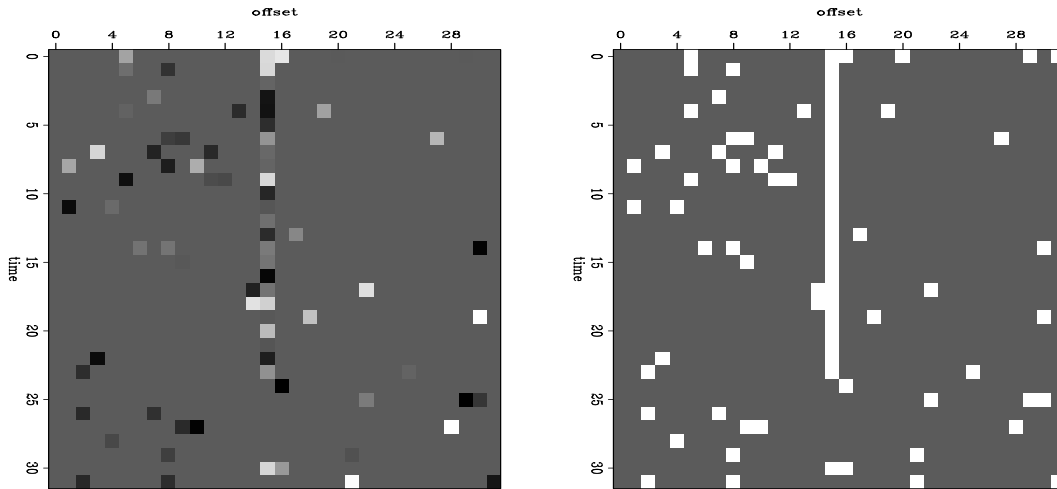
Figure 2: Left: Collected data - one known trace, about 60 randomly-selected known data points. Right: Known data selector. test-data [ER]
