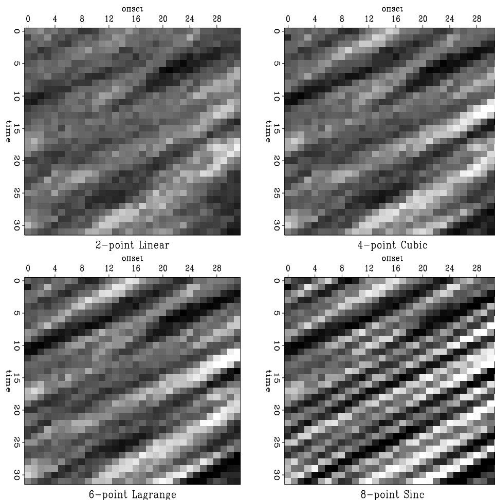
Figure 4: Interpolation schemes compared. Deconvolution of random image with labeled steering filters. test-interp-comp [ER]
