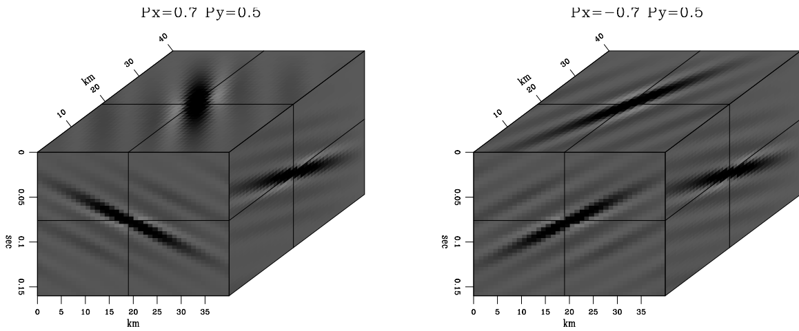
Figure 1: 3-D plane wave prediction with a 402-point filter. Left: p_x = 0.7, p_y = 0.5 . Right: p_x = -0.7, p_y = 0.5 . plane-eplane [ER]
