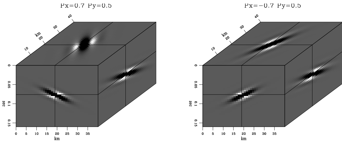
Figure 3: 3-D plane wave prediction with a 26-point filter. Left: p_x = 0.7, p_y = 0.5 . Right: p_x = -0.7, p_y = 0.5 . plane-tplane [ER]
