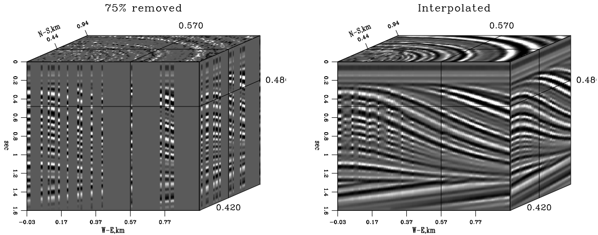
Figure 9: Left: “qdome” model with 75% of the randomly chosen traces removed. Right: result of missing data interpolation with a 3-D local plane-wave prediction filter. plane-qmiss [CR]
