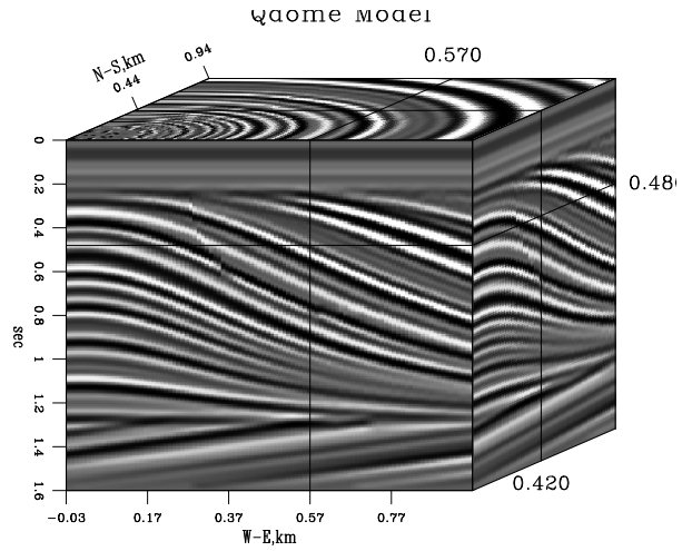
Figure 7: Claerbout's "qdome" synthetic model. plane-qdome [ER]
