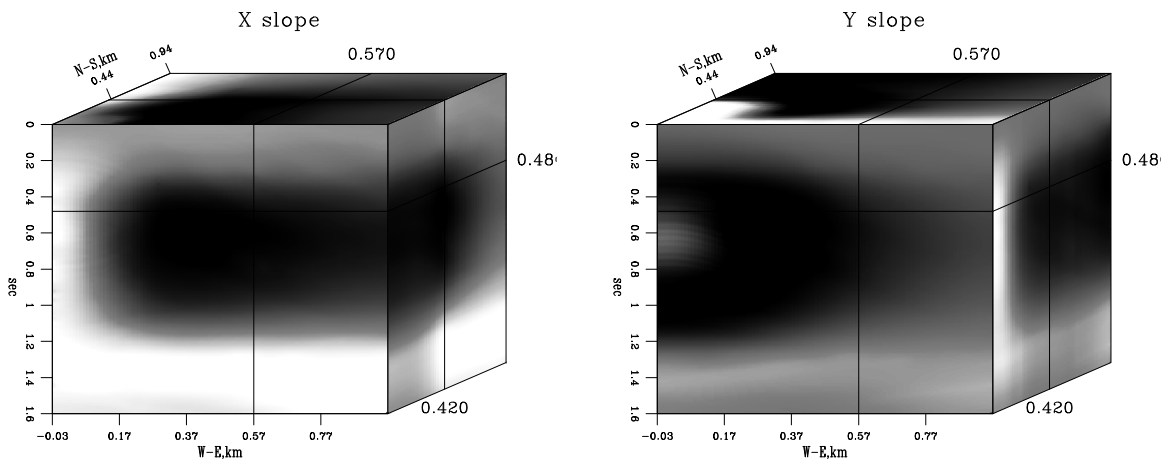
Figure 8: Plane wave slope estimates in the x and y directions (left and right plots, respectively) from the "qdome" model. plane-qslope [CR]
