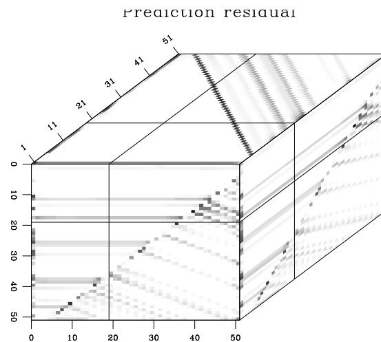
Figure 6: Magnitude of the residual after convolving the synthetic two-plane model with a local 3-D plane wave filter. plane-cmain [ER]
