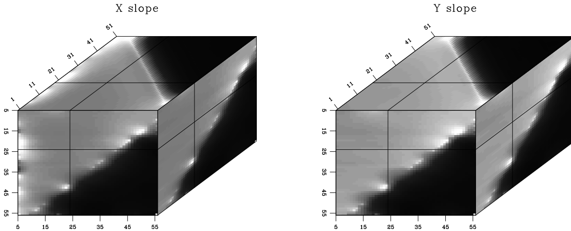
Figure 5: Plane wave slope estimates in the x and y directions (left and right plots, respectively) from the synthetic two-plane model. plane-cslope [ER]
