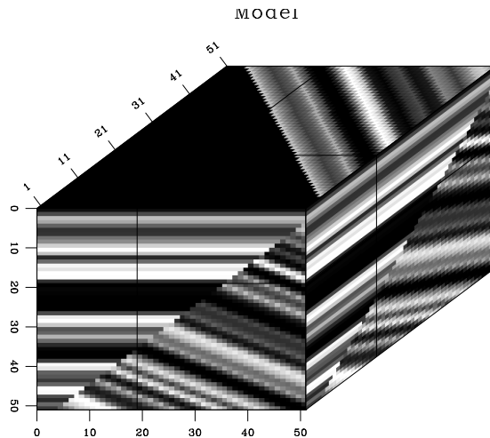
Figure 4: A synthetic model, showing a fault between two plane waves of different slopes. plane-cube [ER]
