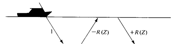
FIGURE 8-3 An initial downgoing disturbance 1 results in a later upgoing reflected wave -R(Z) which reflects back down as R(Z) . The pressure at the surface is D + U = 1 + R - R = 1 .
