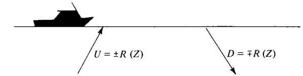
FIGURE 8-2 A waveform R(Z) reflecting at the surface of the sea. Pressure equal to U + D vanishes at the surface. The vertical velocity of the surface is proportional to D - U . Theoretically, waves are observed by measuring W at the surface; however, as a practical matter P is often observed a fraction of a wavelength below the surface.
