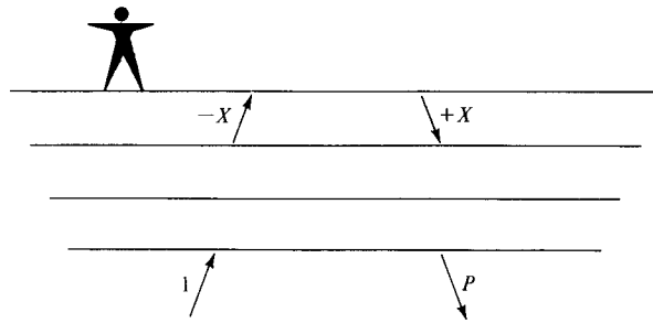
FIGURE 8-8 Earthquake seismology geometry. An impluse 1 is incident from below. The waveform X(Z) is incident upon the free surface and is reflected back down. The waveform P(Z) scatters back into the earth.
