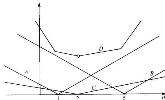
FIGURE 6-3 A sum of weighted absolute value norms. The function labeled A is .5|m - 1| , B is .5|m - 5| , C is .1|m - 2| , and D is the sum of A , B , and C . The sum D is minimized at m = 2 , a point which exactly solves C = 0 = .1|m - 2| .
