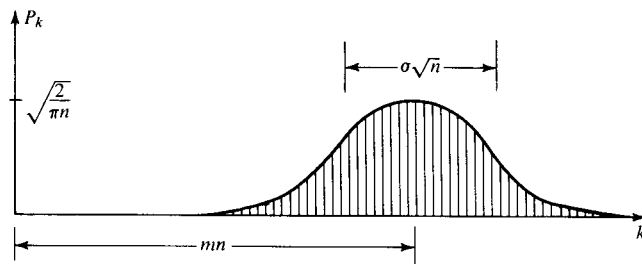
FIGURE 4-9 Coefficients of [Z^m(Z^\sigma + Z^{-\sigma})/2]^n .
