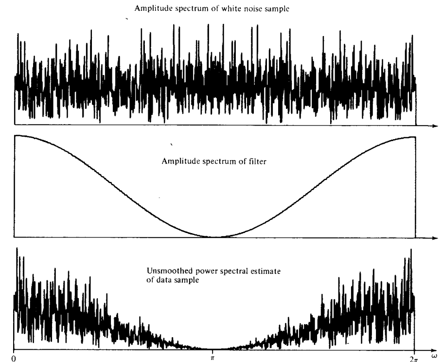
FIGURE 4-5 Spectral estimation.
