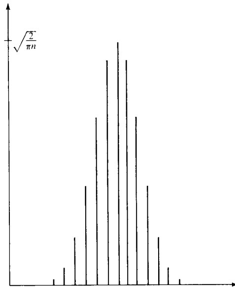
FIGURE 4-1 Binomial coefficients tend to the gaussian function. Plotted are the coefficients of Z^t in (.5 + .5Z)^{20} .
