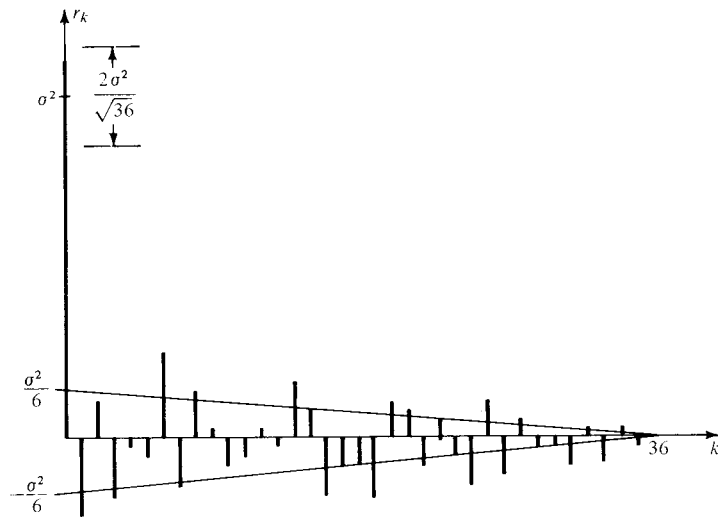
FIGURE 4-3 Positive lags of autocorrelation of 36 random numbers.
