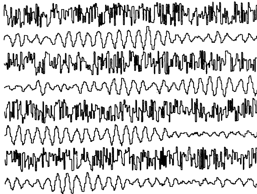
FIGURE 4-7 1,024 random numbers before and after narrowband filtering. The filter was (1-Z)/[i(1-Z/Z_0)(1-Z/\bar{Z}_0)] where Z_0 = 1.02 e^{i\pi/5} .
