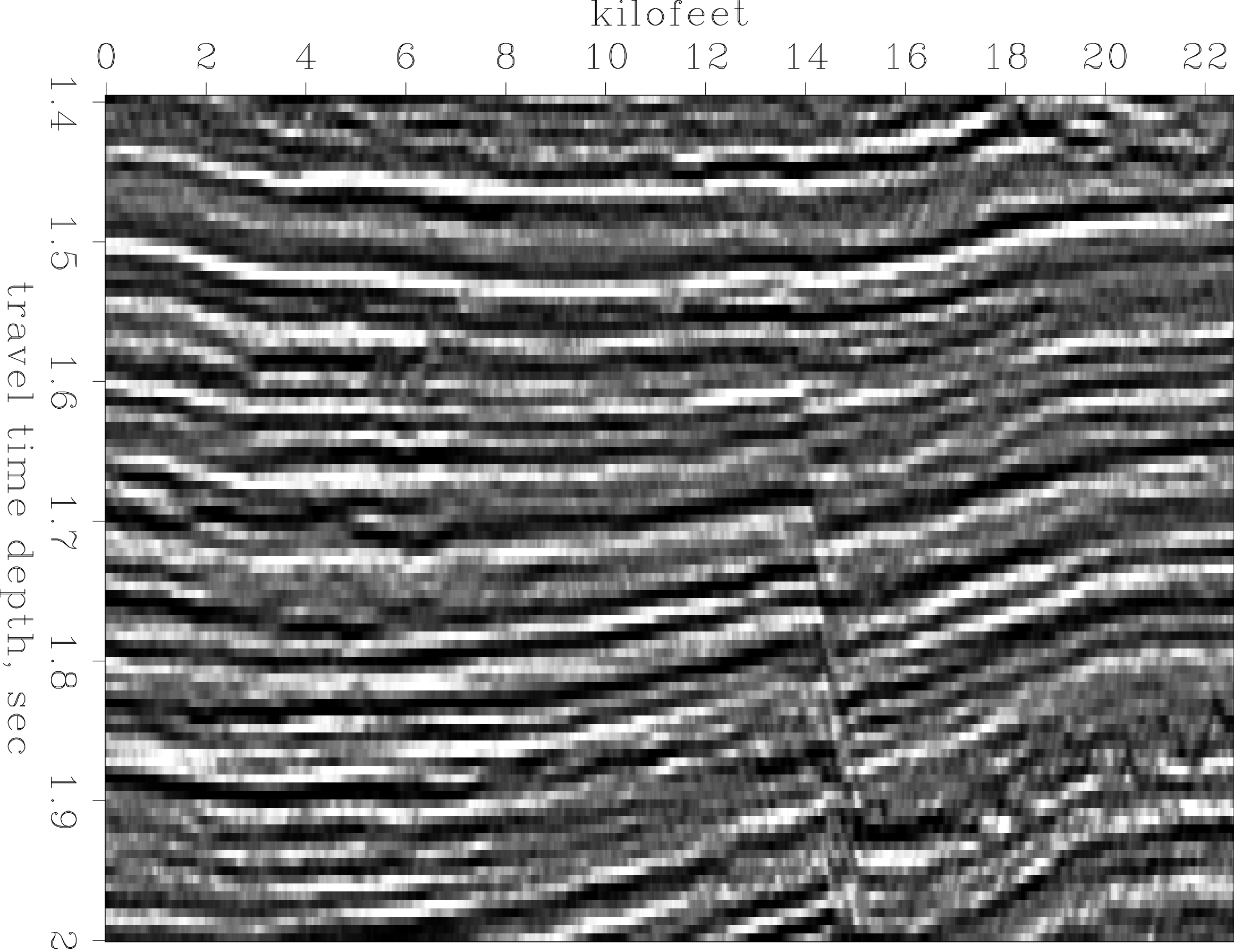
2-D line with fault
