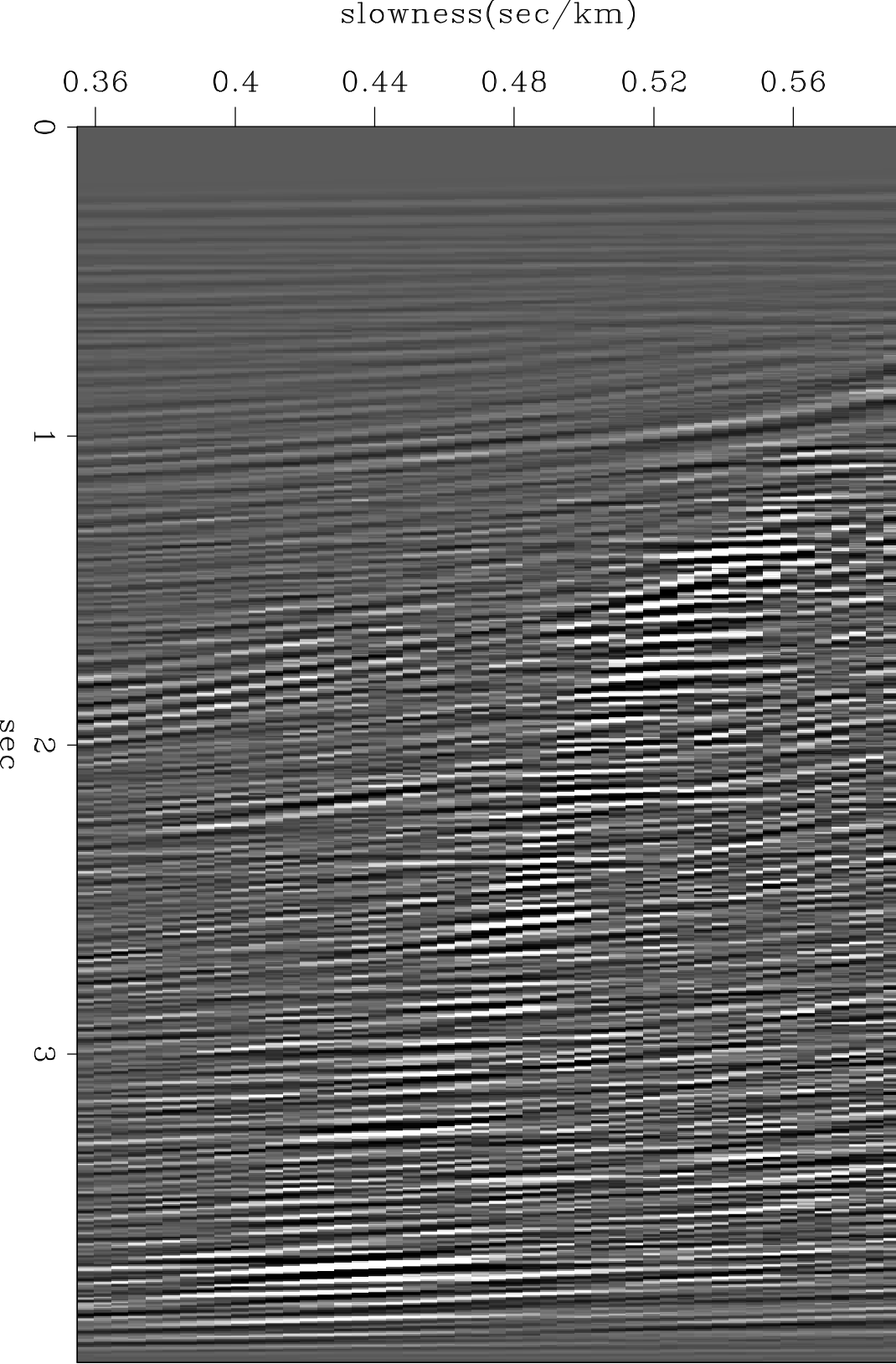
Slowness scan
