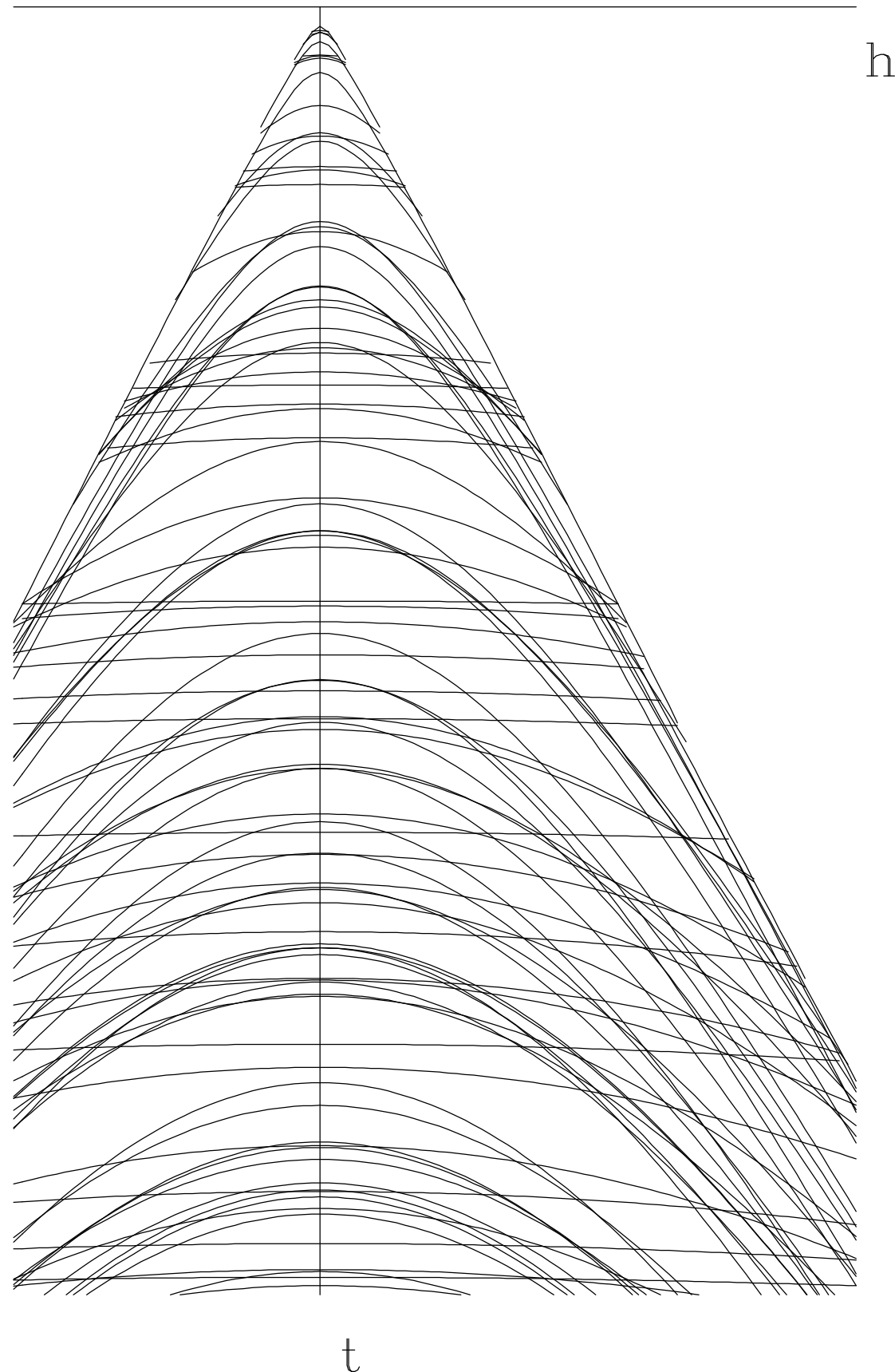
Common Midpoint
