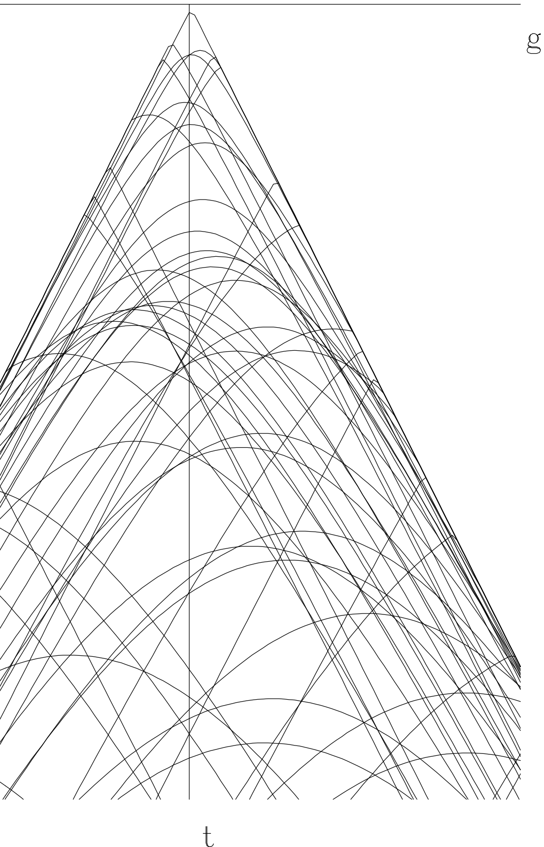
Common Shot
