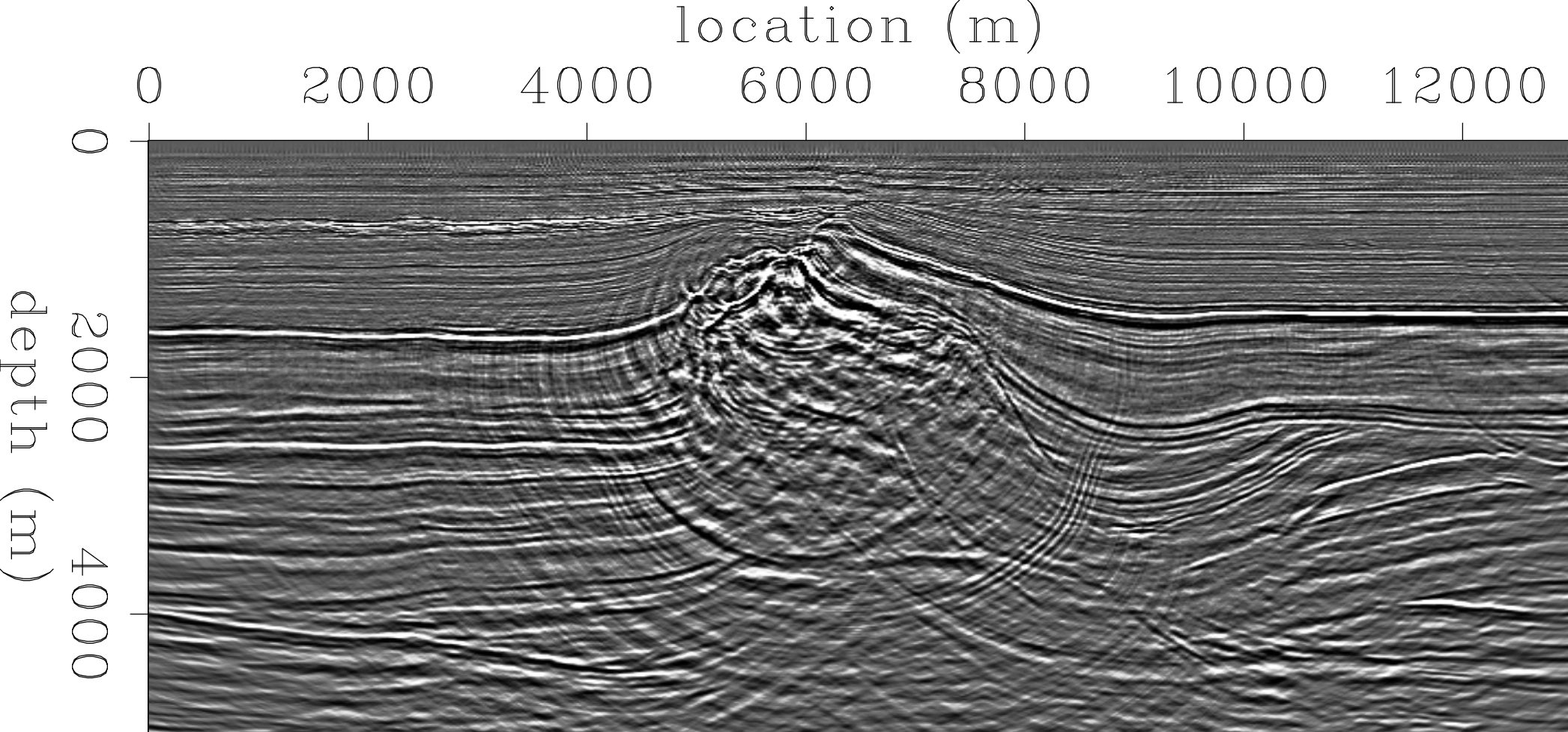
2-D Kirchhoff migration
