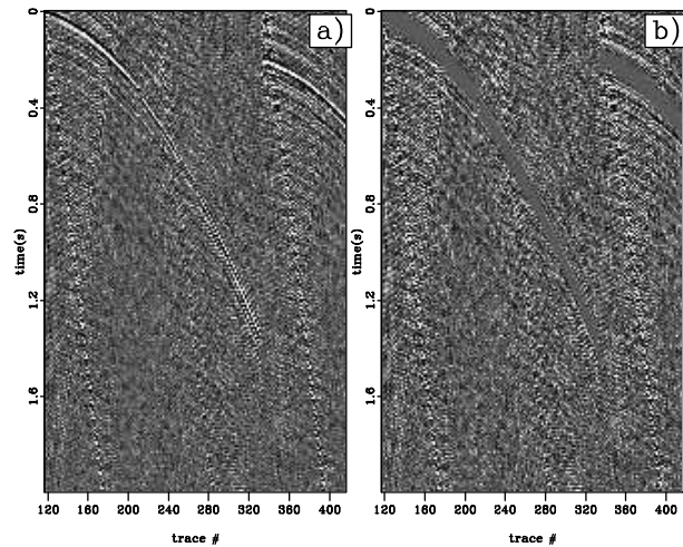
Figure 6.10: a) Synthesized shot gather using 9 hours of passive data. b) Direct arrival from production noise windowed away. DepthVal-noeventdat [NR]
