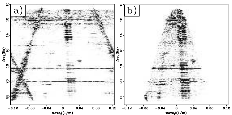
Figure 3.12: Frequency-wavenumber power spectrum of on OBC cable calculated from raw passive data. Panel b shows mute applied to focus on energy near zero wavenumber. TimeShot-fkpow [ER]
