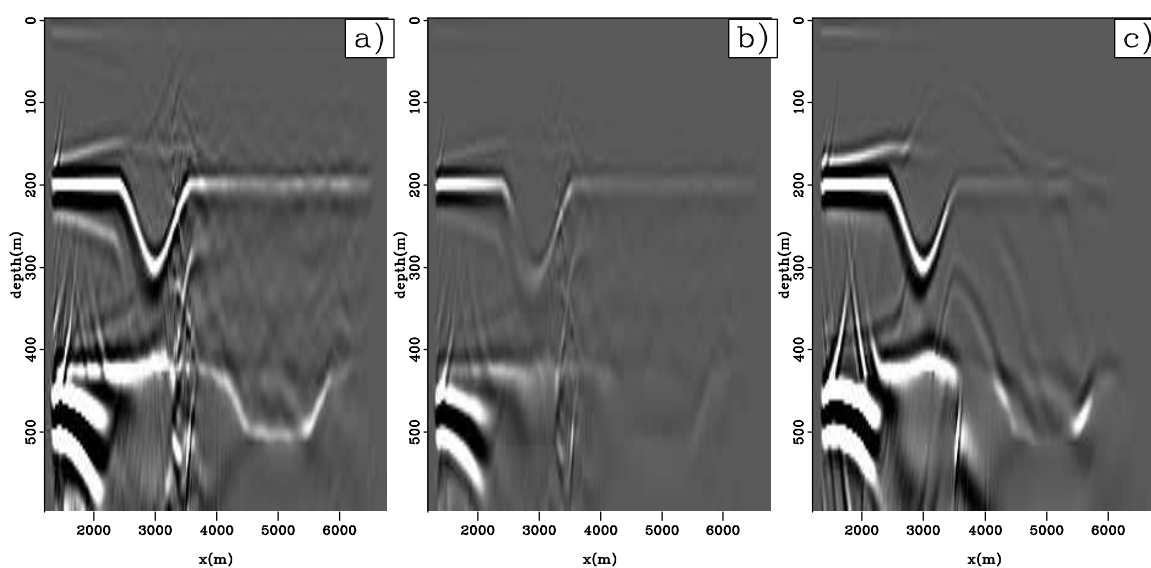
Figure 5.8: a) Direct migration of a transmission wavefield due to an impulsive subsurface source at the left edge of the model domain. b) Migration of synthesized gathers produced with the same transmission wavefield. c) Image produced with the transmission wavefield as data and only the direct arrival as the source. DepthSyn-dmig1200 [CR]
