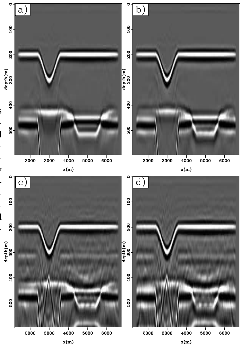
Figure 5.11: Left column shows direct migrations, while right column shows migrations of synthesized gathers. Top row processed impulsive transmission wavefields independently, while the bottom row used a single transmission wavefield generated by summing the transmission wavefields due to randomized subsurface sources distributed densely below the entire model domain. DepthSyn-allcomp [CR]
