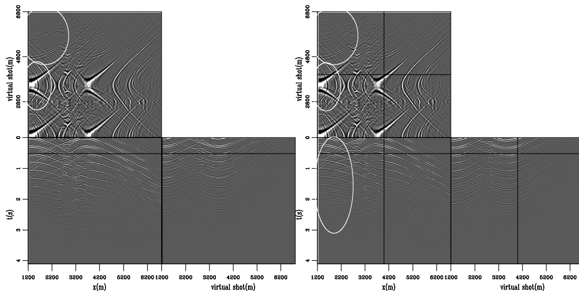
Figure 2.5: Synthesized shot gathers produced by correlating the sum of transmission wavefields due to sources beneath the left edge and middle of the model. Compare artifacts within the ovals to the more correctly processed result in Figure 2.6 TimeSynth-vshot1200.3500 [CR]
