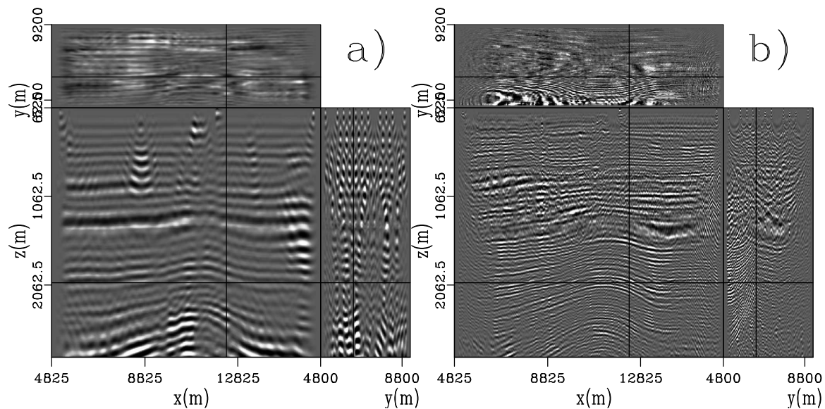
Figure 6.7: Images produced with likely coherent noise sources as data. Panel a was produced with repeated horizontal plane waves, Figure 6.6a. Panel b was produced with repeated far-field production noise, Figure 6.6b. DepthVal-manyimg [NR]
