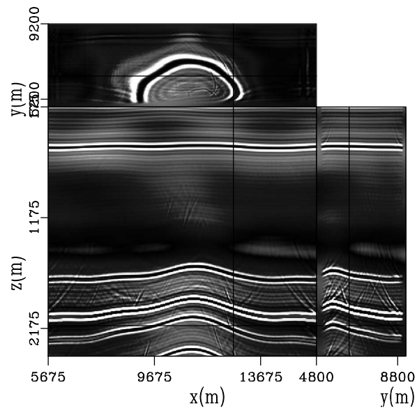
Figure 6.4: Interval velocity model merged with an image produced by migrating 5 horizontal plane waves.
