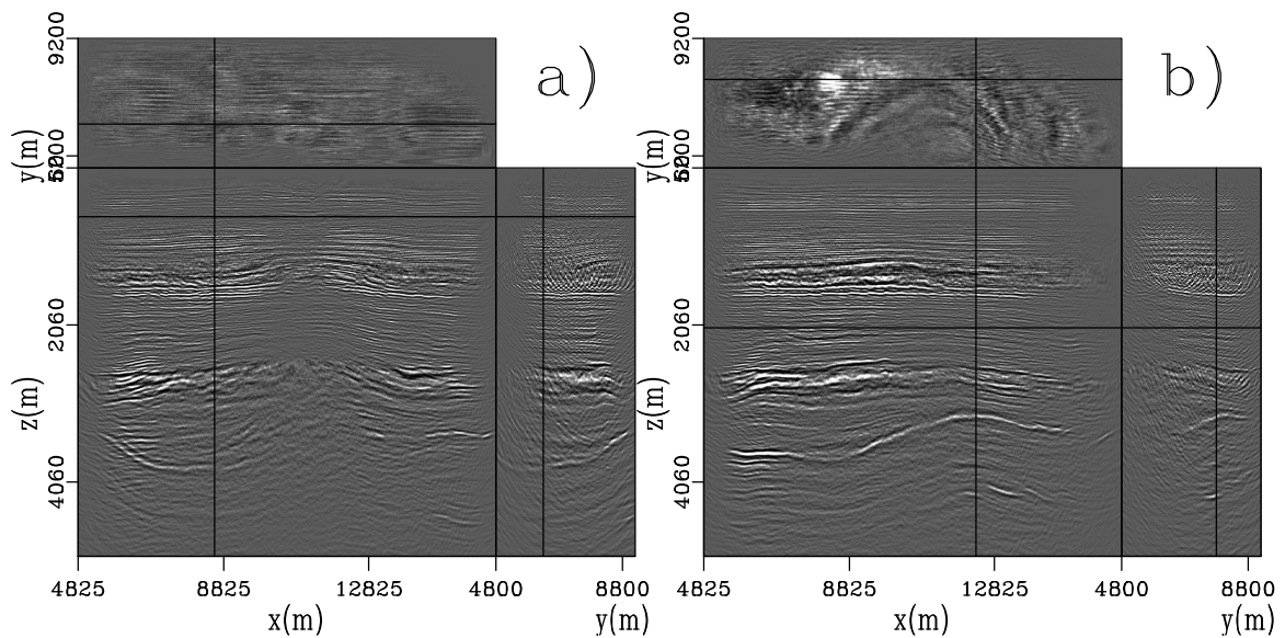
Figure 6.3: Control image produced with active seismic data using only shots locations directly above a receiver location. DepthVal-Vactive [NR]
