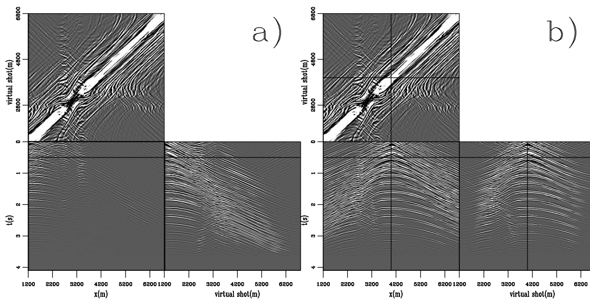
Figure 2.3: Two correlated shot gathers from the volume generated by summing correlations from 225 sources across the bottom of the model. TimeSynth-allshots [CR]
