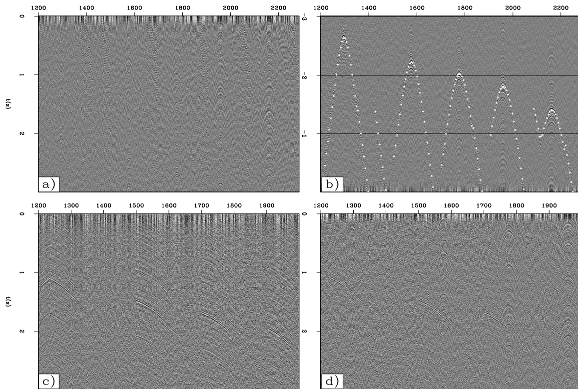
Figure 3.11: Correlated gathers from the Eastern side of the array. Top row: Early causal (a) and acausal lags (b) of a correlated gather using the data in Figure 3.4. Overlays on panel b have the same velocity (1450 m/s) and origin as those delineating the top and bottom boundaries of the noise train in the raw data. Bottom row: Early causal lags of correlated gathers using 12 s of raw data. Panel c used data in Figure 3.3 and panel d used data in Figure 3.5. TimeShot-evtest [CR]
