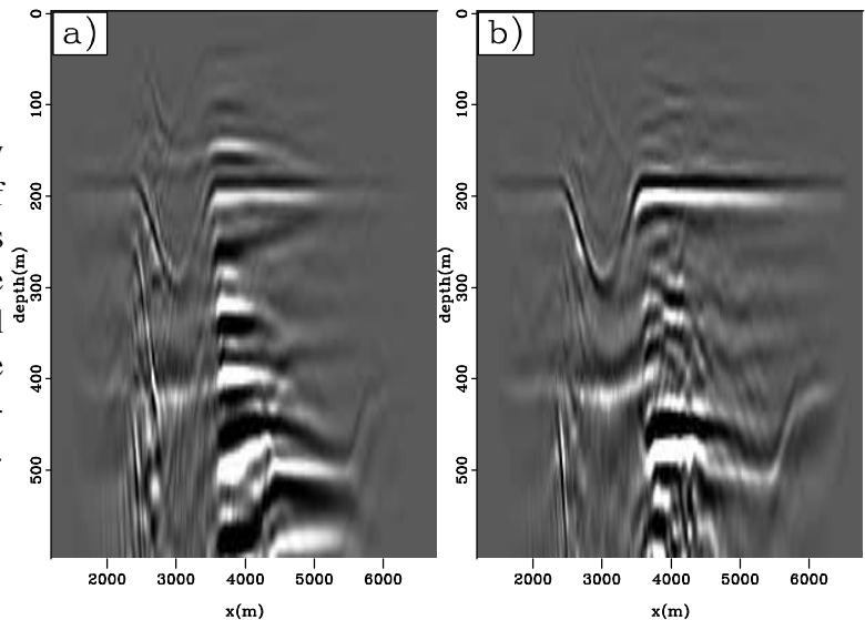
Figure 5.6: Images produced by migrating synthesized gathers of summed transmission wavefields from 30 sources clustered around the center of of the model domain. Panel a used impulsive wavelets, while Panel b was produced after introducing randomized source functions.
