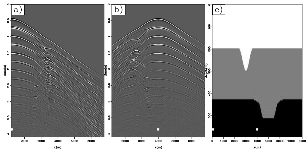
Figure 2.1: Representative transmission wavefields (a,b) from impulsive subsurface sources through a three layer velocity model with two synclines (c). All surface-related and internal multiples are included. Asterisks show subsurface source locations. TimeSynth-data [ER]
