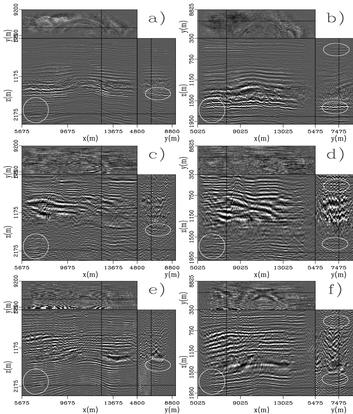
Figure 6.9: a,b) Image produced with active data. b,c) Image produced by direct migration of 100 minutes of passive data. e,f) Image produced with modeled data in Figure 6.6b.
