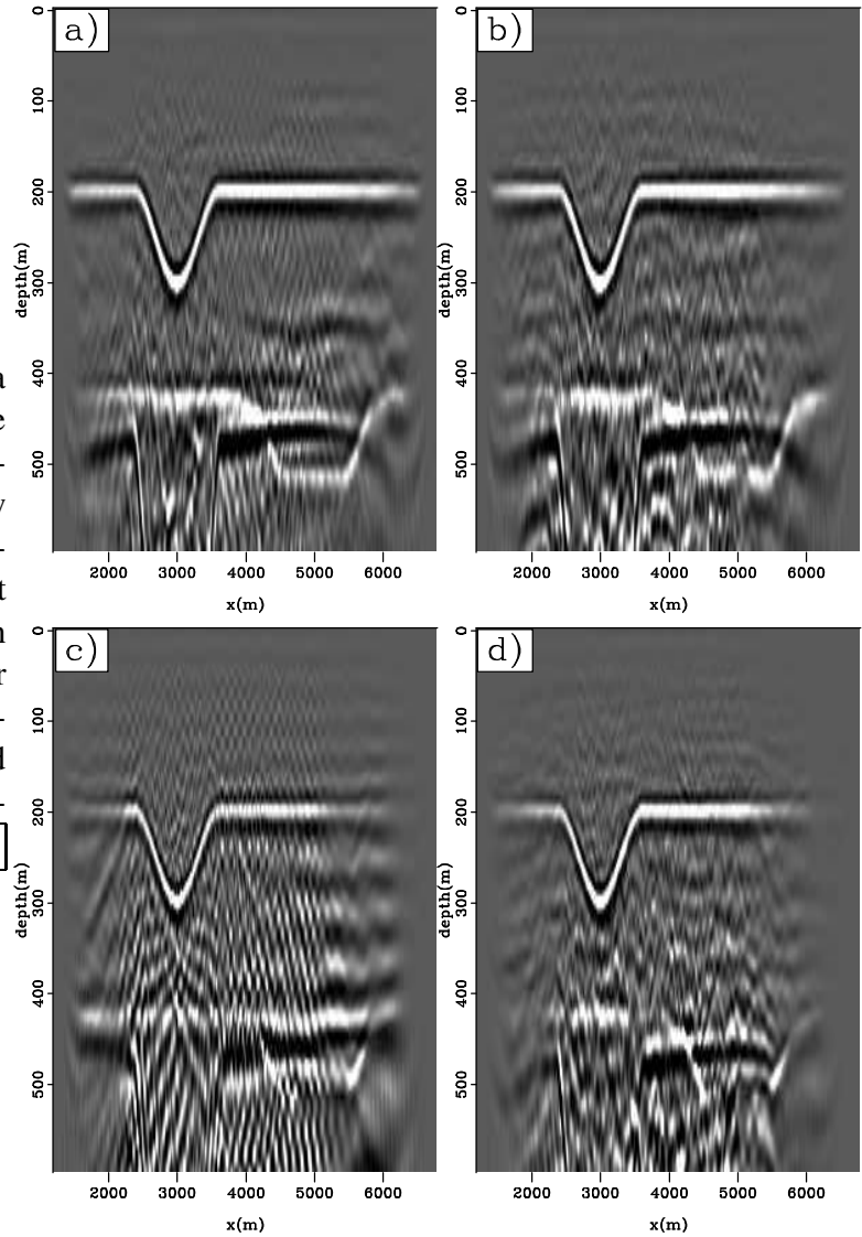
Figure 5.13: Images produced from a transmission wavefield due 30 source clustered around the center of the bottom of the model domain. Top row produced by direct migration. Bottom row produced using the direct arrivals for the source wavefield in the migration. Wavefields used for results in the left column had impulsive wavelets, while those used for the right column had randomized wavelets. DepthSyn-dmigsmall [CR]
