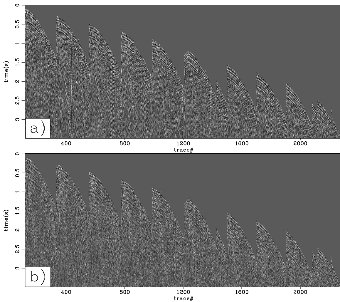
Figure 4.6: Top:Muted shot gather corresponding to the first 9 hours of data (Figure 4.4 top). Bottom: Muted shot gather generated with 5 hours of data 25 hours after those used to create the top panel. TimeCMP-modl.dat [NR]
