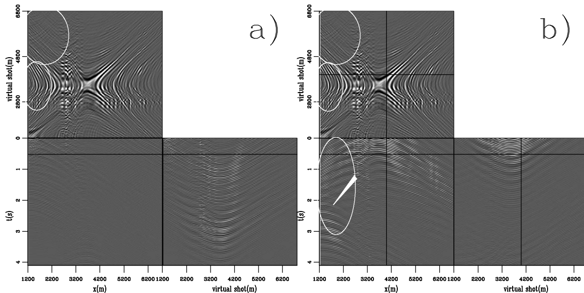
Figure 2.8: Synthesized shot gathers produced by correlating the sum of transmission wavefields due to randomized sources beneath the left edge and middle of the model.
