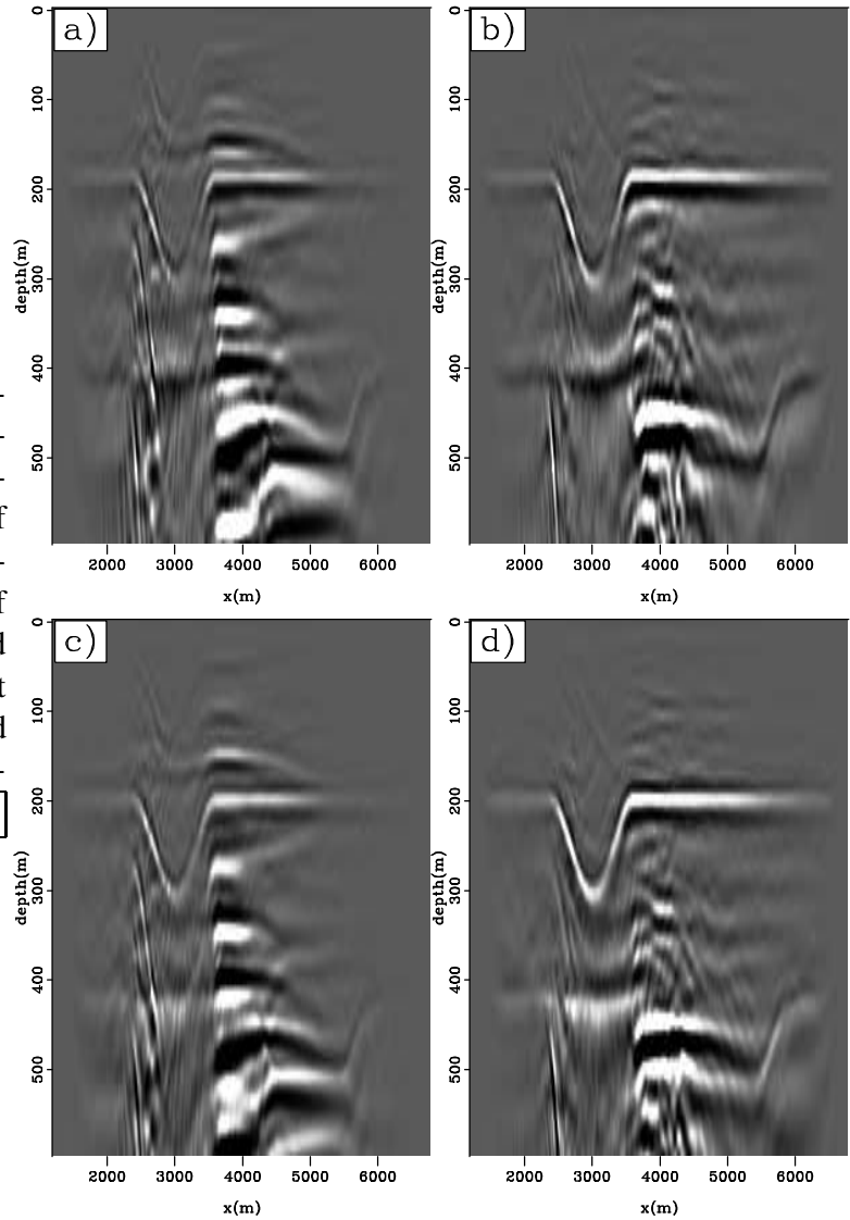
Figure 5.16: Comparison of processing strategies to image a transmission wavefield due to 25 sources distributed evenly across the bottom of the domain. Top: Migration of correlations. Bottom: Direct migration of the wavefield. Left column summed wavefields as modeled, while right column convolved each wavefield with a random wavelet before summing. DepthSyn-smallsmallcomp [CR]
