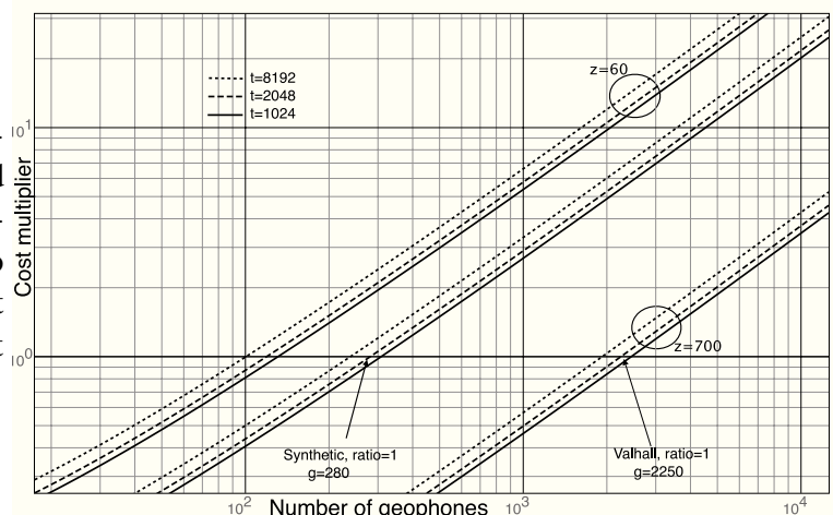
Figure 5.18: Cost ratio of processing a single transmission wavefield by synthesizing shot gathers or imaging with direct migration. Cost ratio values greater than 10^0 indicate that it is more expensive to synthesize shot gathers. DepthSyn-cost2 [NR]
