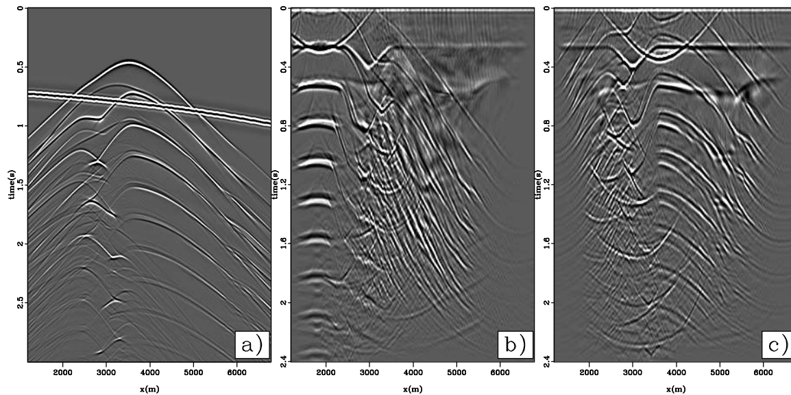
Figure 4.9: a) Transmission wavefield from the modeled data presented in Chapter 2 due to a source below the center of the domain. b) NMO-stack image produced from a transmission wavefield due to a source below the left edge of the domain. c) Stacked time image produced from the transmission wavefield in panel a. TimeCMP-synNMO [NR]
