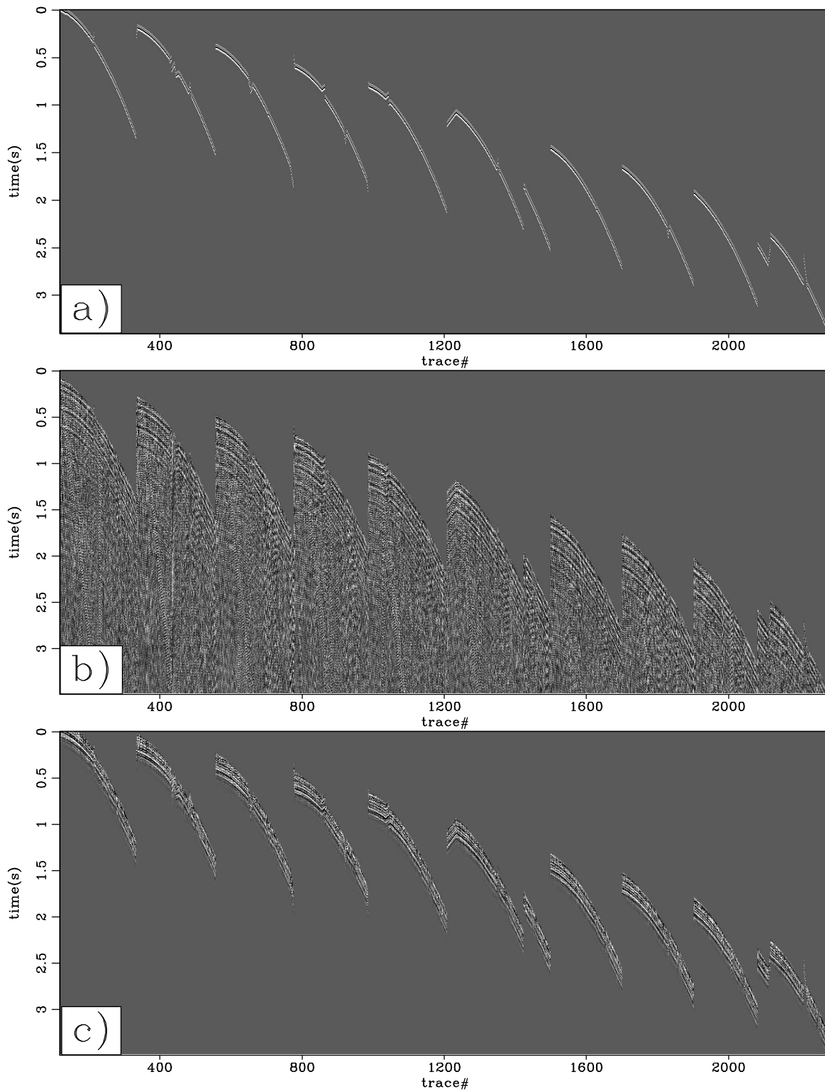
Figure 4.4: Shot gathers used to test the origin of the events in Figure 4.1. Panel a is a modeled shot gather using the inversion results presented in Chapter 3. Panel b is muted to the kinematics of the distant noise source. Panel c is a short window of data around the modeled event. TimeCMP-modldat [NR]
