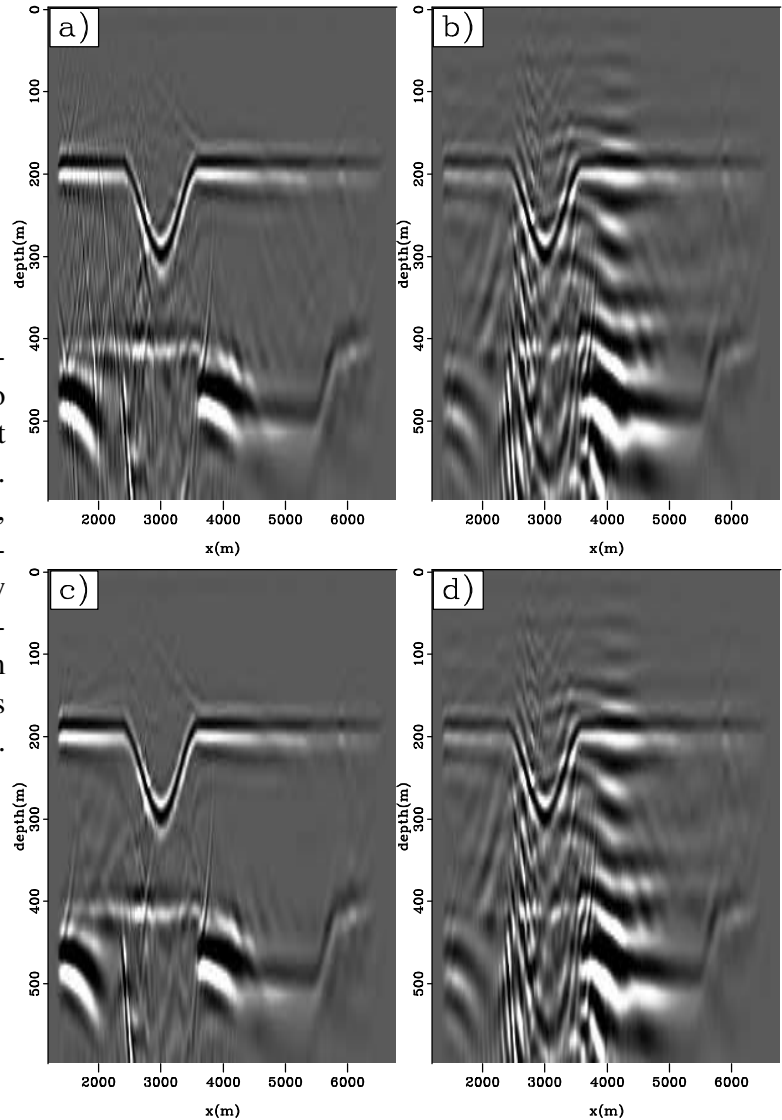
Figure 5.4: Images obtained by migrating correlation volumes due to two sources (located below the left edge and center of model domain). Left column used impulsive sources, while source functions were randomized for the right column. Top row was produced with summed transmission wavefields, and the bottom row by summing the correlations of single transmission wavefields. DepthSyn-mig.shot1200.3500 [CR]
