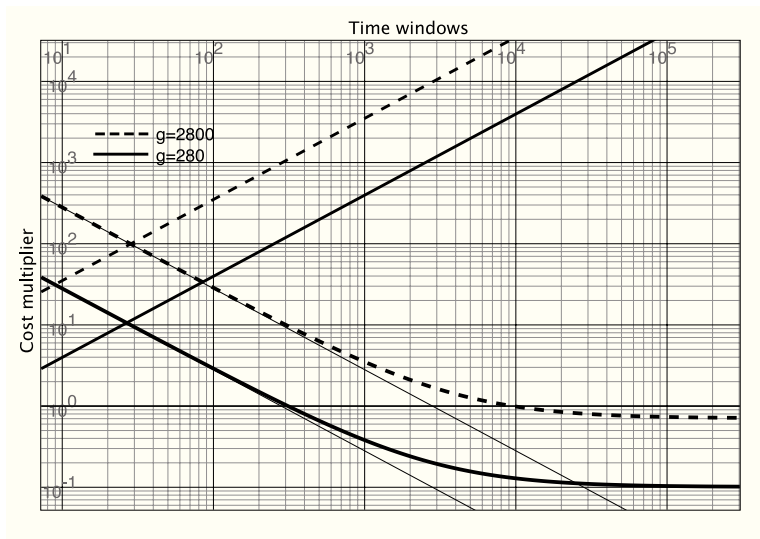
Figure 5.19: Cost ratio of processing many transmission wavefields by synthesizing shot gathers or imaging with direct migration. Cost ratio values greater than 10^0 indicate that it is more expensive to create and migrate synthesized shot gathers.
