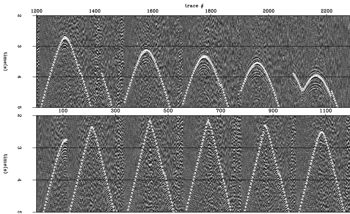
Figure 3.6: Raw data with a clear hyperbolic event annotated with the time calculated for a coplanar direct arrival from the array center traveling at 1450 m/s are. TimeShot-raw3ev [ER]
