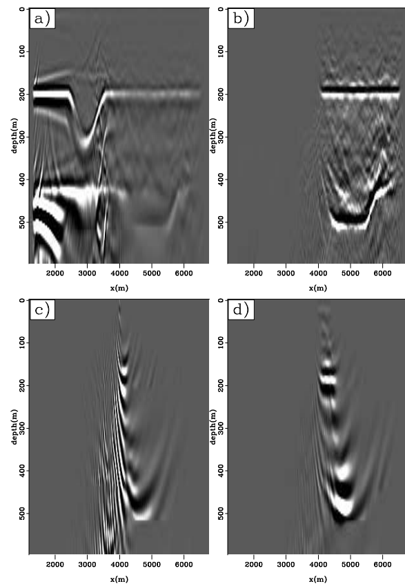
Figure 5.3: a) Image produced by migrating all synthesized gathers from a single transmission wavefield due to an impulsive source at the left edge of the domain. b) Image produce by migrating right half of the total volume of synthesized gathers. c) Migration of synthesized gather with virtual source location x = 4000 m. d) Migration of 20 synthesized gathers from virtual shot locations x = 4000 - 4380 m.
