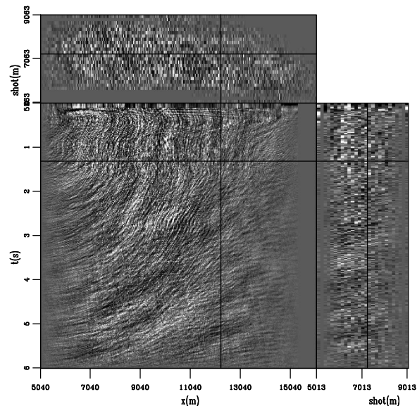
Figure 4.9: NMO-stack image created with only source-receiver trace combinations resulting in negative offset values. By correlating toward the source location, the strong arrival in the synthesized shot gathers is discarded with the acausal correlation lags. TimeCMP-oneside [NR]
