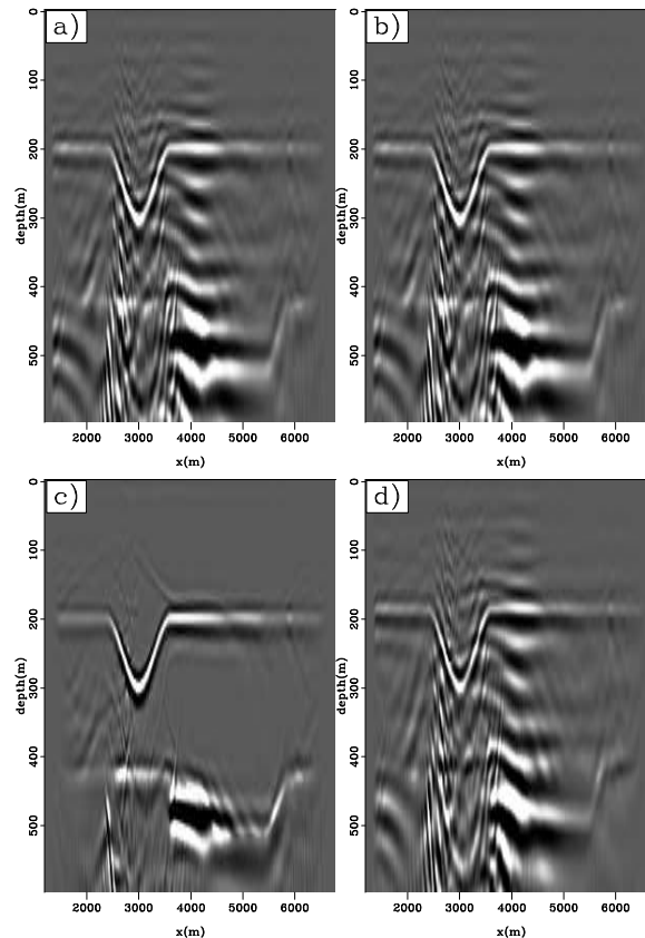
Figure 5.9: a,b) Direct migration of two summed transmission wavefields without and with randomized source functions. c) Sum of images produced by direct migration of individual transmission wavefields. d) Migration of synthesized gathers produced from the summed transmission wavefield.
