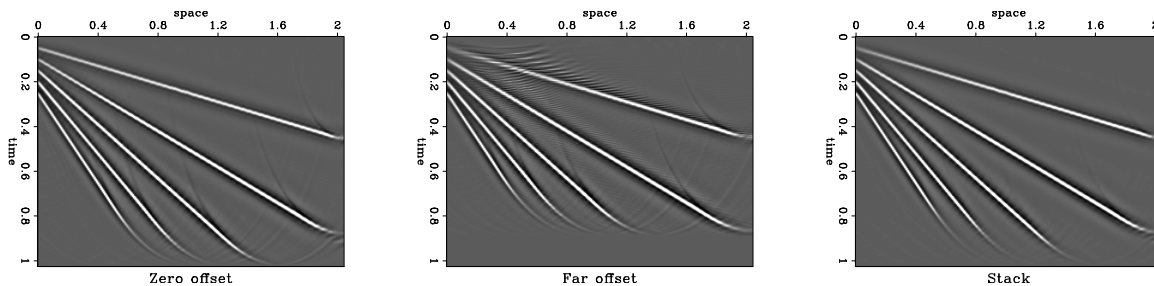
Figure 8: Left: Migrated offset section at zero offset. Center: Migrated offset section at far offset. Right: Stack. angle-offset.lines [ER]
