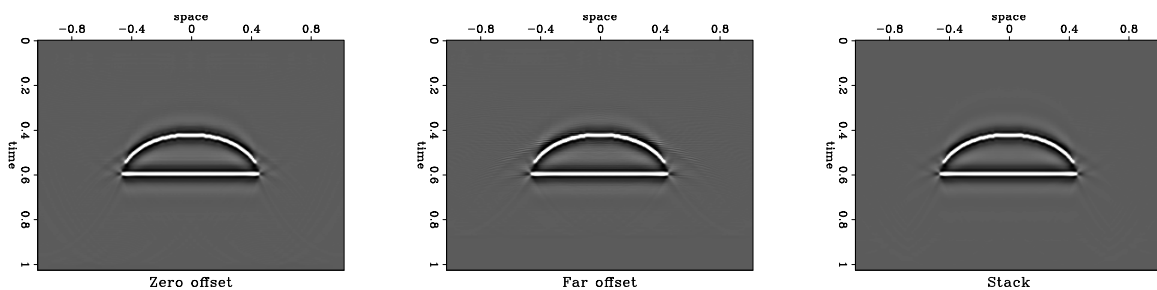
Figure 6: Left: Migrated offset section at zero offset. Center: Migrated offset section at far offset. Right: Stack. angle-offset.dome [ER]
