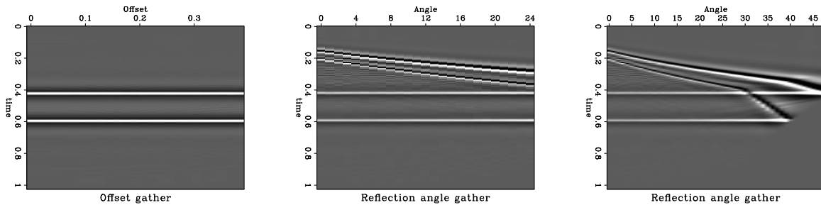
Figure 10: Gathers taken from space location zero in the dome model. Left: Offset domain. Center: Angle domain less than 25^\circ . Right: Angle domain. angle-reflect-ta.dome [ER]
