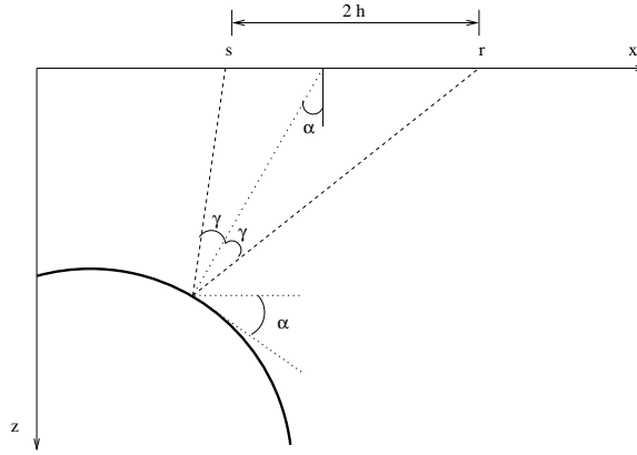
Figure 1: Reflection rays in a constant-velocity medium: a scheme. angle-rays [NR]
