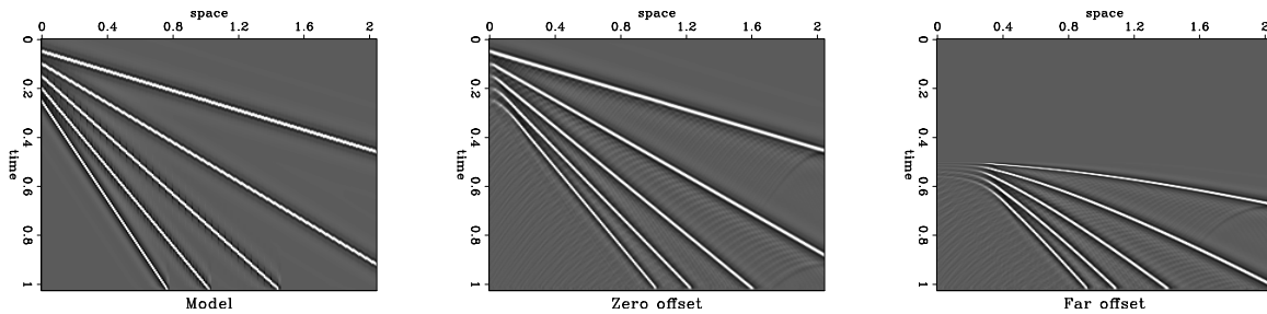
Figure 5: Left: Model. Center: Data at zero offset. Right: Data at far offset. angle-data.lines [ER]
