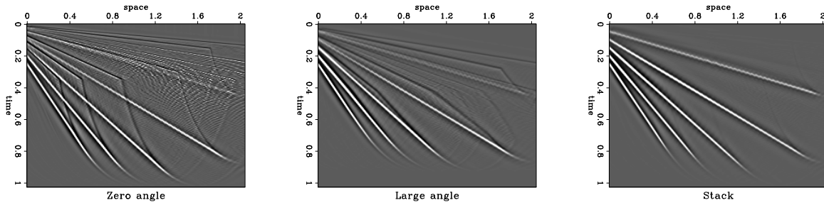
Figure 9: Left: Migrated angle section at zero angle. Center: Migrated angle section at large angle. Right: Stack. angle-angle-ta.lines [ER]
