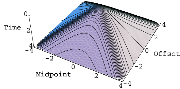
Figure 3: Traveltime pyramid, composed of common-reflection-angle summation curves. angle-cangle [CR]
