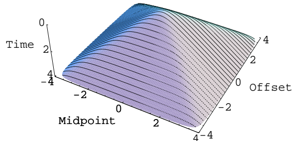
Figure 2: Traveltme pyramid, composed of common-offset summation curves. angle-coffset [CR]
