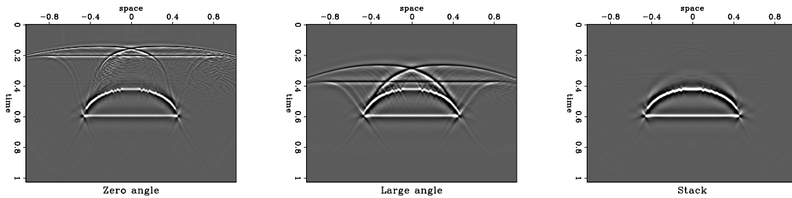
Figure 7: Left: Migrated angle section at small angle. Center: Migrated offset section at large angle. Right: Stack. angle-angle-ta.dome [ER]
