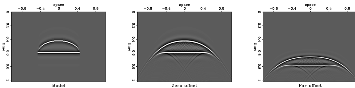
Figure 4: Left: Model. Center: Data at zero offset. Right: Data at far offset. angle-data.dome [ER]
