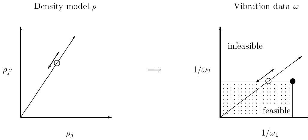
Figure 5: Feasible part of the density space is determined implicitly by the explicit boundaries defined by the frequency data.
