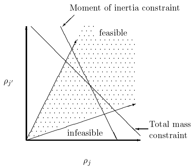
Figure 10: The scale of the density is determined by the total mass and/or the moment of inertia of the Earth.
