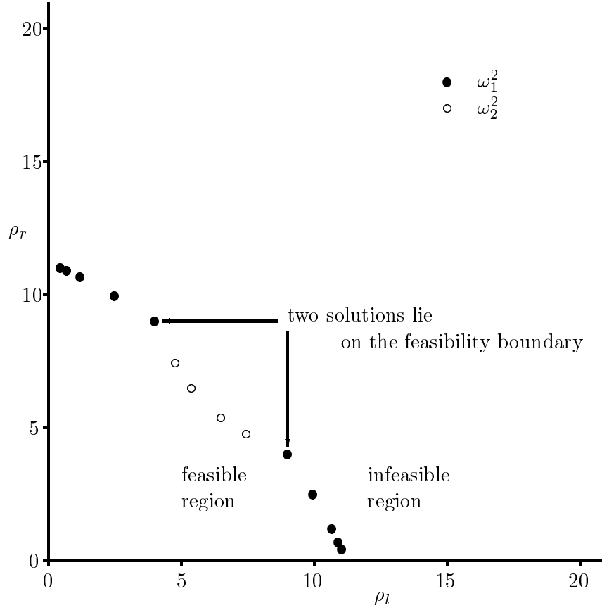
Figure 8: Using the data from Fig. 4, we find the boundary of the feasible region is determined in this problem by the data for \omega_1^2 for large density ratios, and by \omega_2^2 for density ratios closer to unity. These two sets of data cross at the two solutions to the inverse problem, which are seen to be two points in the model plane: (4,9) and (9,4). It is not possible to choose between these two solutions using frequency data alone.
