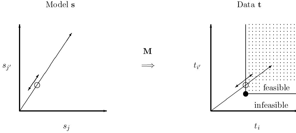
Figure 2: Scaling \mathbf{s} to find feasibility boundary point. Feasibility boundary in data space is explicitly determined by the data. Feasibility boundary in model space is implicitly determined through the traveltime calculation.
