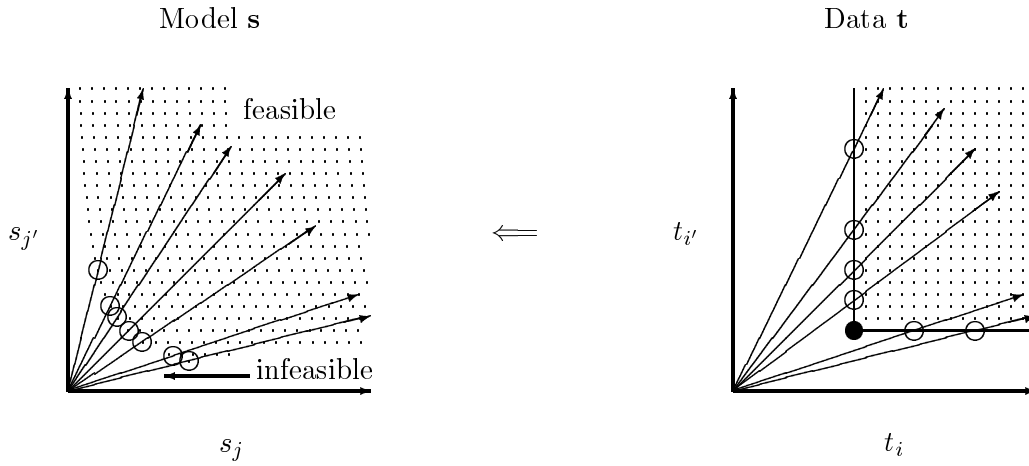
Figure 3: By scaling many slowness vectors \mathbf{s} , the location of the feasibility boundary in the model space can be mapped.
