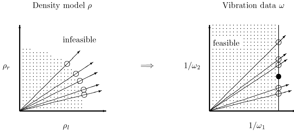
Figure 6: By scaling many density distributions, the location of the feasibility boundary can be mapped.
