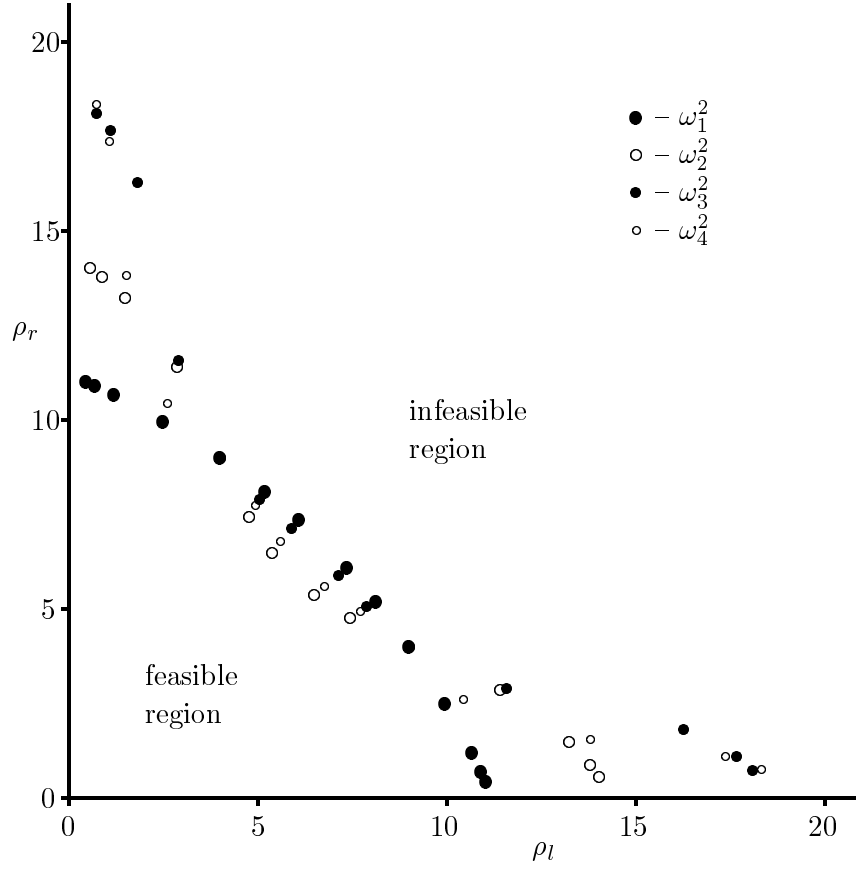
Figure 7: Using the four measurements of eigenfrequencies \omega_1^2, \dots, \omega_4^2 and exact calculations of the eigenfrequencies for various density ratios in TABLE 1, we obtain this plot through scaling of the densities for fixed density ratios. The region near the origin is feasible, while the exterior region is infeasible.
