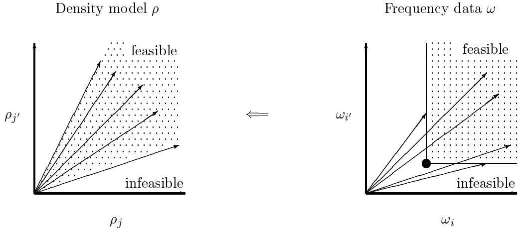
Figure 9: For free oscillations, scaling the density \rho by a positive constant does not change either the trial eigenfunctions or the frequencies, showing that any point along a ray in density space is equally good for satisfying the frequency data. Thus, the feasible region forms a cone in the density space.
