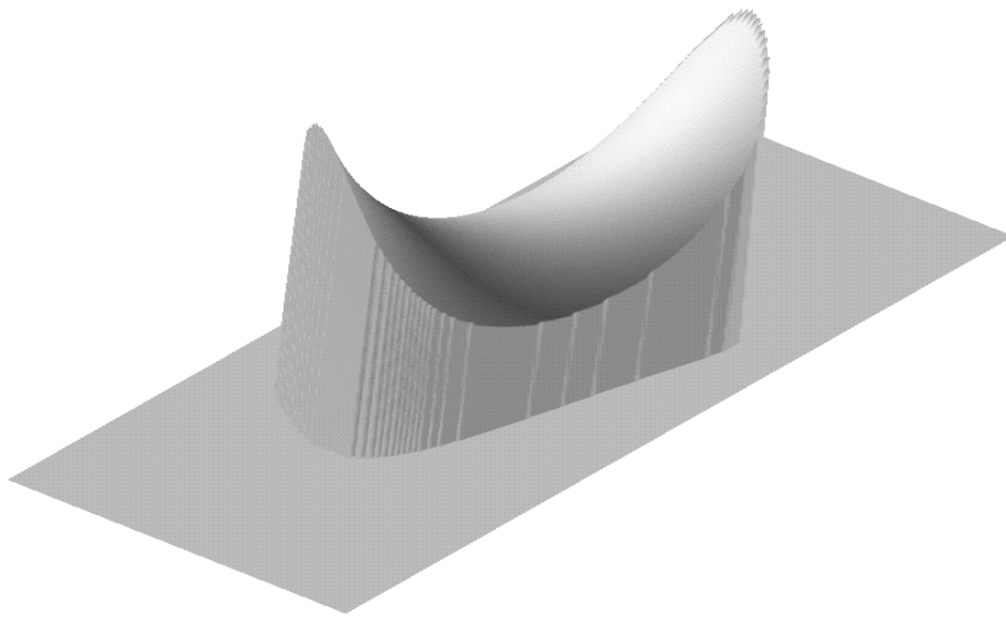
Figure 4: AMO impulse response traveltime in three dimensions (the AVS display). Parameters: |\mathbf{h1}| = 1000 m, |\mathbf{h2}| = 750 m, t_1 = 1 sec, v = 2000 m/s, \varphi = 30^\circ . sergey4-amovs [NR]
