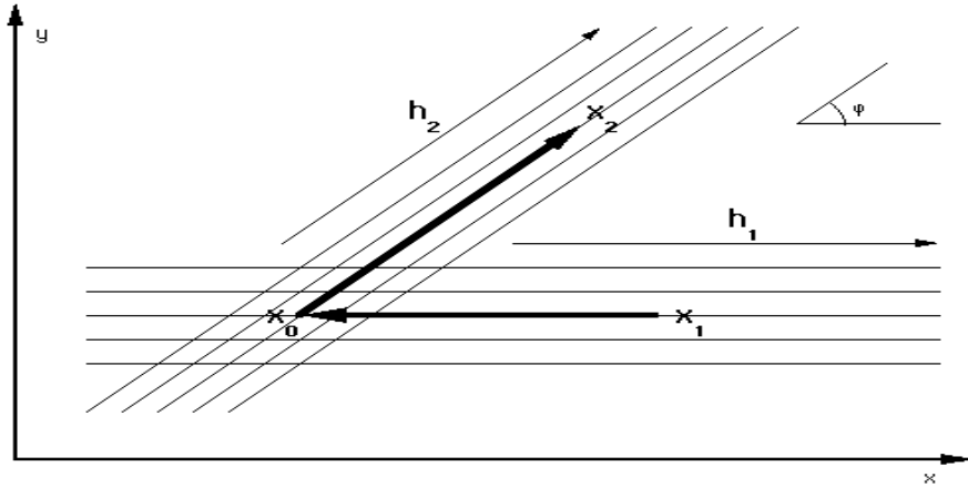
Figure 1: Geometric relationships between input and output midpoint locations in AMO. sergey4-amox12 [NR]
