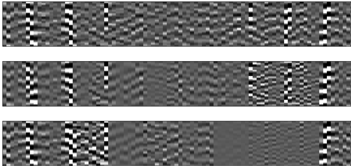
Figure 1.9: Reciprocal traces were extracted from the ten four-component shots and equalized using matching filters designed for each individual trace pair after the energy level in the trace was optimally matched with a limit of five iteration. The top plot shows the data obtained with no source variations; the middle plot shows the data resulting from reciprocal equalization and the bottom plot shows the data with source variations. The equalization finds approximately the right amplitude level, but deviates still a small amount in the frequency character of some events; however it is an improvement compared to the unequalized data. srceq-windowxx [CR]
