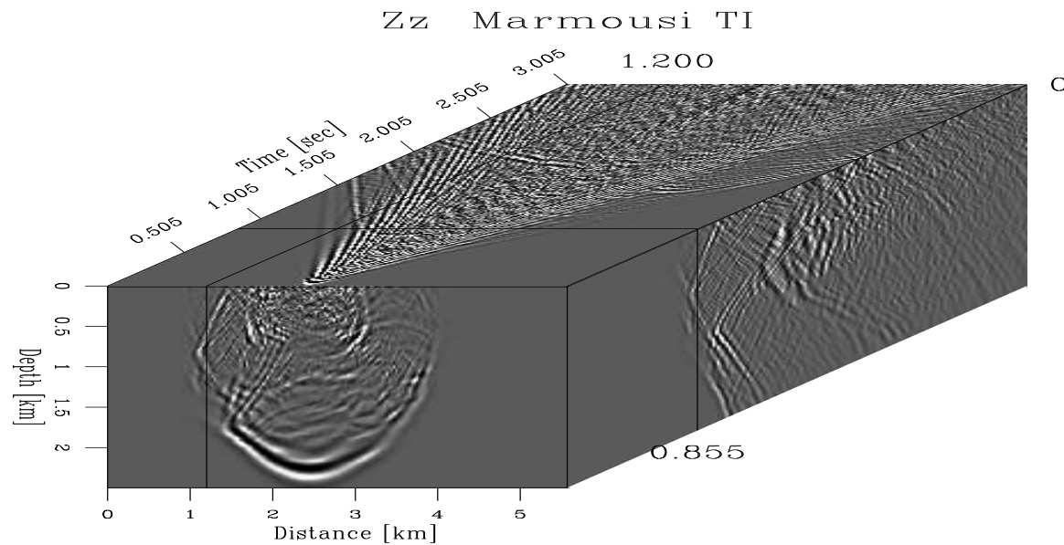
Figure 1.3: Ten shot are modeled in a Marmousi model that has been extended to a transverse isotropy. The Zz component of the recording is shown in this picture.
