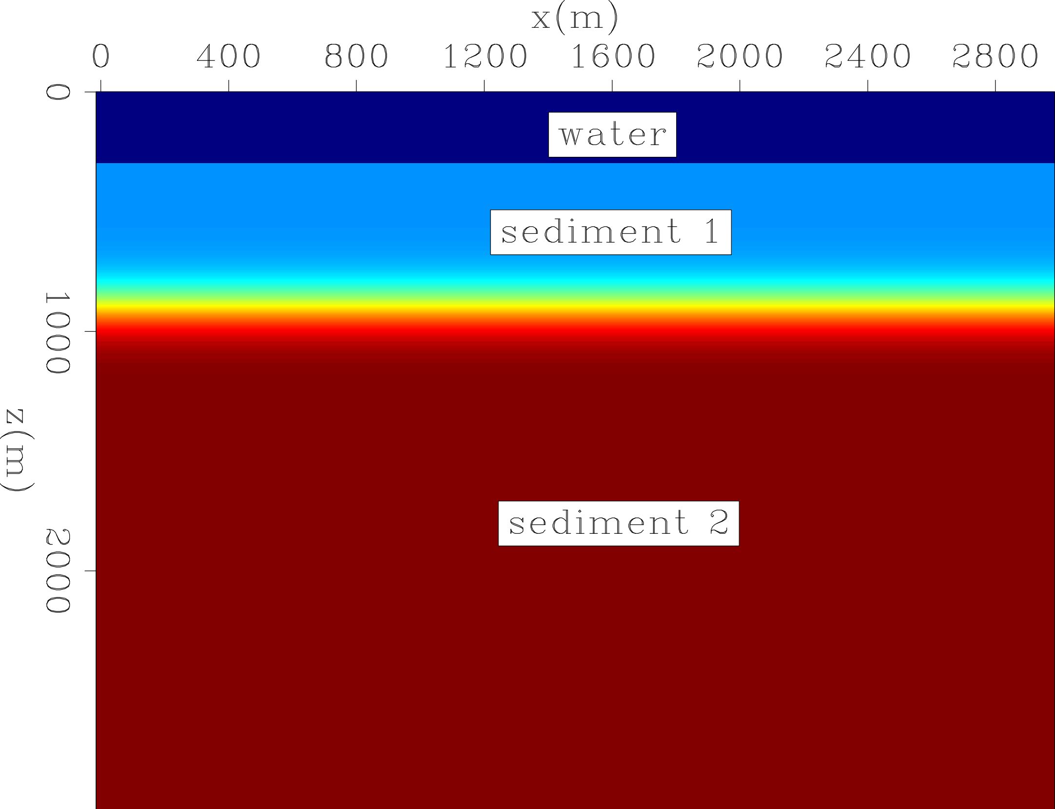
1D V_p , V_s , density layers
