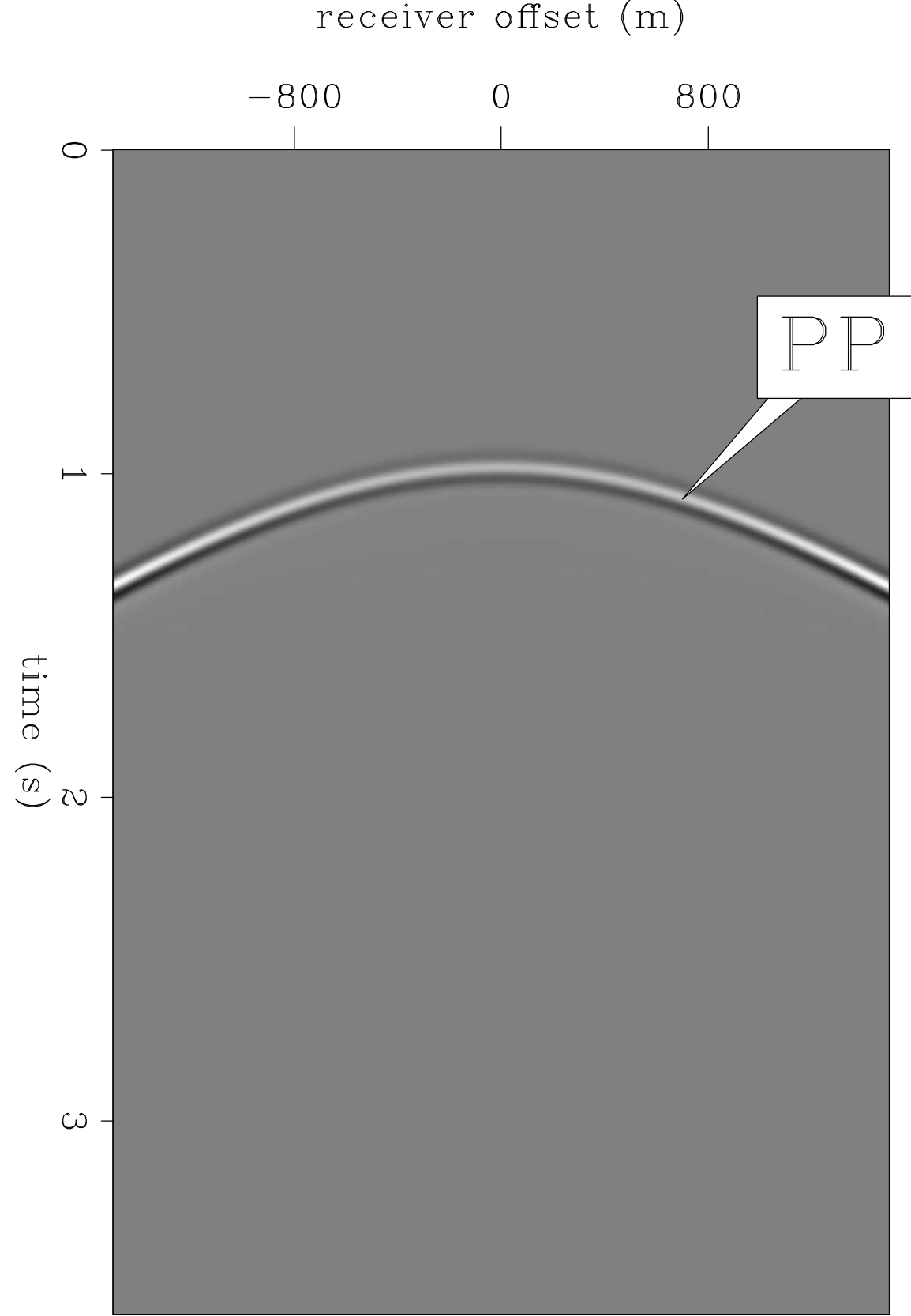
PZ sum of acoustic data: upgoing
