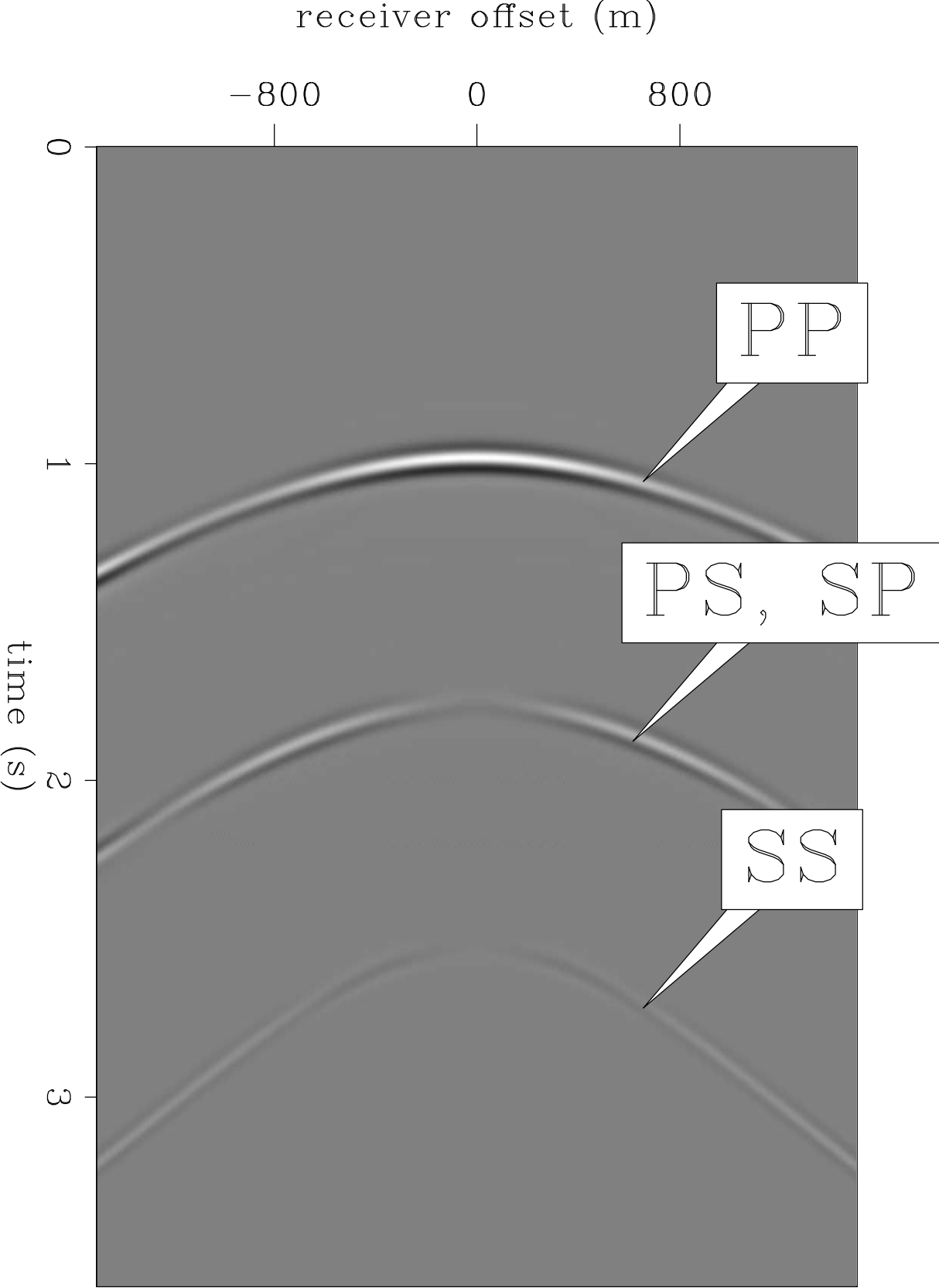
PZ sum of elastic data: upgoing
