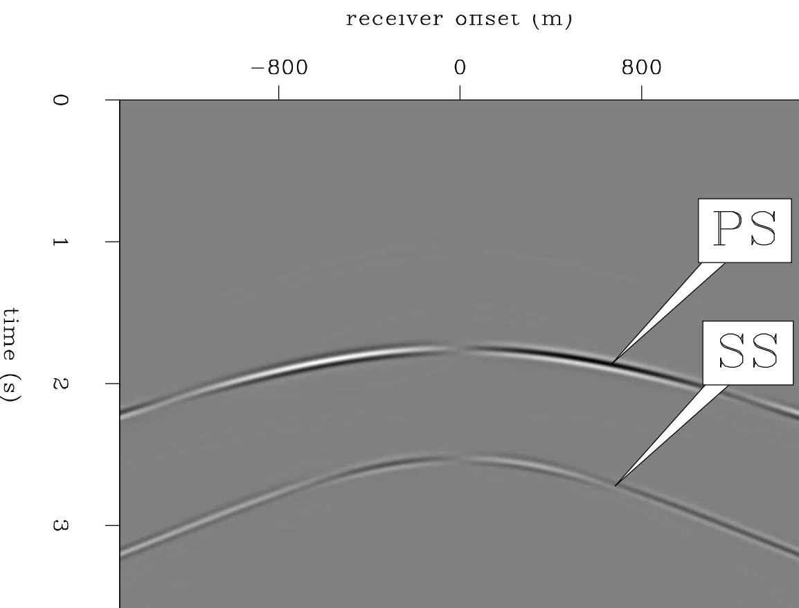
Shear wave
