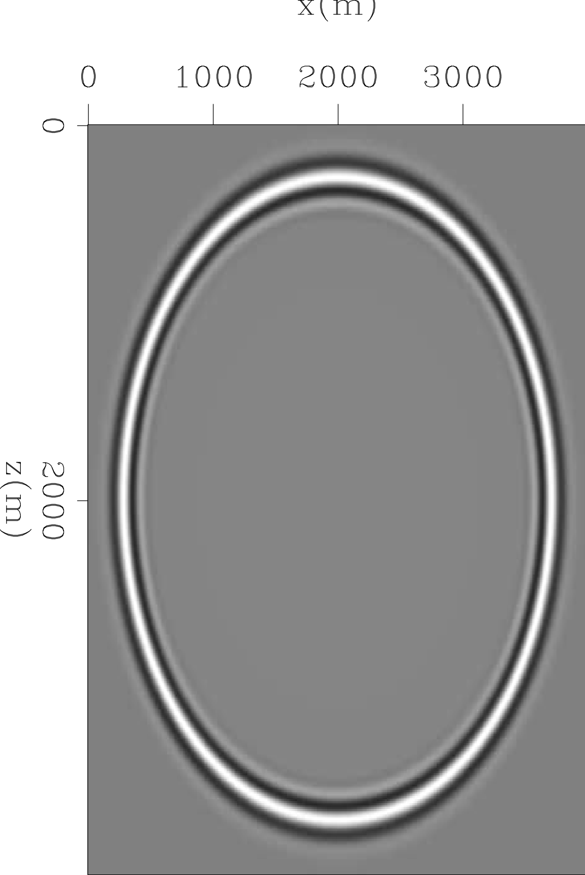
implicit helical FD with dt=0.005
