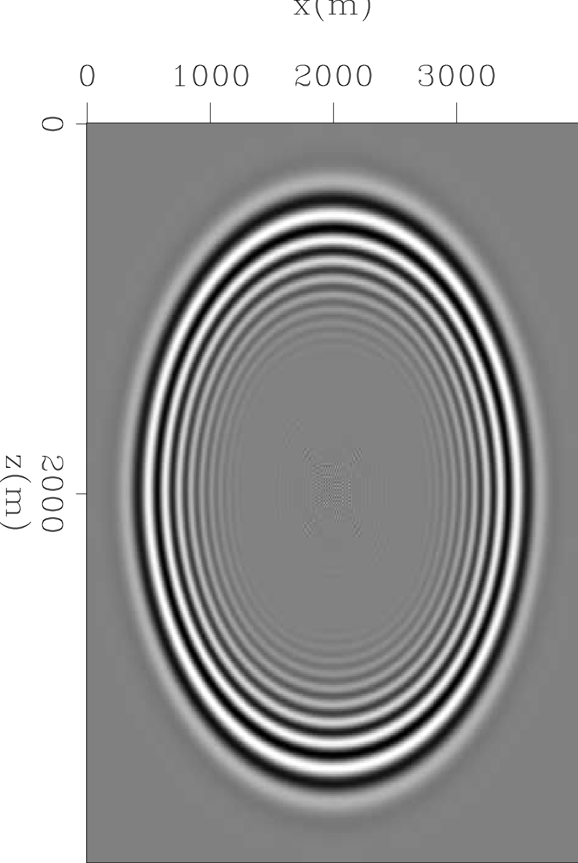
implicit helical FD with dt=0.02 \epsilon=0.04
