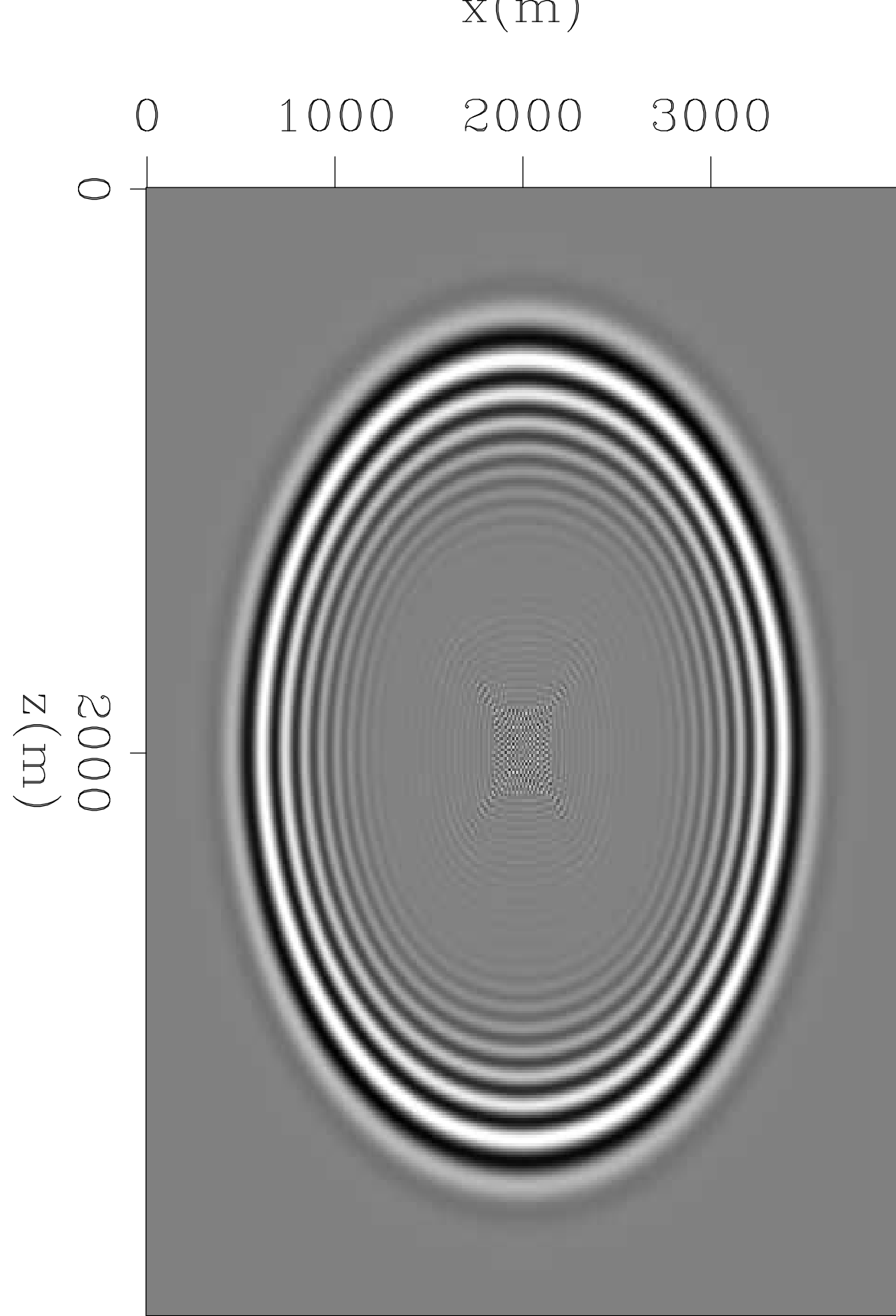
implicit helical FD with dt=0.02 \epsilon=0.08
