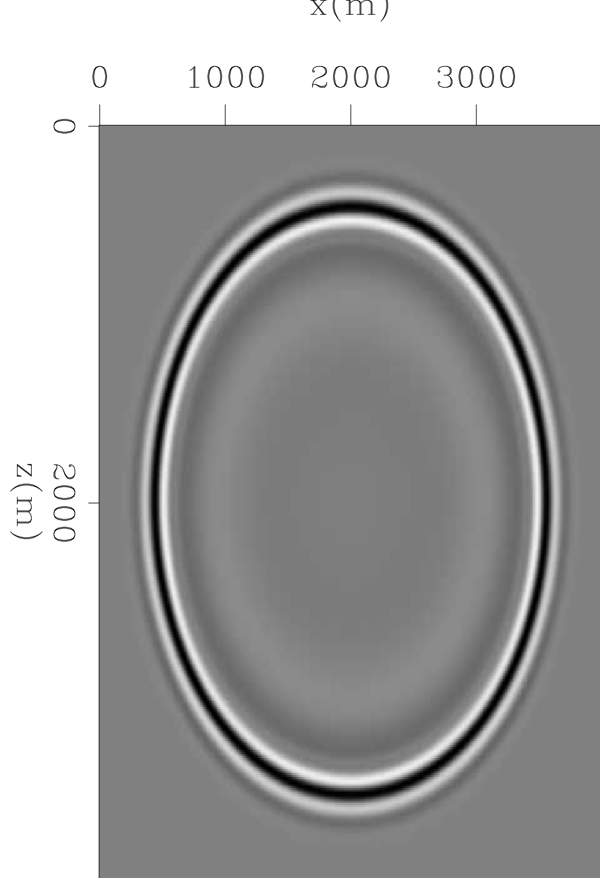
implicit helical FD with dt=0.01 \epsilon=0.02
