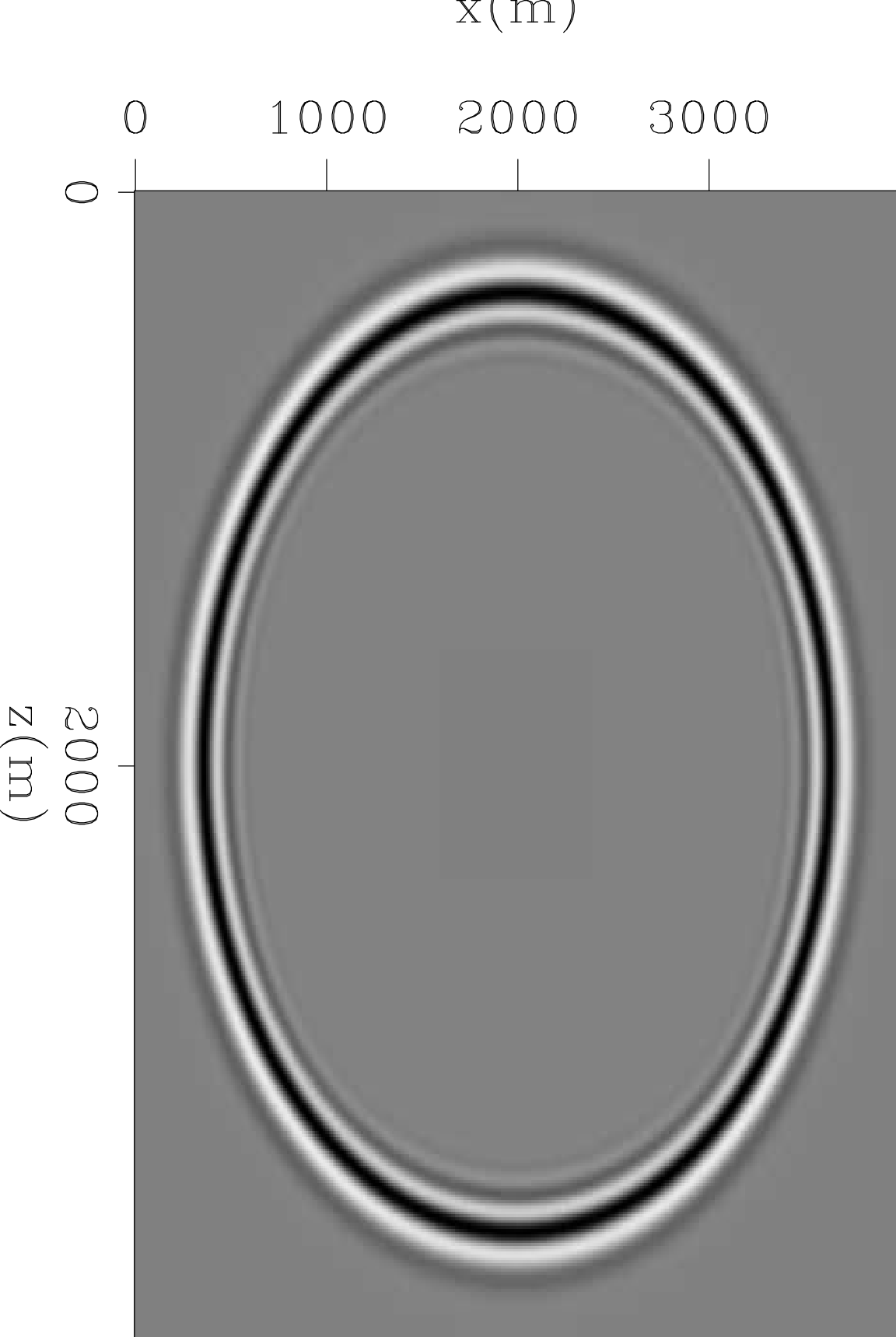
implicit helical FD with dt=0.01 \epsilon=0.005
