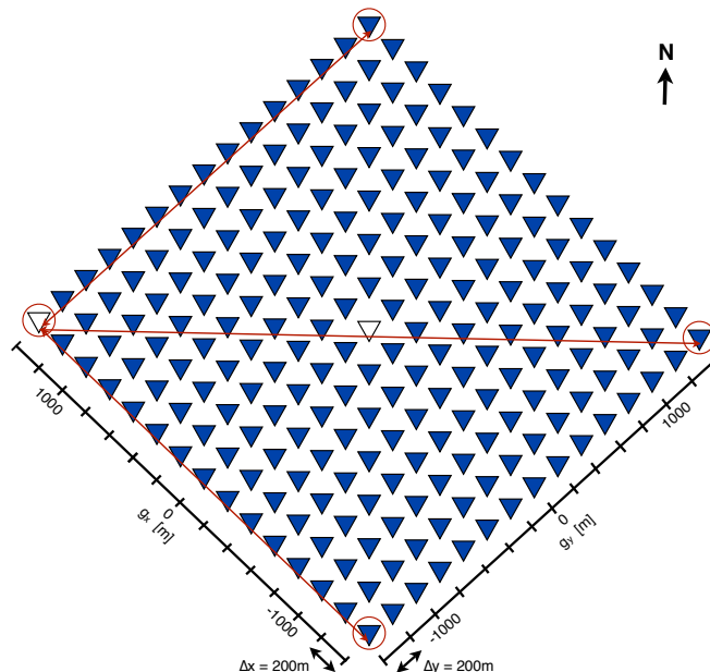
Figure 1: Geometry of the Aramco passive experiment; 225 stations (denoted by triangles) placed in a 15 by 15 grid. The geographic North is indicated by N . Open triangles denote stations turned into virtual sources for Figures 7 and 8. Lines denote receiver lines for sections shown in Figure 7. [NR]
