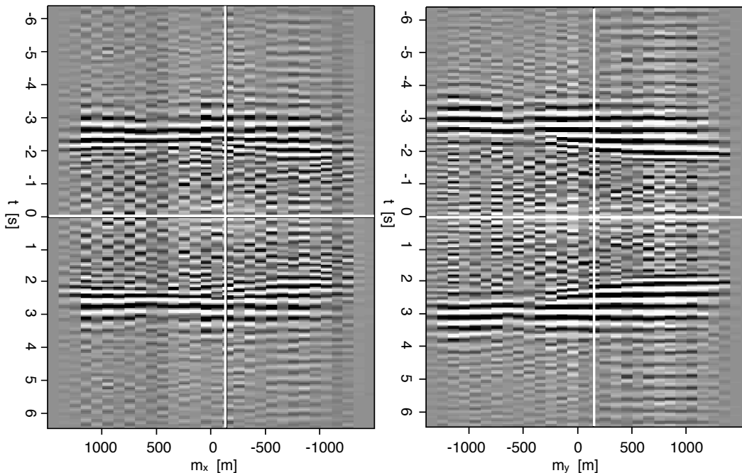
Figure 9: Two slices through a cube of retrieved Green's functions as a function of midpoints, for fixed full radial offset of 2h_r = 1640 m. Left: m_y = 100 m, right: m_x = 100 m. [CR]
