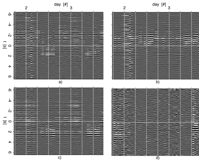
Figure 8: Green's functions for a virtual shot gather of a source positioned at (s_x, s_y) = (0, 0) m and stations at; a) (g_x, g_y) = (1400, -1400) m; b) (g_x, g_y) = (1400, 1400) m; c) (g_x, g_y) = (-1400, -1400) m; d) (g_x, g_y) = (-1400, 1400) m. [CR]
