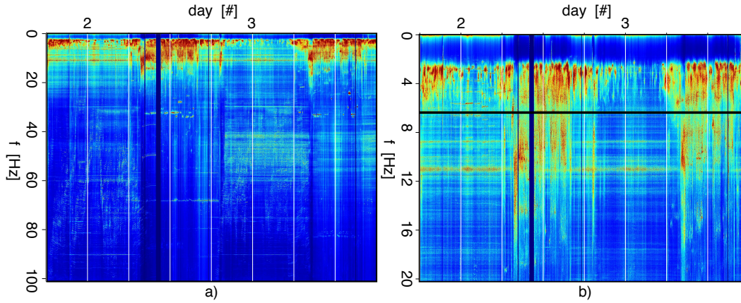
Figure 2: Frequency-domain amplitude spectrum averaged over the array as a function of time for 48 hours. White grid lines denote 6 hour blocks. a) Frequency-domain amplitude spectrum between 0 Hz and 100 Hz; b) frequency-domain amplitude spectrum between 0 Hz and 20 Hz; the black line denotes the frequency of the low-pass filter applied before interferometry. [CR]
