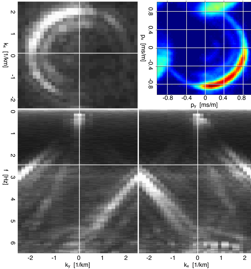
Figure 4: Cross-sections through frequency-wavenumber spectra cube and averaged over the data recorded between 20:00 and 21:00 on day 1. The top right panel contains a beam-forming experiment for the frequency band of 1 Hz to 3.5 Hz. [CR]
