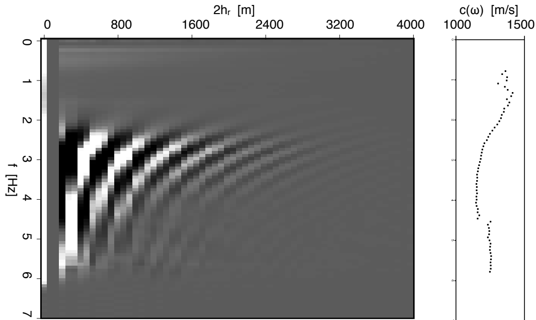
Figure 10: Left; real part of the retrieved Green’s functions in the frequency-domain, shown as function of full radial offset, averaged over all midpoints. Right; estimated dispersion curve for the retrieved Green’s functions shown in the left panel. [CR]
