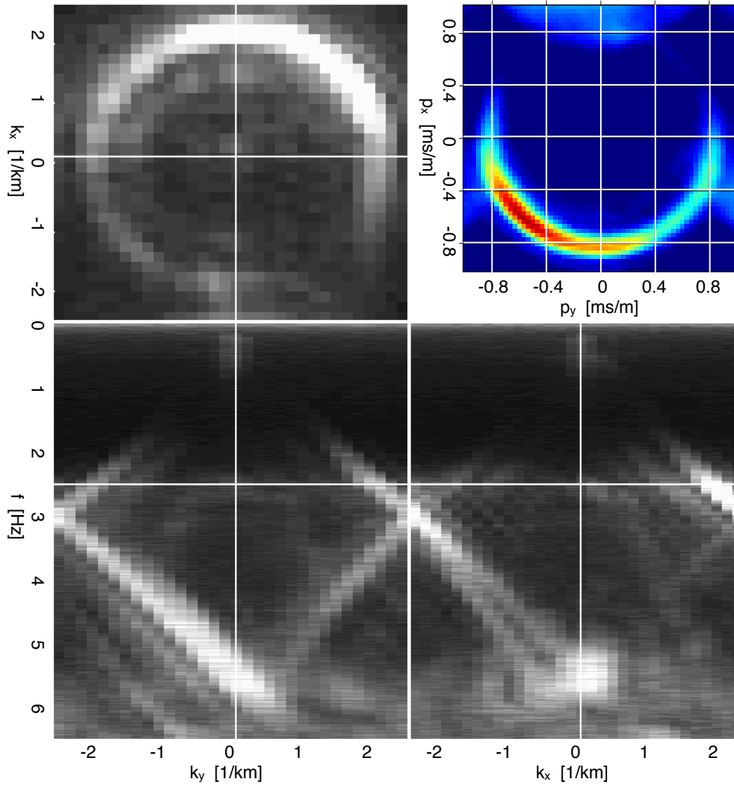
Figure 5: Cross-sections through frequency-wavenumber spectra cube and averaged over the data recorded between 11:00 and 12:00 on day 2. The top right panel contains a beam-forming experiment for the frequency band of 1 Hz to 3.5 Hz. [CR]
