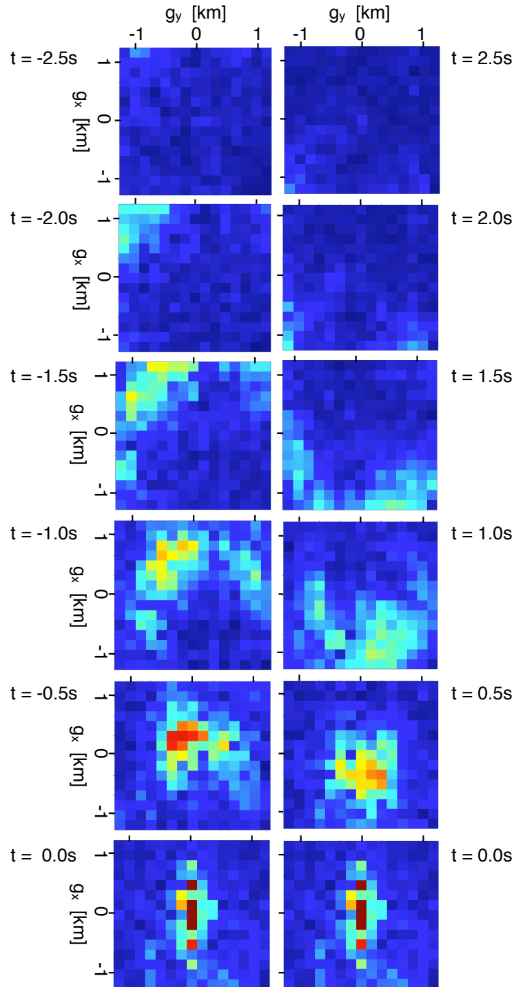
Figure 6: Snap shots of a movie of the acausal (left) and causal (right) parts of retrieved Green's functions for a virtual source at (s_x, s_y) = (0, 0) m. [NR]
