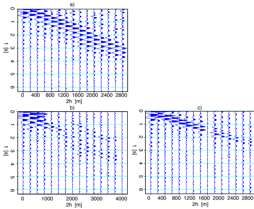
Figure 7: Causal retrieved Green's functions plotted as a function of full offsets ( 2h ) for a source positioned at (s_x, s_y) = (1400, -1400) m. a) A g_x -slice at g_y = -1400 m; b) a g_y -slice at g_x = -1400 m and; c) a diagonal slice. [CR]
