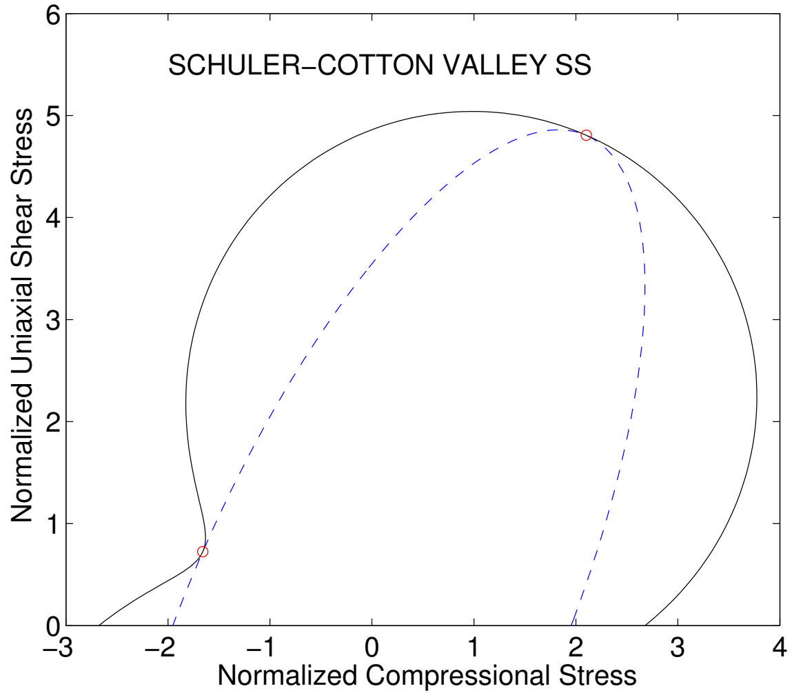
Figure 6: Same as Figure 2 for Schuler-Cotton Valley Sandstone using the parameters from the TABLE. jim2-SCV2Stress [NR]
