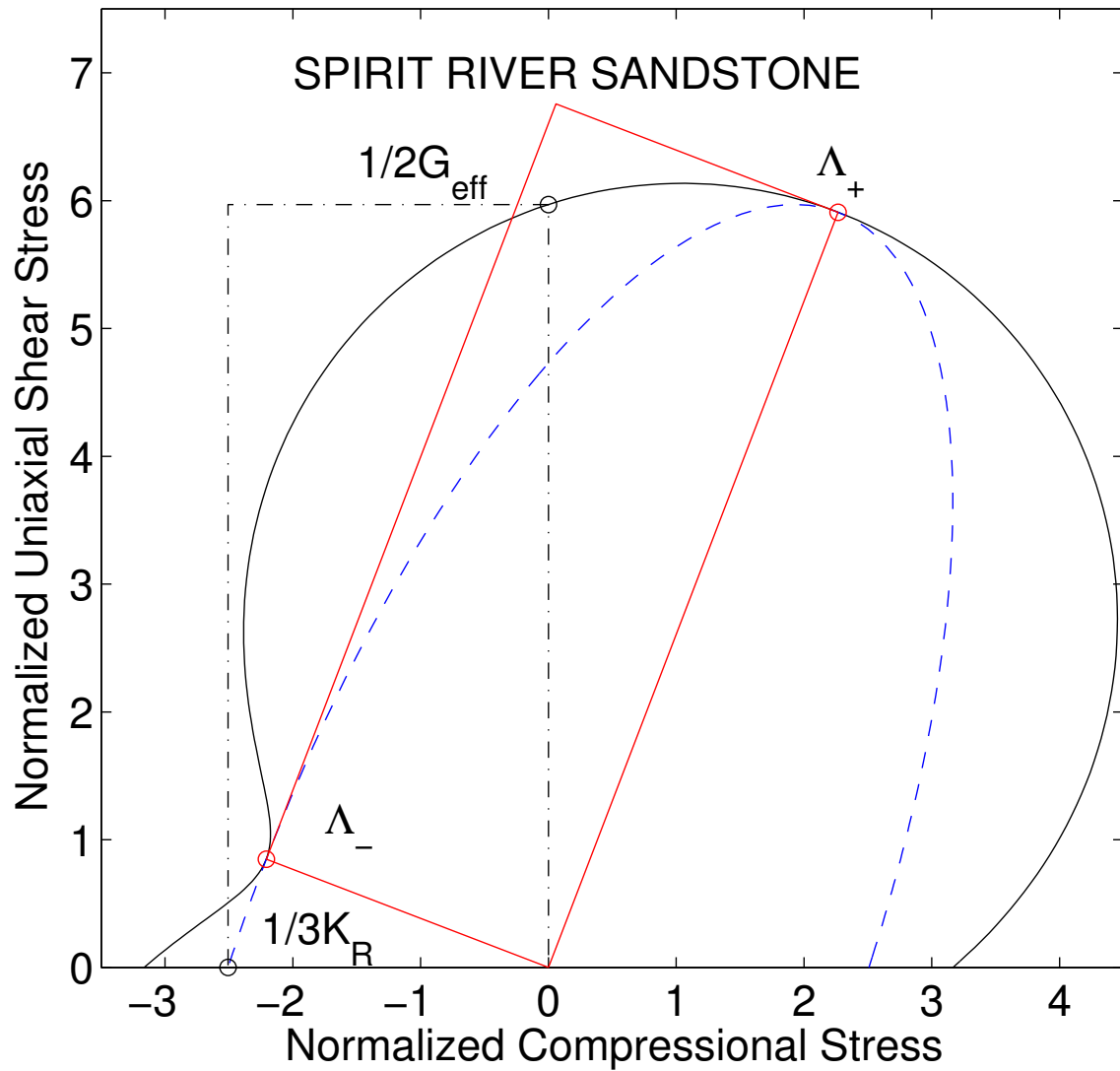
Figure 8: Same as Figure 2 for Spirit River Sandstone using the parameters from the TABLE.
