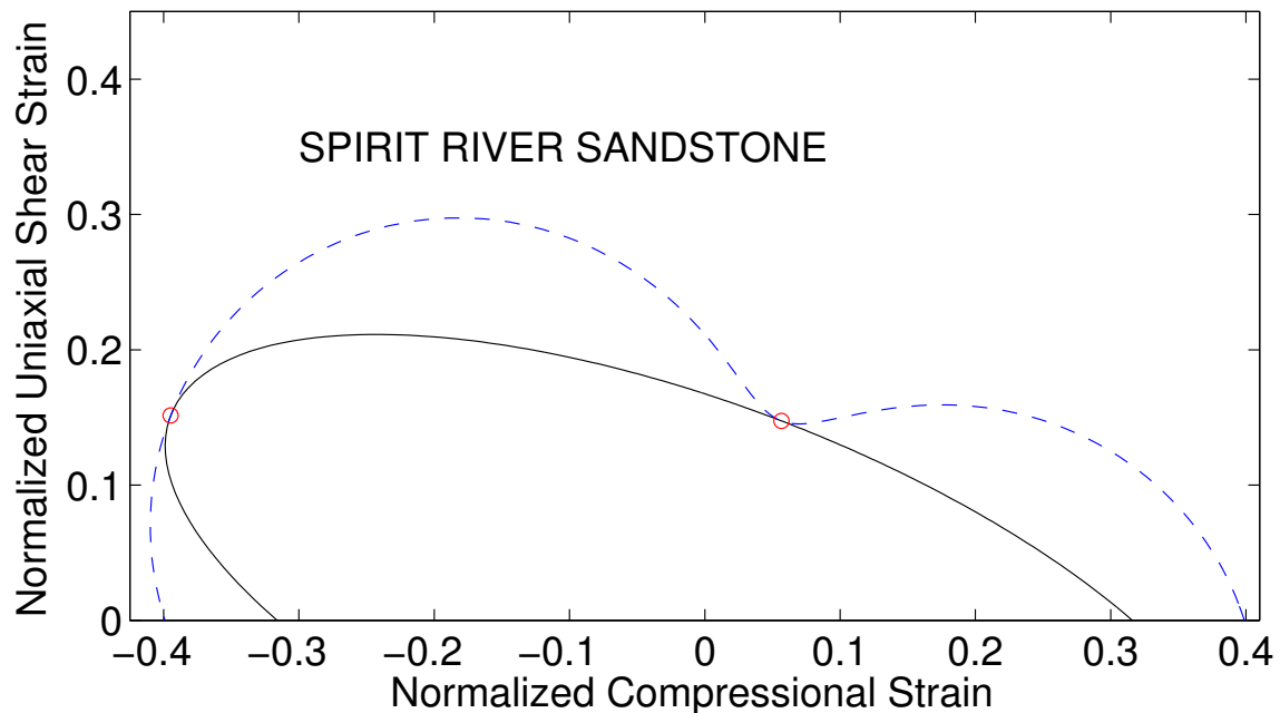
Figure 7: Same as Figure 1 for Spirit River Sandstone using the parameters from the TABLE. jim2-SRSStrain [NR]
