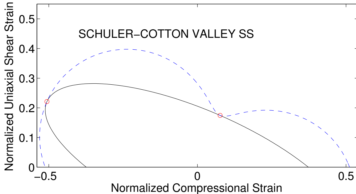
Figure 5: Same as Figure 1 for Schuler-Cotton Valley Sandstone using the parameters from the TABLE. jim2-SCV2Strain [NR]
