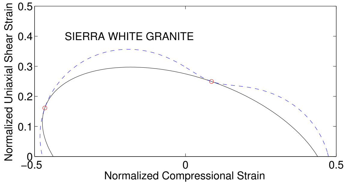
Figure 3: Same as Figure 1 for Sierra White Granite using the parameters from the TABLE. jim2-SW2Strain [NR]
