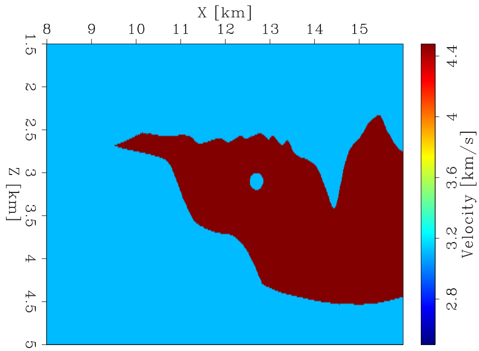
Figure 4: True model [ER]
