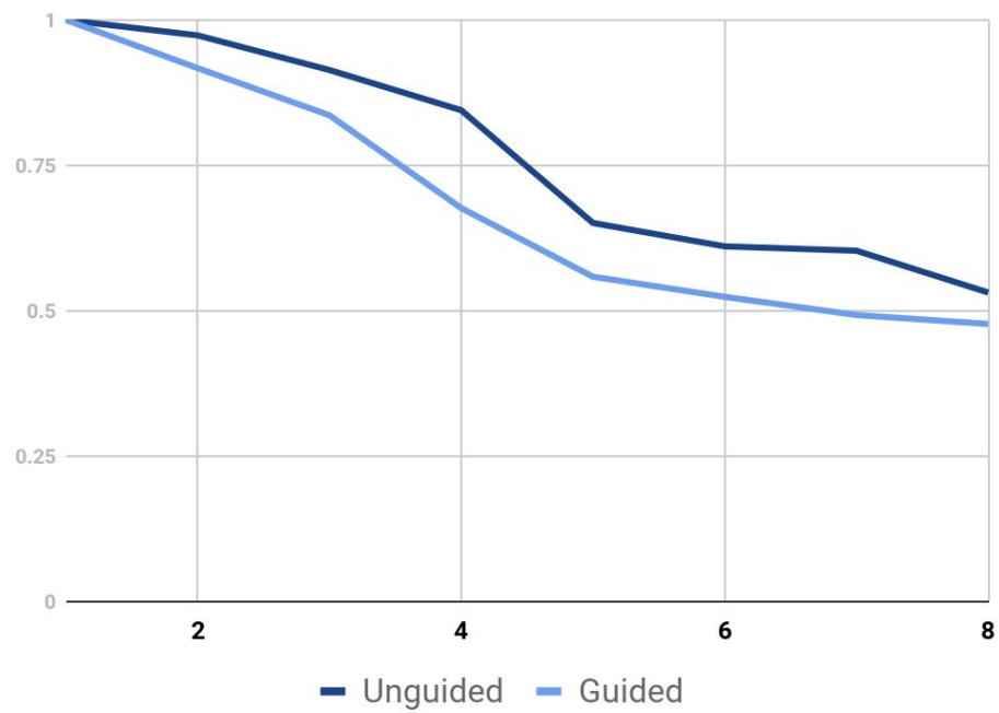
Figure 8: Model residual norm. [CR]
