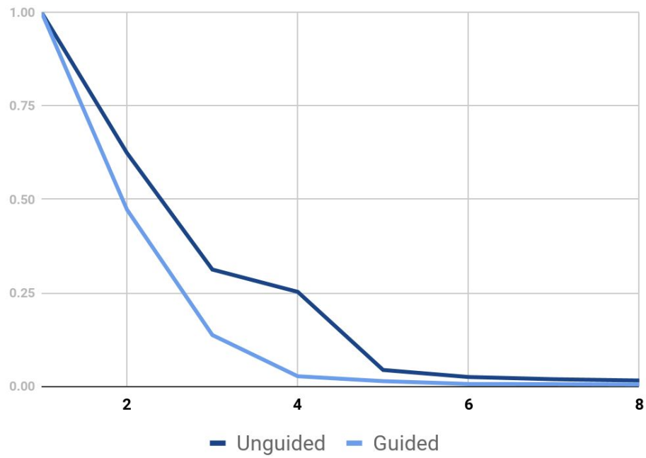
Figure 7: Objective function value (data residual norm). [CR]
