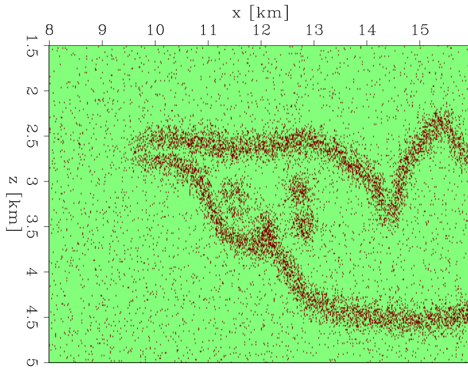
Figure 3: RBF center locations. [ER]
