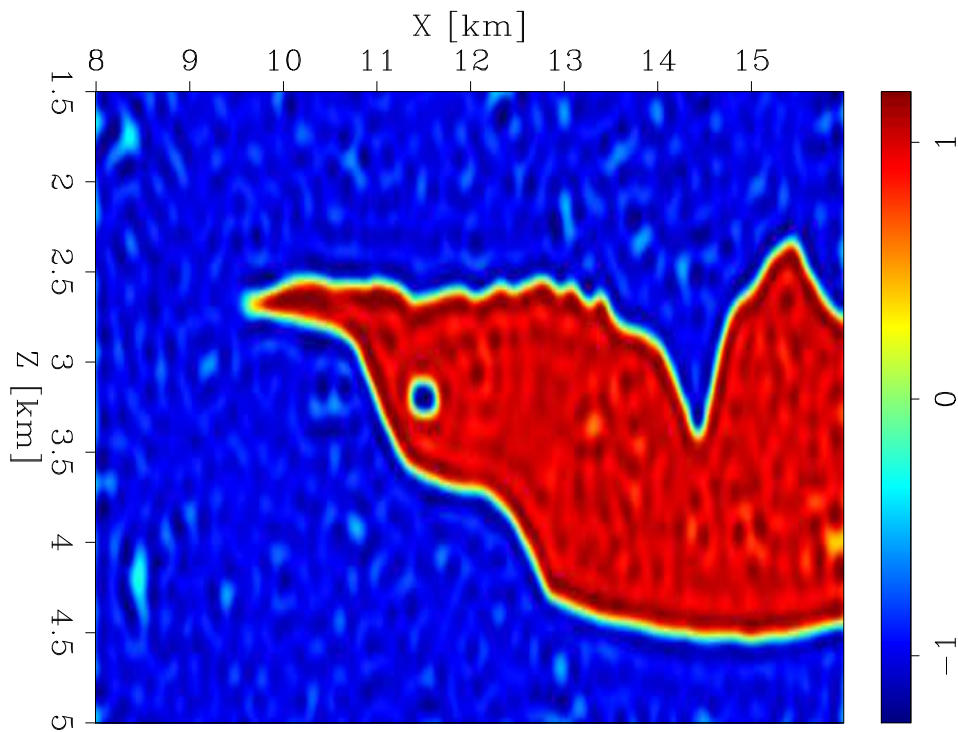
Figure 2: Initial implicit surface (unguided). [ER]
