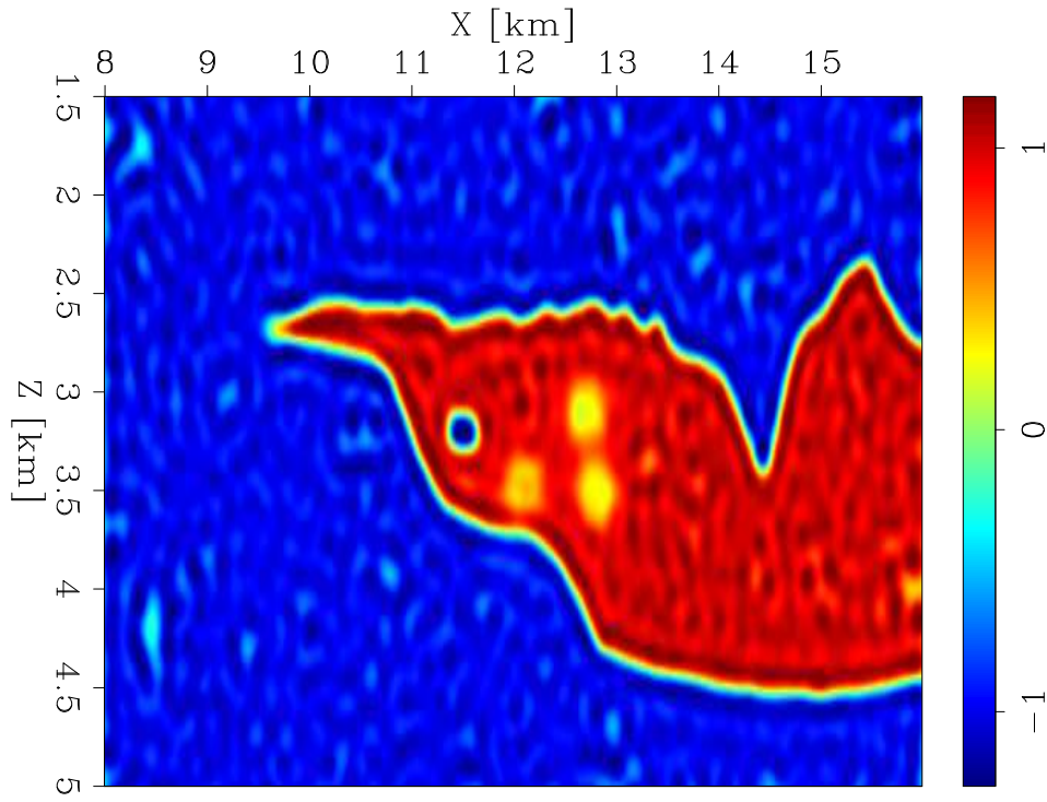
Figure 1: Initial implicit surface (guided). [ER]
