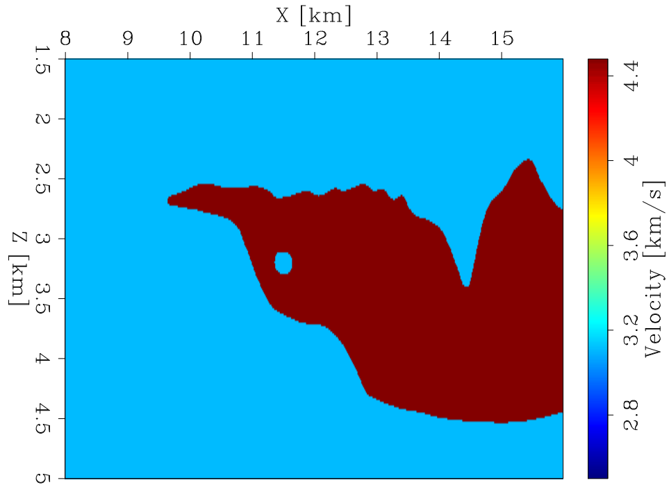
Figure 5: Initial model (guided). [ER]
