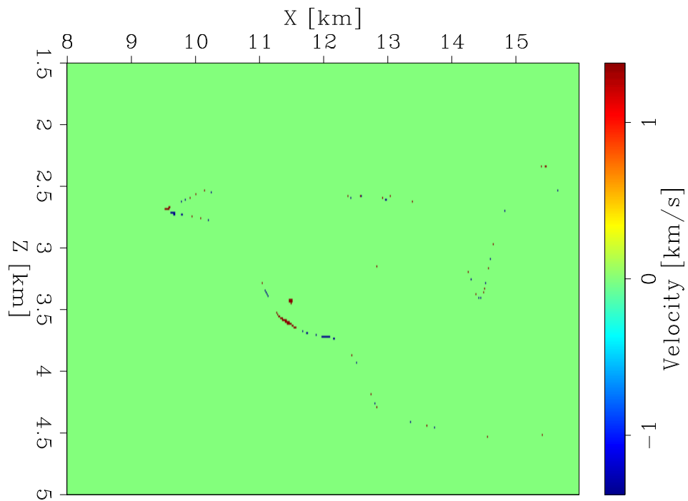
Figure 6: m_{\text{true}} - m_{\text{init}} (guided, at it=8) [CR]
