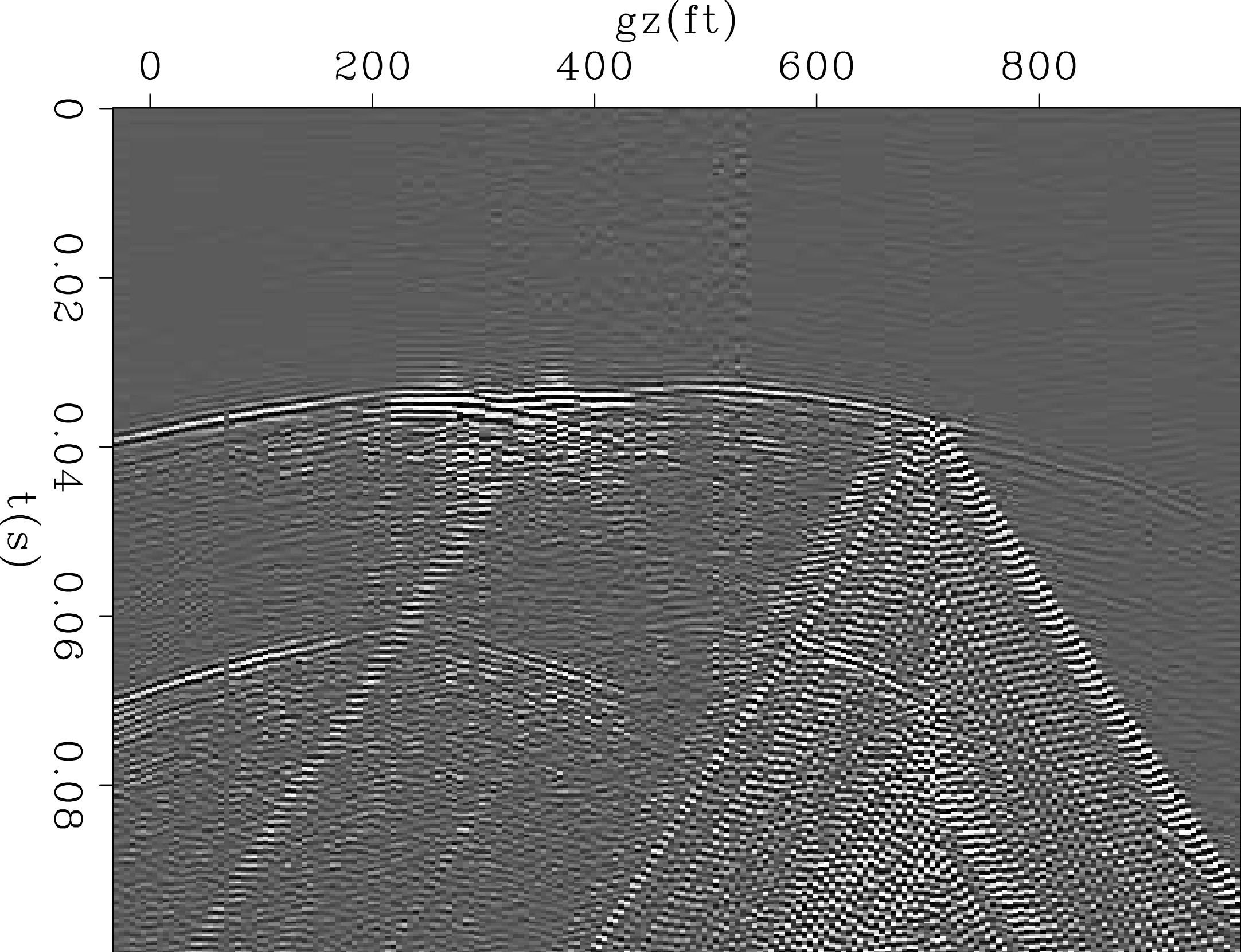
raw shot gather
