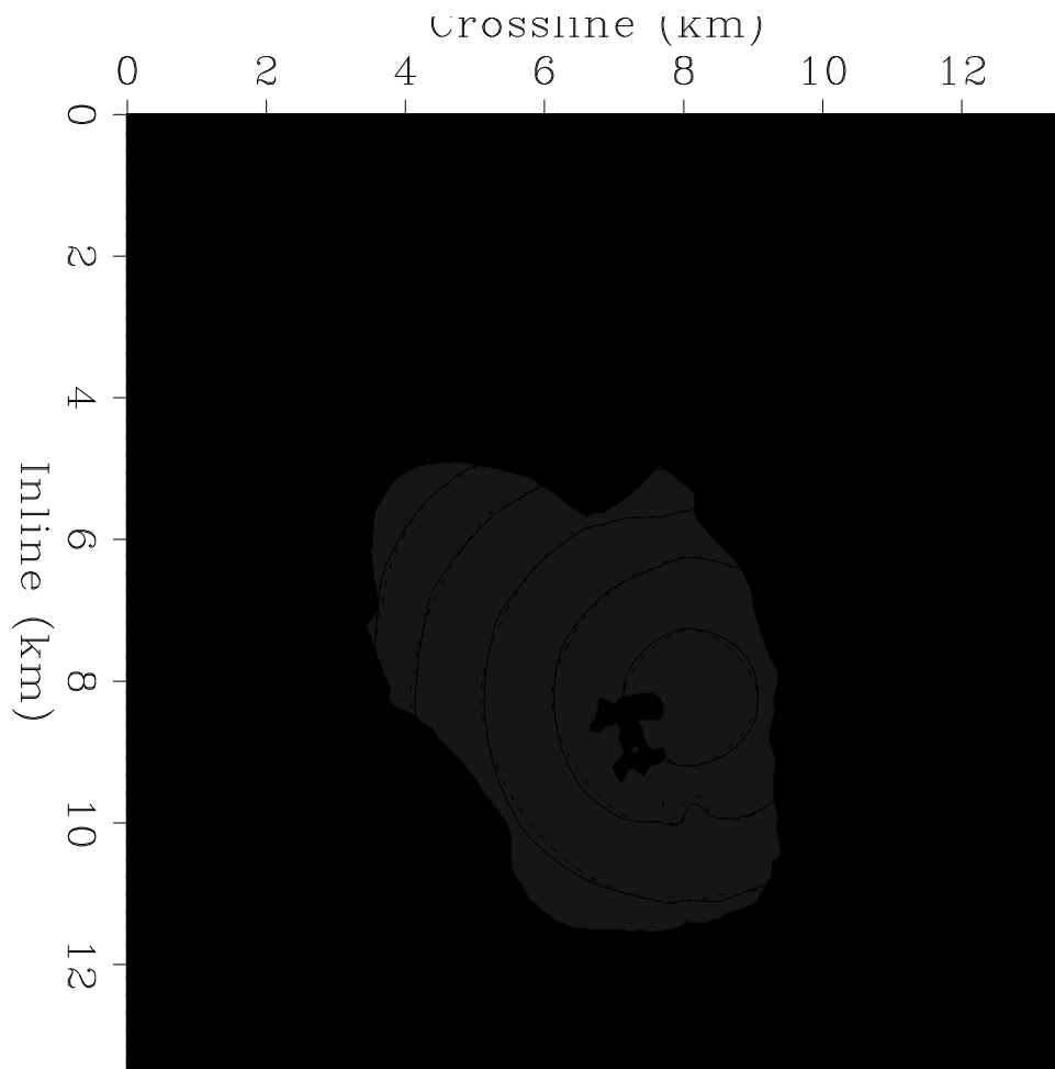
Figure 9: Traveltime slice of 3-D SEG/EAGE salt dome model for a constant z = 1560m . The solid line represents tetragonal result and the dash line for the Cartesian result. For most part, the Cartesian result tends to over-estimate the traveltime than the tetragonal result.
