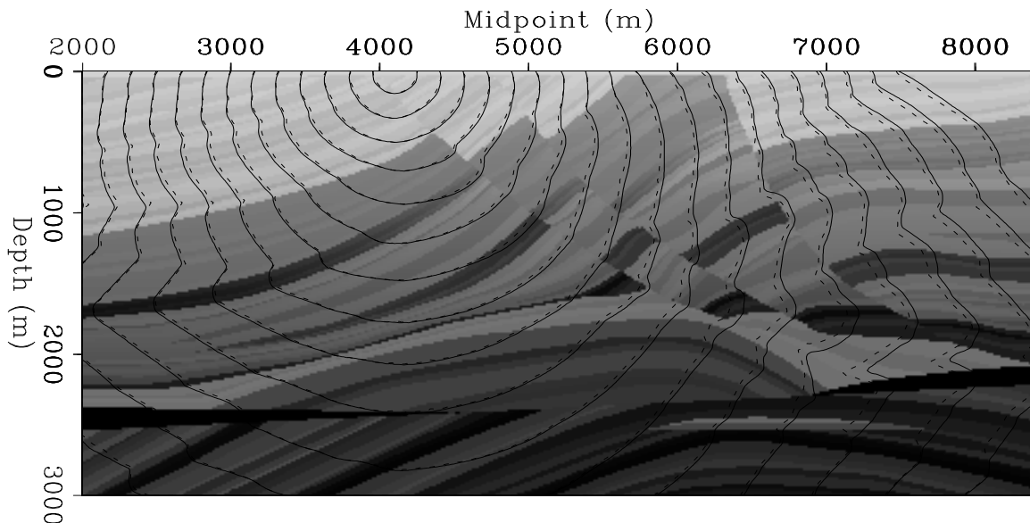
Figure 8: Traveltime slice of 2-D Marmousi model. The solid line stands for the trigonal result and the dash line for the Cartesian result. The Cartesian implementation tends to over-estimate the traveltime. fmtetra-marm-comp [ER]
