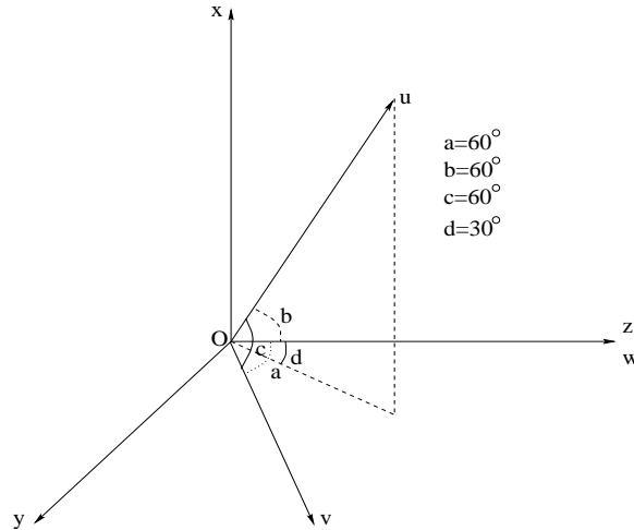
Figure 1: The tetragonal coordinates used in this paper. It reduces to the trigonal coordinates by omitting axis u . fmtetra-coord [NR]
