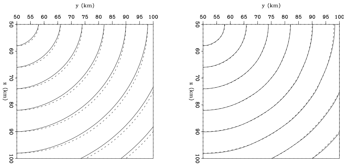
Figure 7: Left: Cartesian. Right: tetragonal. Traveltime slice from a 3-D constant velocity model. The source is located at the upper-left corner and the spatial sampling interval is 1km in all the three directions. The dash line represents the analytical solution. The solid line on the left panel stands for the Cartesian implementation and the solid line on the right for the tetragonal case. The Cartesian result has obvious errors in the diagonal direction. The tetragonal result matches the analytical result accurately. fmtetra-const3D-comp [CR]
