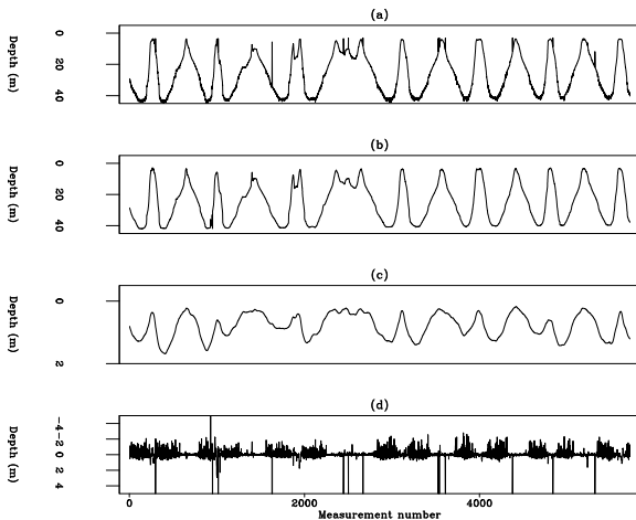
Figure 7.23: (a) Track 14 (input data) in Figure 7.18. (b) Modeled data, \mathbf{BH}^{-1}\mathbf{p} . (c) Estimated drift. (d) Data-space residual. noiz-antoine6 [ER]
