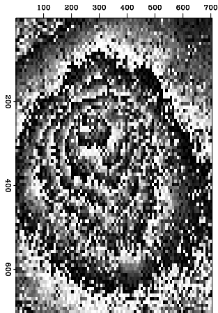
decimated
