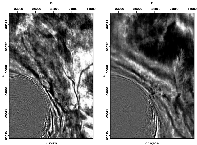
Figure 11.2: Some time slices show a salt dome, some river channels, a dendritic drainage canyon, and a fault. Press button for interactive “Rickmovie”.
