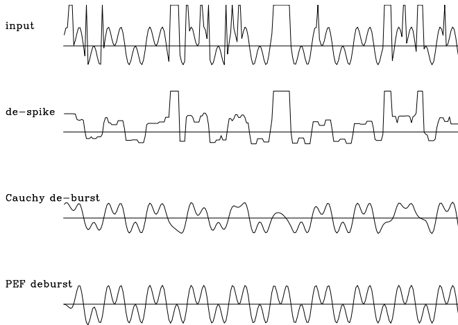
Figure 7.6: Top is synthetic data with noise spikes and bursts. (Some bursts are fifty times larger than shown.) Next is after running medians. Next is Laplacian filter Cauchy deburst processing. Last is PEF-deburst processing. noiz-pefdeburst90 [ER]
