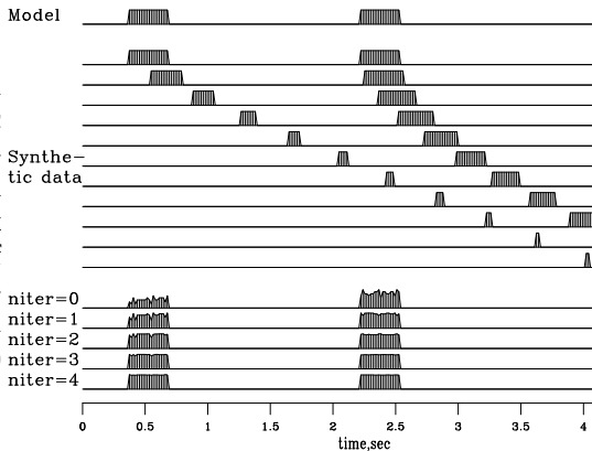
Figure 2.1: Top is a model trace \mathbf{m} . Next are the synthetic data traces, \mathbf{d} = \mathbf{M}\mathbf{m} . Then, labeled \text{niter}=0 is the stack , a result of processing by adjoint modeling. Increasing values of \text{niter} show \mathbf{x} as a function of iteration count in the fitting goal \mathbf{d} \approx \mathbf{M}\mathbf{m} . (Carlos Cunha-Filho)
