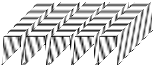
Figure 9.3: A plane of identical values passed through the idempotent patching reconstruction operator. Results are shown for the same parameters as Figure 9.2. pch-idempatch90 [ER]
