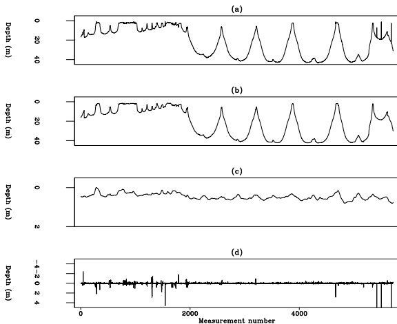
Figure 7.22: (a) Track 17 (input data) in Figure 7.18. (b) The estimated noise-free data \mathbf{BH}^{-1}\mathbf{p} . (c) Estimated drift \mathbf{Lq} . (d) Data residual. noiz-antoine5 [ER,M]
