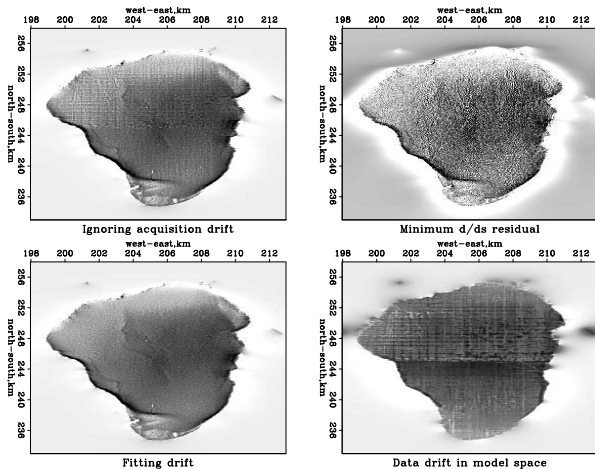
Figure 7.21: Top left: Estimated \mathbf{p} without attenuation of the tracks, i.e., equation (7.23). Top right: Estimated \mathbf{p} with the derivative along the tracks, i.e., equation (7.25). Bottom left: Estimated \mathbf{p} without tracks, i.e., equation (7.26). Bottom right: recorder drift in model space \mathbf{B}^T \mathbf{L} \mathbf{q} . noiz-antoine4 [ER,M]
