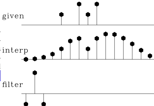
Figure 3.4: Top is the same input data as in Figure 3.3. Middle is interpolated. Bottom shows the filter (-1, 2, -1) . The missing data seems to be interpolated by parabolas.
