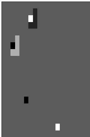
((\text{input}/\text{filter})/\text{filter}')\text{filter}'\text{filter}
