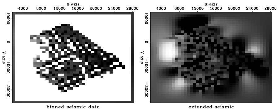
Figure 3.9: Seismic binned (left) and extended (right) by minimizing energy in \nabla^2 \mathbf{s} . iin-misseis90 [ER]
