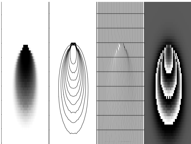
Figure 2.6: Synthetic mountain with hidden backside. For your estimation enjoyment. lsq-synmod90 [ER,M]
