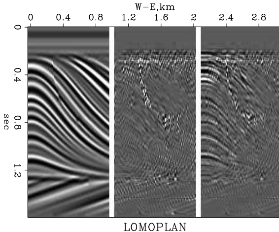
Figure 10.8: Left is a vertical slice through the 3-D “qdome” model. Center is the in-line component of the LOMOPLAN. Right is the cross-line component of the LOMOPLAN. lmn-qdomesico90 [CR]
