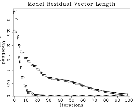
Figure 5.7: Convergence of the iterative optimization, measured in terms of the model residual. The “p” points stand for preconditioning; the “r” points, regularization. prc-schwab1 [ER]
