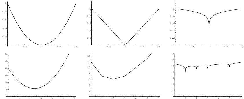
Figure 7.1: Mean, median, and mode. The coordinate is m . Top is the L_2 , L_1 , and L_{1/10} \approx L_0 measures of m-1 . Bottom is the same measures of the data set (1, 1, 2, 3, 5) . (Made with Mathematica.) noiz-norms [CR]
