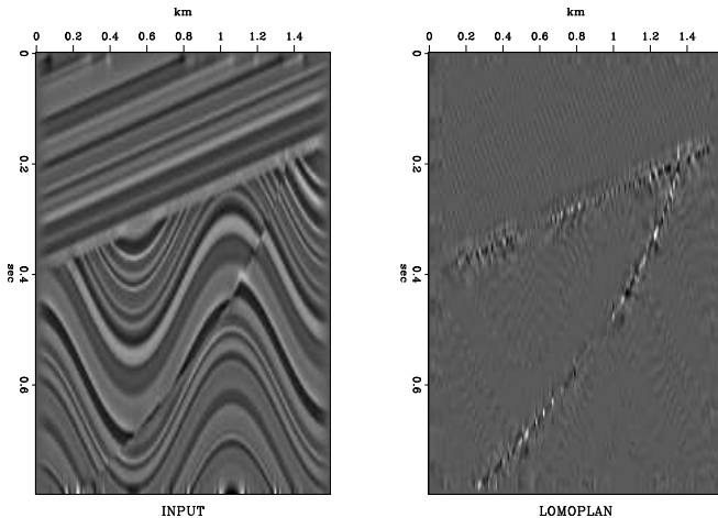
Figure 10.4: Left is a synthetic reflectivity model. Right is the result of local monoplane annihilation. lmm-sigmoid090 [ER]
