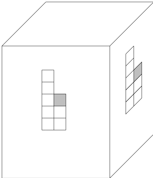
Figure 10.2: An inline 2-D PEF and a crossline 2-D PEF both applied throughout the volume. To find each filter, minimize each output power independently. lmn-rayab3Doper [NR]
