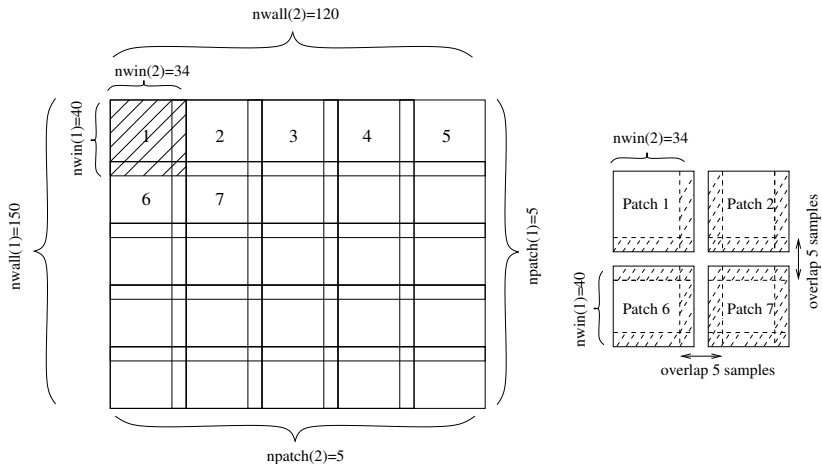
Figure 9.1: Decomposing a wall of information into windows (also called patches). Left is an example of a 2-D space input to module patch. Right shows a close-up of the output (top left corner). pch-antoine [NR]
