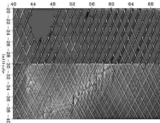
Figure 7.12: The roughened, normalized adjoint, \mathbf{H} \text{diag}(\mathbf{L}'\mathbf{1})^{-1}\mathbf{L}'\mathbf{d} . Some topography appears through the haze of the tracks. noiz-jesse2 [ER]
