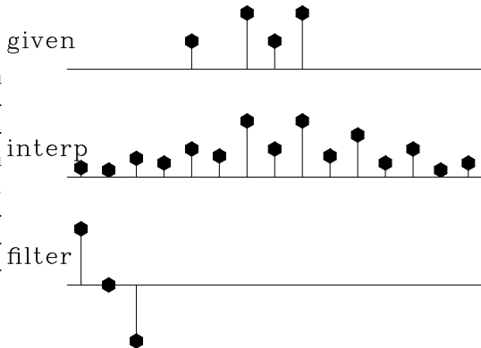
Figure 3.7: Top is the same as in Figures 3.3 to 3.6. Middle is interpolated. Bottom shows the filter (1, 0, -1) , which comes from the coefficients of (1, -1) * (1, 1) . Both the given data and the interpolated data have significant energy at both zero and Nyquist frequencies. iin-mbest90 [ER]
