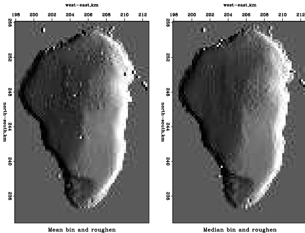
Figure 7.5: Galilee water depth binned and roughened. Left is binning with the mean, right with the median. noiz-medbin90 [ER,M]
