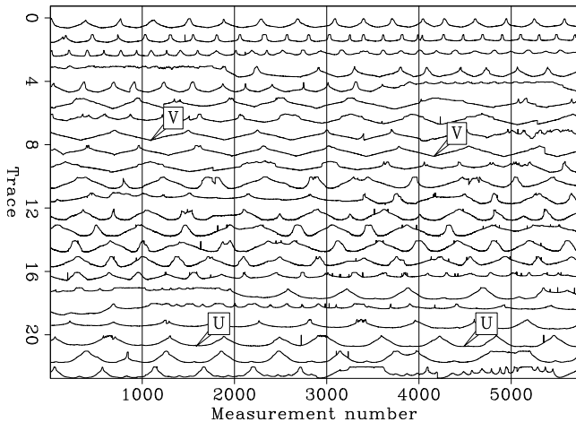
Figure 7.18: The complete Galilee data space. noiz-antoine1 [ER]
