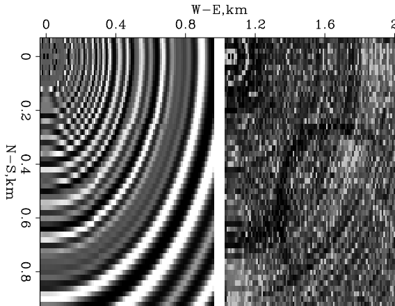
LOMOPLAN
