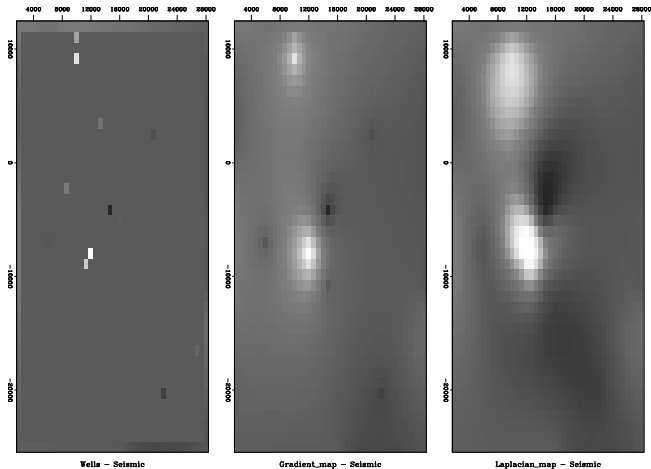
Figure 3.11: Difference between wells (the final map) and the extended seismic data. Left is plotted at the wells (with gray background for zero). Center is based on gradient roughening and shows tent-pole-like residuals at wells. Right is based on Laplacian roughening. iin-diffdiff90 [ER]
