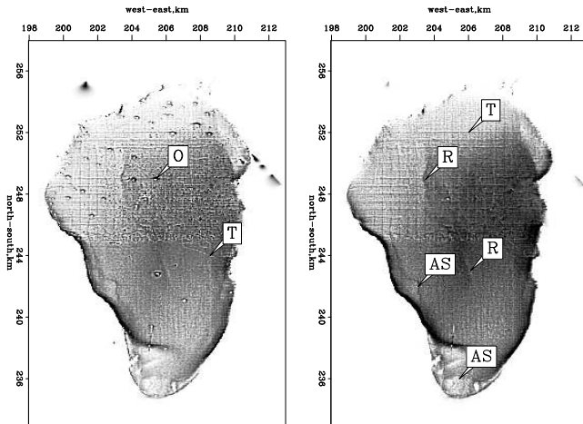
Figure 7.19: Estimated p in a least-squares sense (left) and in an \ell^1 sense (right). Pleasingly, isolated spikes are attenuated. Some interesting features are shown by the arrows: AS points to few ancient shores, O points to some outliers, T points to few tracks, and R points to a ridge. noiz-antoine2 [ER,M]
