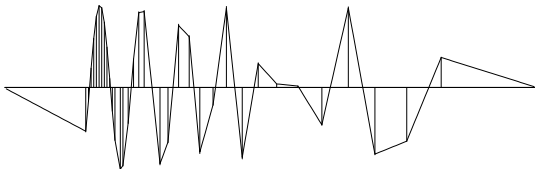
Figure 3.14: The same data samples and a function through them that minimizes the energy in the first derivative. iin-im1-1a90 [ER,M]
