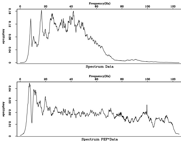
Figure 6.10: \omega spectrum of a shot gather of Figure 6.11 before and after 1-D decon. mda-antoinedecon1 [ER]
