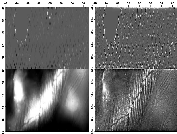
Figure 7.14: All data merged into a track-free image (hooray!) by applying the track derivative, not to the data, but to the residual. Left is \mathbf{h} estimated by \mathbf{0} \approx \mathbf{W} \frac{d}{dt} (\mathbf{L}\mathbf{h} - \mathbf{d}) . Right is the roughened altitude, \mathbf{p} = \mathbf{H}\mathbf{h} . noiz-jesse10 [ER,M]
