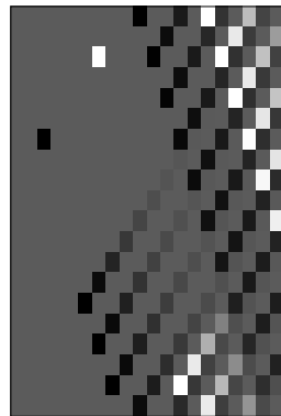
input/filter
