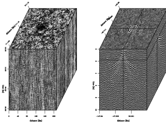
Figure 4.9: Left is raw data, vertical motion V(t, x, y) . Right is the derived impulse response. hlx-solar [ER,M]
