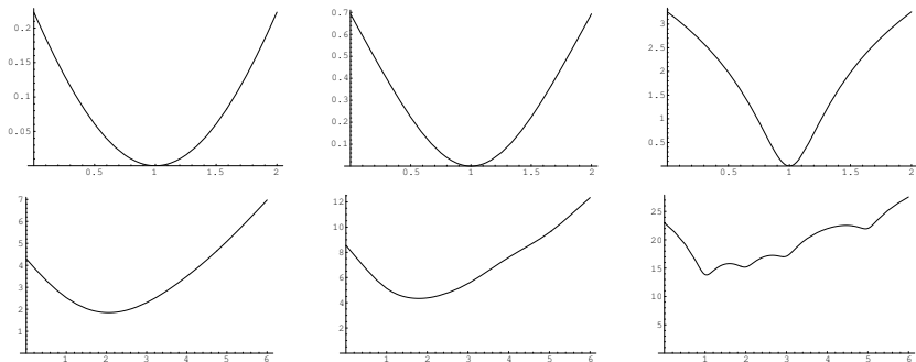
Figure 7.3: The coordinate is m . Top is Cauchy measures of m-1 . Bottom is the same measures of the data set (1,1,2,3,5) . Left, center, and right are for \bar{r} = (2,1,.2) . noiz-cauchy [CR]
