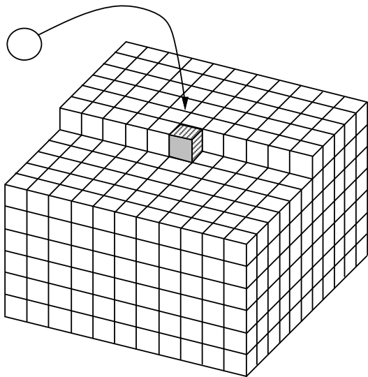
Figure 4.13: A 3-D causal filter at the starting end of a 3-D helix.
