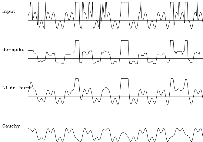
Figure 7.4: Top is synthetic data with noise spikes and bursts. (Most bursts are a hundred times larger than shown.) Next is after running medians. Bottom is after the two processes described here. noiz-burst90 [ER]
