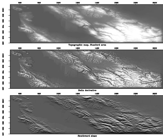
Figure 4.7: Topography, helical derivative, slope south. hlx-helocut90 [ER,M]
