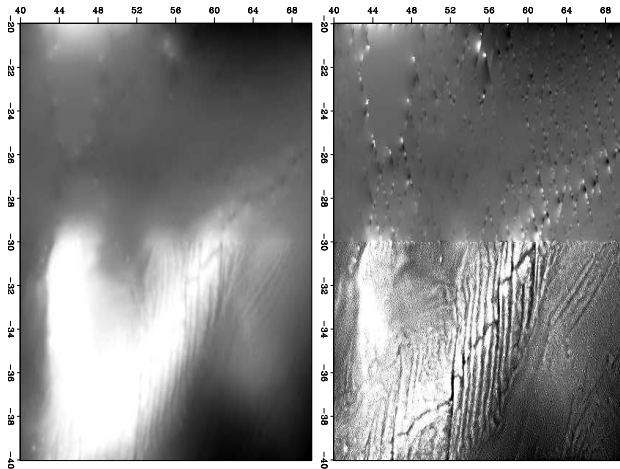
Figure 7.15: Using the track derivative in residual space and helix preconditioning in model space we start building topography in the north. Left is \mathbf{h} = \mathbf{H}^{-1}\mathbf{p} where \mathbf{p} is estimated by \mathbf{0} \approx \mathbf{W} \frac{d}{dt} (\mathbf{LH}^{-1}\mathbf{p} - \mathbf{d}) for only 10 iterations. Right is \mathbf{p} = \mathbf{H}\mathbf{h} .
