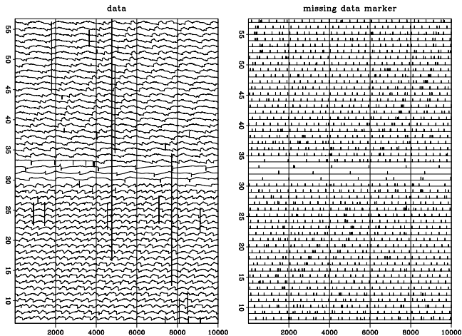
Figure 7.11: All the data d and the missing data markers. noiz-jesse5 [ER,M]
