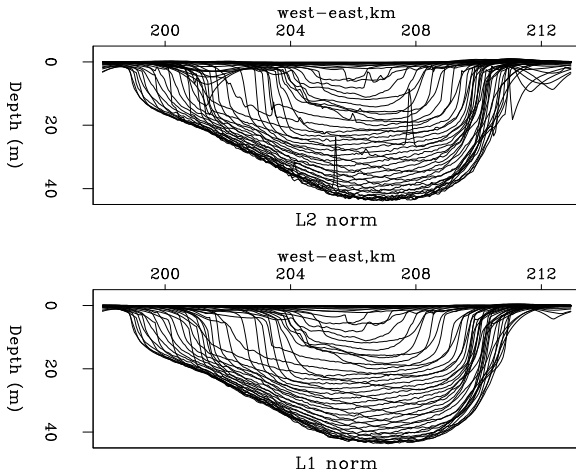
Figure 7.20: East-west cross sections of the lake bottom ( \mathbf{h} = \mathbf{H}^{-1}\mathbf{p} ). Top with the \ell^2 solution. Bottom with the \ell^1 approximating procedure. With \ell^1 , all depth values are positive and the spikes are attenuated. noiz-antoine3 [ER,M]
