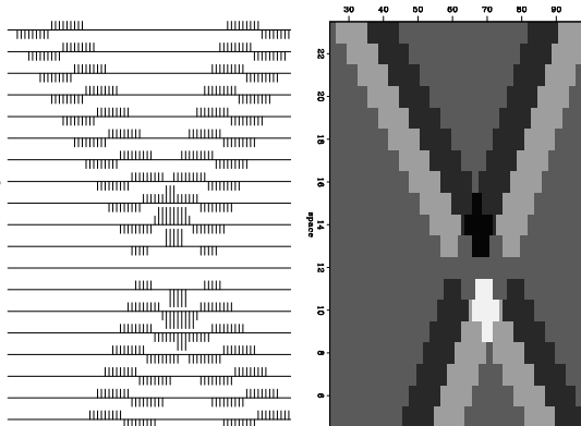
Figure 10.3: Superposition of plane waves of opposite polarity.
