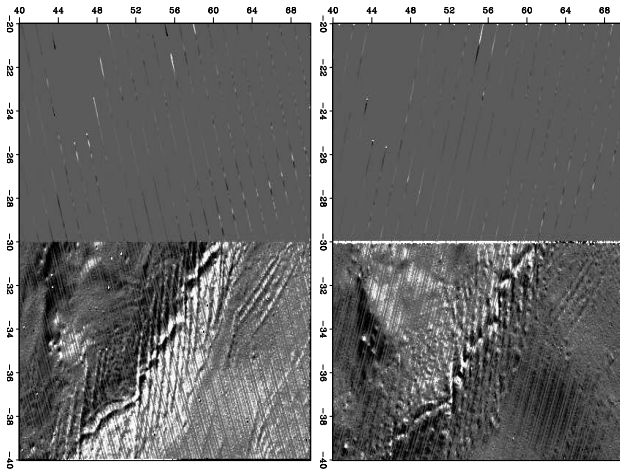
Figure 7.13: With a simple roughening derivative in data space, model space shows two nice topographic images. Let \mathbf{n} denote ascending tracks. Let \mathbf{s} denote descending tracks. Left is \mathbf{L}' \frac{d}{dt} \mathbf{n} . Right is \mathbf{L}' \frac{d}{dt} \mathbf{s} . noiz-jesse3 [ER,M]
