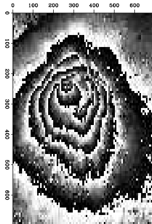
smoothed
