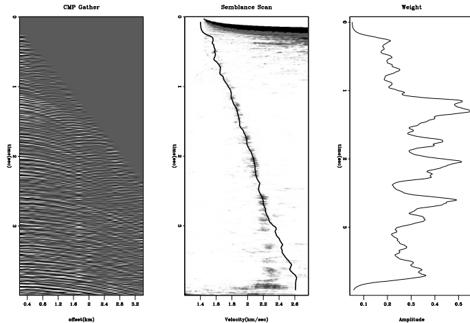
Figure 5.1: Raw CMP gather (left), Semblance scan (middle), and semblance value used for weighting function (right). (Clapp) prc-clapp [ER,M]
