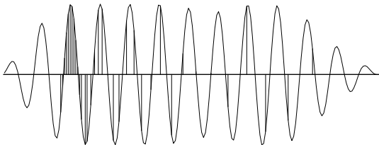
Figure 6.26: Interpolating with a three-term filter. The interpolated signal is fairly monofrequency.
