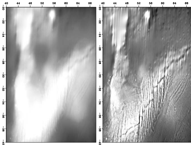
Figure 7.16: Given a PEF \mathbf{A} estimated on the densely defined southern part of the model, \mathbf{p} was estimated by \mathbf{0} \approx \mathbf{W} \frac{d}{dt} (\mathbf{L} \mathbf{A}^{-1} \mathbf{p} - \mathbf{d}) for 50 iterations. Left is \mathbf{h} = \mathbf{A}^{-1} \mathbf{p} . Right is \mathbf{p} = \mathbf{H} \mathbf{h} . noiz-jesse9 [ER,M]
