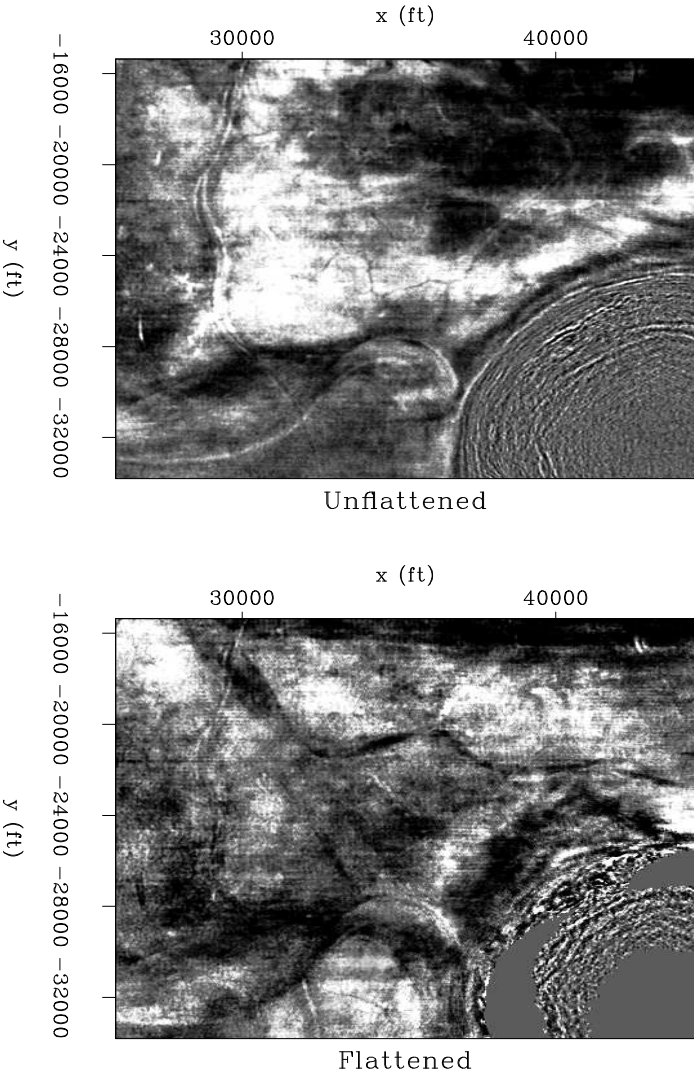
Figure 2.10: Slices of constant time before and after flattening. Notice the rings surrounding the dome are gone giving the dome a reduced diameter. (Ignore the inside of the dome.)
