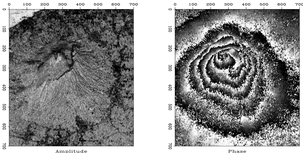
Figure 2.11: Radar image of Mt. Vesuvius. Left is the amplitude |Z(x, y)| . Non-reflecting ocean in upper left corner. Right is the phase \arctan(\text{Re } Z(x, y), \text{Im } Z(x, y)) . (Umberto Spagnolini) VIEW lsq/. vesuvio90
