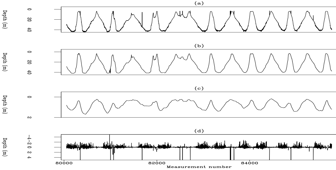
Figure 7.20: (a) Track 14 (input data) in Figure 7.13. (b) Modeled data, \mathbf{B}\mathbf{H}^{-1}\mathbf{p} . (c) Estimated drift. (d) Data-space residual. Notice the residual is large in deep water and it tends to negative polarity. VIEW noiz/. antoine6
