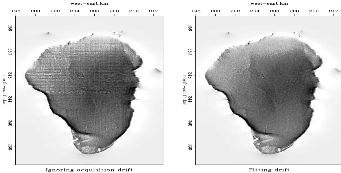
Figure 7.17: LEFT: Estimated \mathbf{p} without attenuation of the tracks, i.e., regression (7.62). RIGHT: Estimated \mathbf{p} without tracks, i.e., regression (7.65). VIEW noiz/. antoine4
