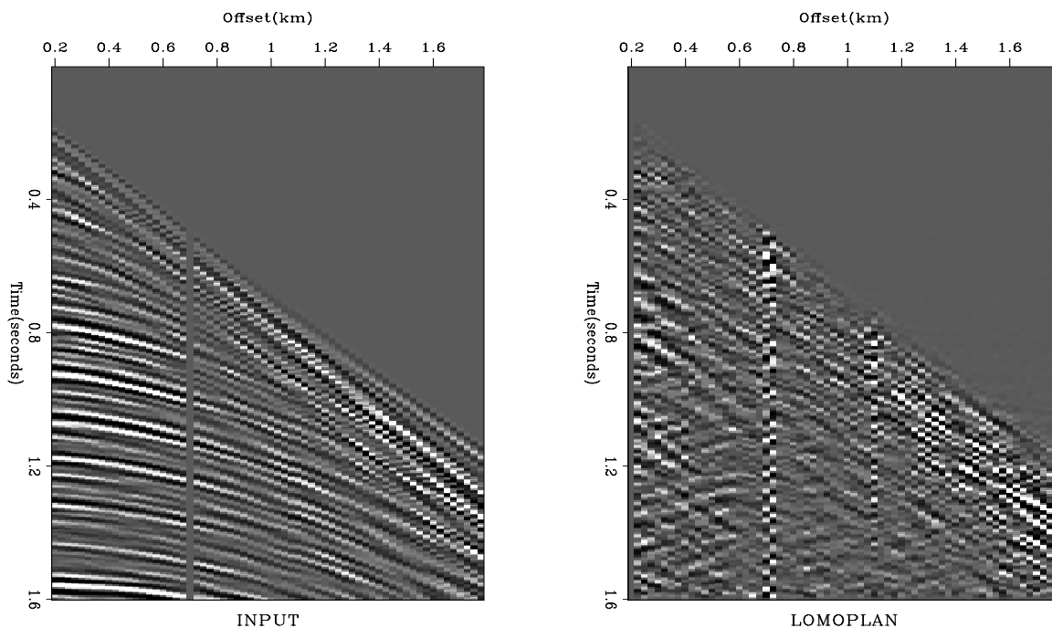
Figure 10.7: Portion of Yilmaz and Cumro data set 27 (left) and after LOMOPLAN (right). Press button for movie. VIEW lmn/. yc2790
