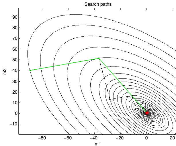
Figure 2.7: Route of steepest descent (black) and route of conjugate direction (light grey or green).
