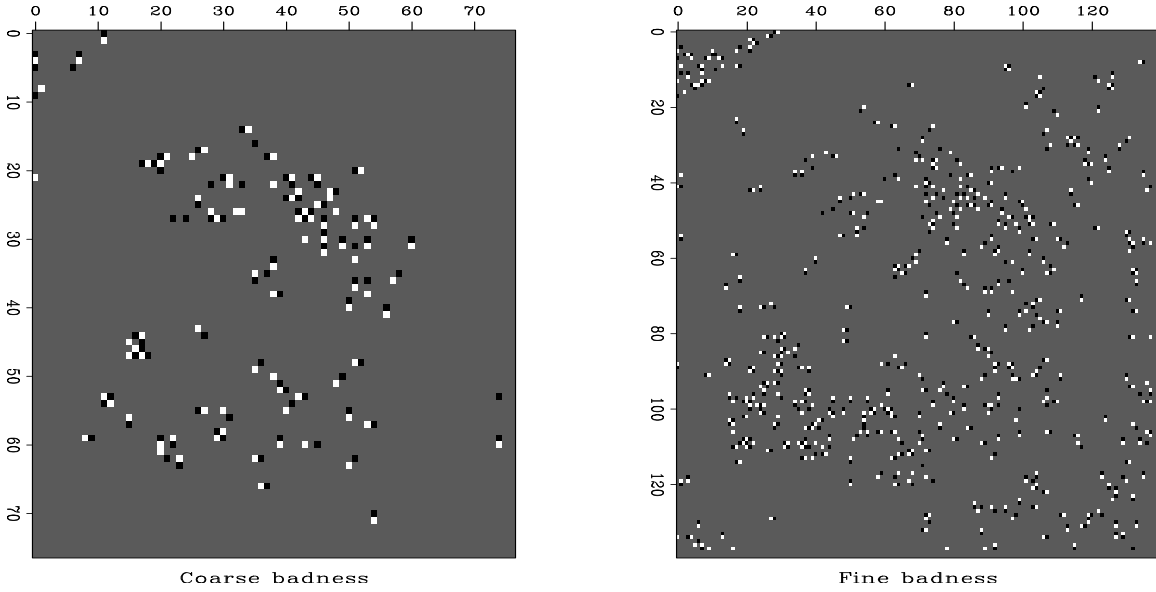
Figure 2.14: Values of curl at Vesuvius. The bad data locations at both coarse and fine resolution tend to occur in pairs of opposite polarity. VIEW lsq/. screw90
