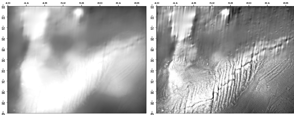
Figure 7.11: Given a PEF \mathbf{A} estimated on the densely defined southern part of the model, \mathbf{p} was estimated by \mathbf{0} \approx \mathbf{W} \frac{d}{dt} (\mathbf{L} \mathbf{A}^{-1} \mathbf{p} - \mathbf{d}) for 50 iterations. Left is \mathbf{h} = \mathbf{A}^{-1} \mathbf{p} . Right is \mathbf{p} = \mathbf{H} \mathbf{h} . VIEW noiz/. jesse9
