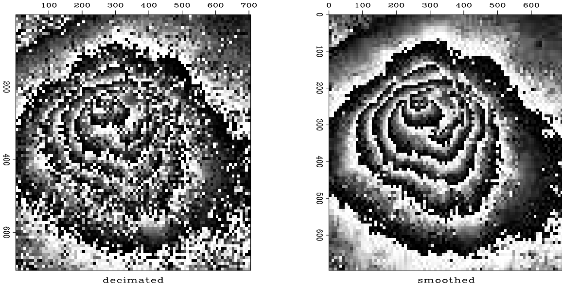
Figure 2.12: Phase based on decimated data (left) and smoothed data (right).
