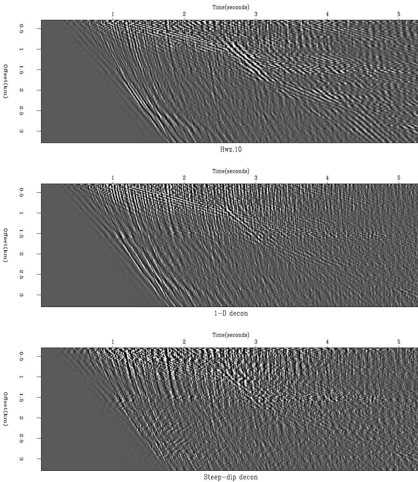
Figure 9.10: Top is a North African vibrator shot profile (Y&C #10) after AGC. Middle is gapped 1-D decon. Bottom is steep-dip decon. VIEW pch/. wz-1090
