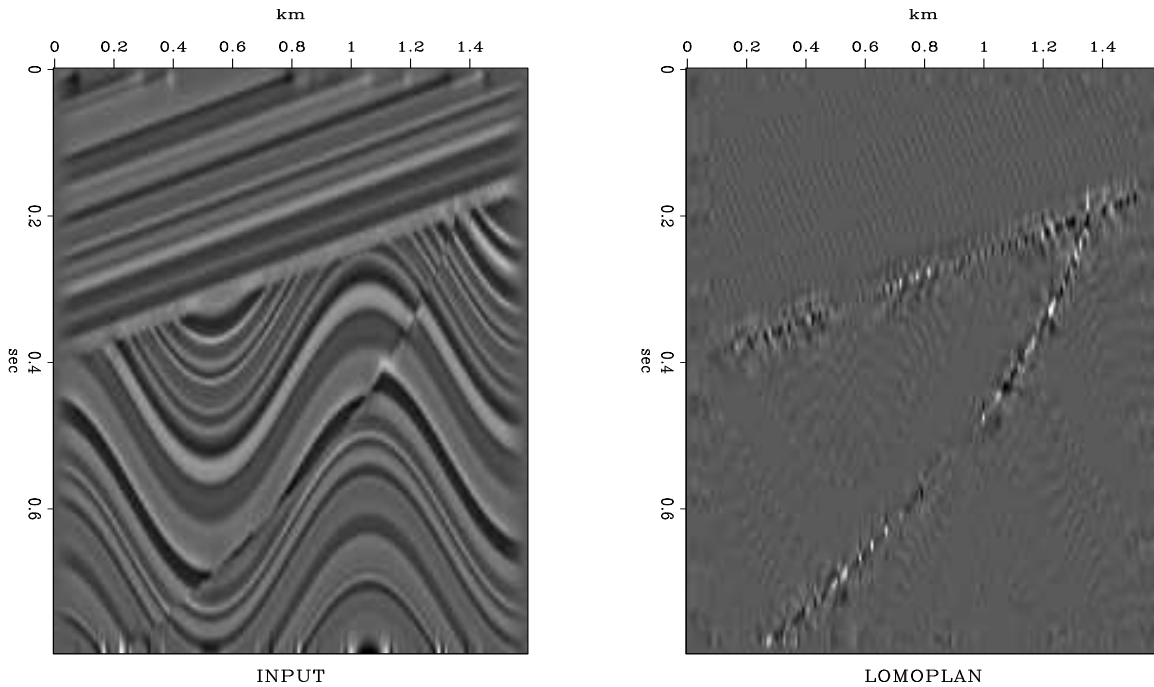
Figure 10.4: Left is a synthetic reflectivity model. Right is the result of local monoplane annihilation. VIEW lmn/. sigmoid090
