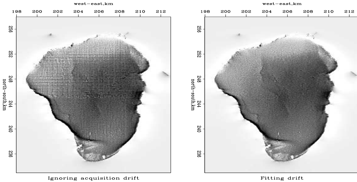
Figure 7.16: LEFT: Estimated \mathbf{p} without attenuation of the tracks, i.e., regression (7.50). RIGHT: Estimated \mathbf{p} without tracks, i.e., regression (7.53). VIEW noiz/. antoine4
