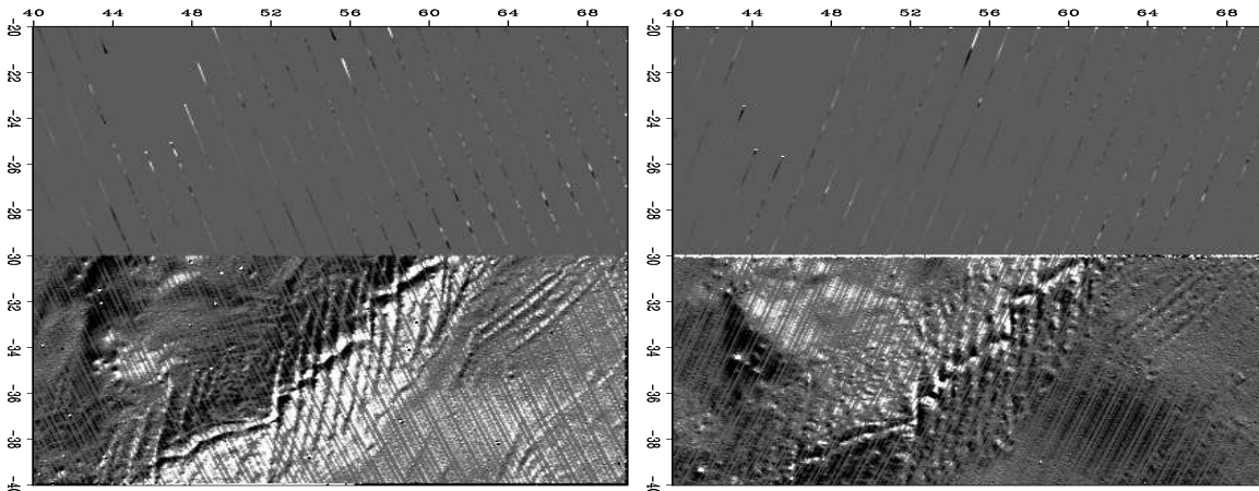
Figure 7.7: With a simple roughening derivative in data space, model space shows two nice topographic images. Let \mathbf{n} denote ascending tracks. Let \mathbf{s} denote descending tracks. Left is \mathbf{L}^T \frac{d}{dt} \mathbf{n} . Right is \mathbf{L}^T \frac{d}{dt} \mathbf{s} . VIEW noiz/. jesse3
