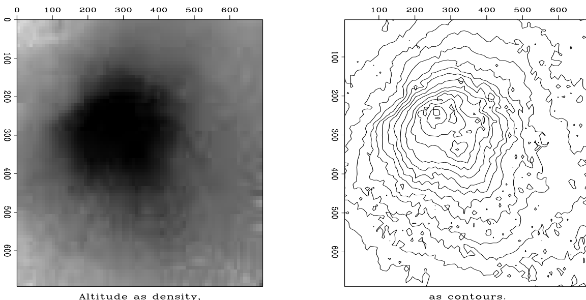
Figure 2.12: Estimated altitude.
