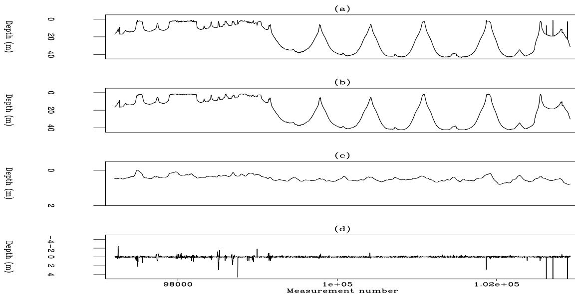
Figure 7.18: (a) Track 17 (input data) in Figure 7.12. (b) The estimated noise-free data \mathbf{BH}^{-1}\mathbf{p} . (c) Estimated drift \mathbf{Lq} . (d) Data residual. VIEW noiz/. antoine5
