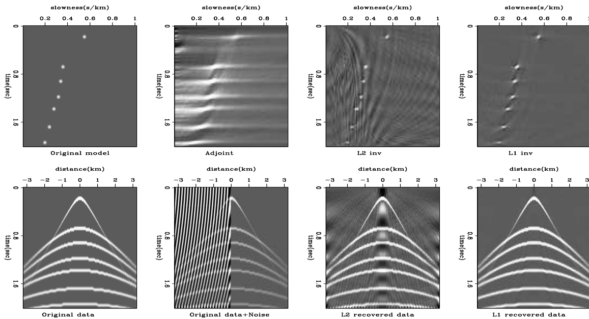
Figure 7.3: Inversion of hyperbolic transformation by means of (1) adjoint, (2) inverse with \ell_2 norm, and (3) inverse with \ell_1 norm. VIEW noiz/. vel-gboyega2
