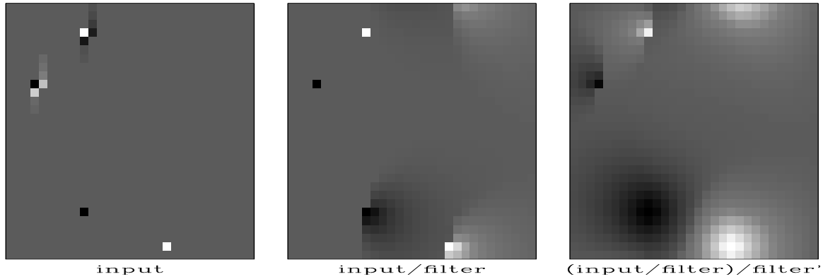
Figure 4.8: Deconvolution by a filter whose autocorrelation is the two-dimensional Laplacian operator. Amounts to solving the Poisson equation. Left is \Pi ; Middle is \Pi/\mathcal{H} ; Right is (\Pi/\mathcal{H})/\mathcal{H}^T . VIEW hlx/. lapfac90
