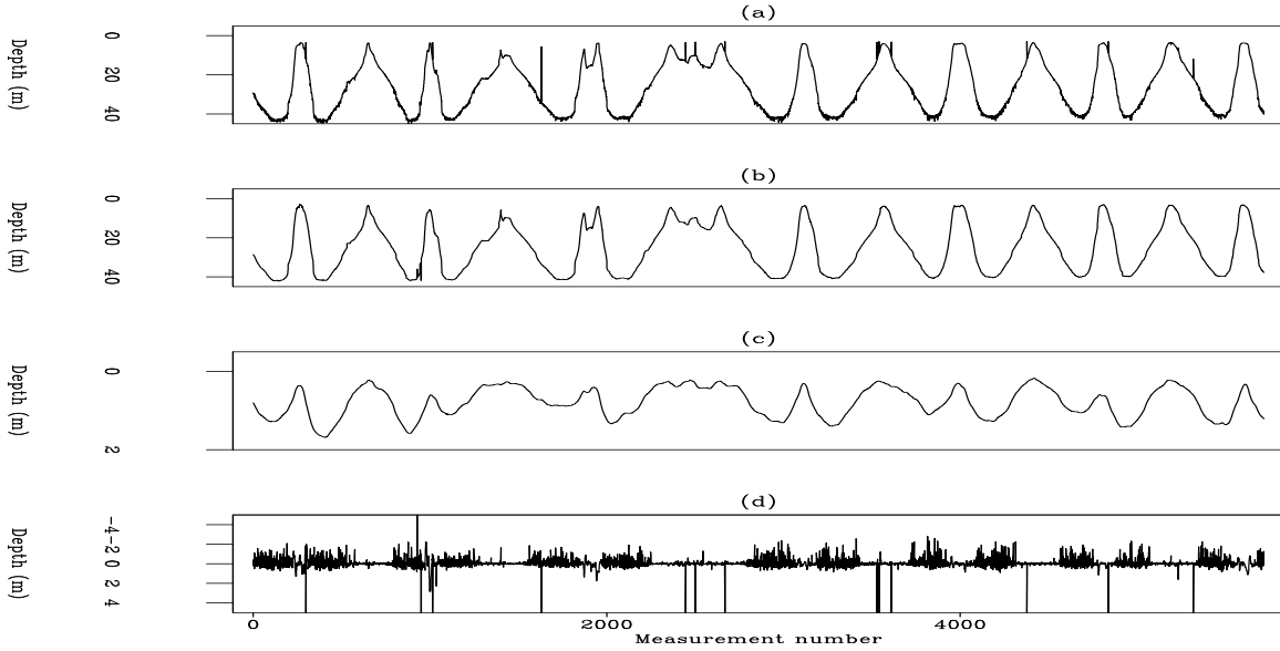
Figure 7.19: (a) Track 14 (input data) in Figure 7.12. (b) Modeled data, \mathbf{BH}^{-1}\mathbf{p} . (c) Estimated drift. (d) Data-space residual. Notice the residual is large in deep water and it tends to negative polarity. VIEW noiz/. antoine6
