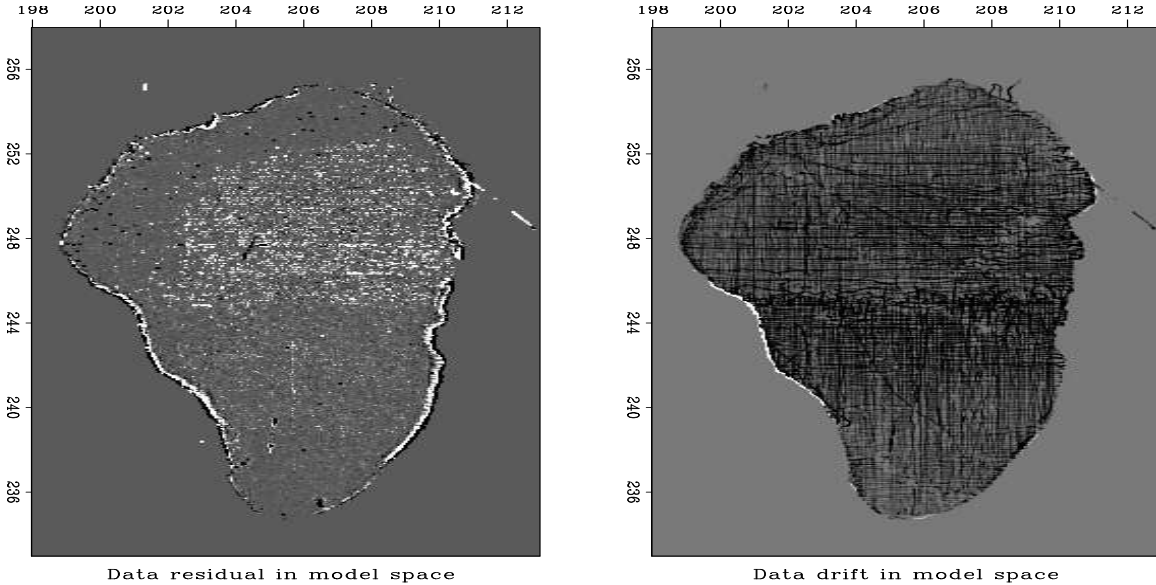
Figure 7.17: (LEFT) Data residual brought back into model space \mathbf{B}^T \mathbf{r}_d . Mostly noise with some geography. (RIGHT) Data drift brought back into model space \mathbf{B}^T \mathbf{L} \mathbf{q} . Mostly tracks with a bit of geography. VIEW noiz/. antoine7
