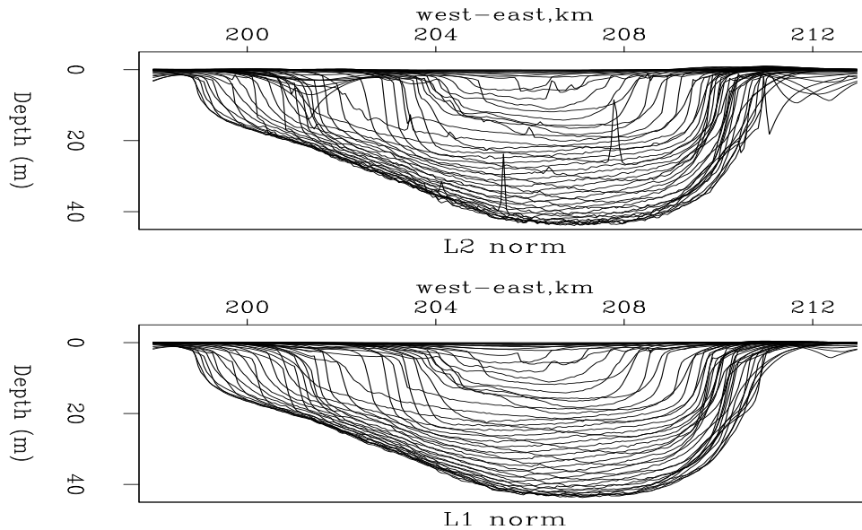
Figure 7.14: East-west cross sections of the lake bottom ( \mathbf{h} = \mathbf{H}^{-1}\mathbf{p} ). Top with the \ell^2 solution. Bottom with the \ell^1 approximating procedure. VIEW noiz/. antoine3
