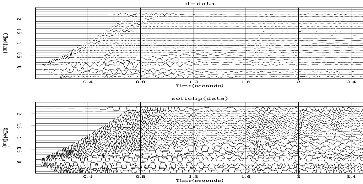
Figure 7.2: Reflection data \mathbf{d} before (top) and after (bottom) soft clip C'(\mathbf{d}) . Clipping large amplitudes enables small ones to be seen. VIEW noiz/. softclip
