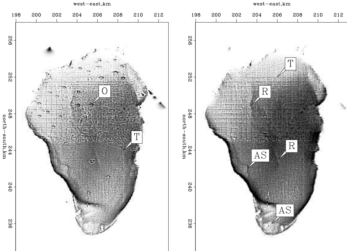
Figure 7.13: Estimated \mathbf{p} in a least-squares sense (left) and in an \ell^1 sense (right). Pleasingly, isolated spikes are attenuated. Some interesting features are shown by the arrows: AS points to few ancient shores, O points to some outliers, T points to few tracks, and R points to a curious feature. VIEW noiz/. antoine2
