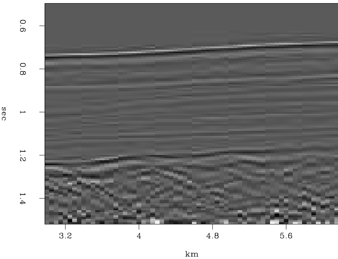
p(t,x)
