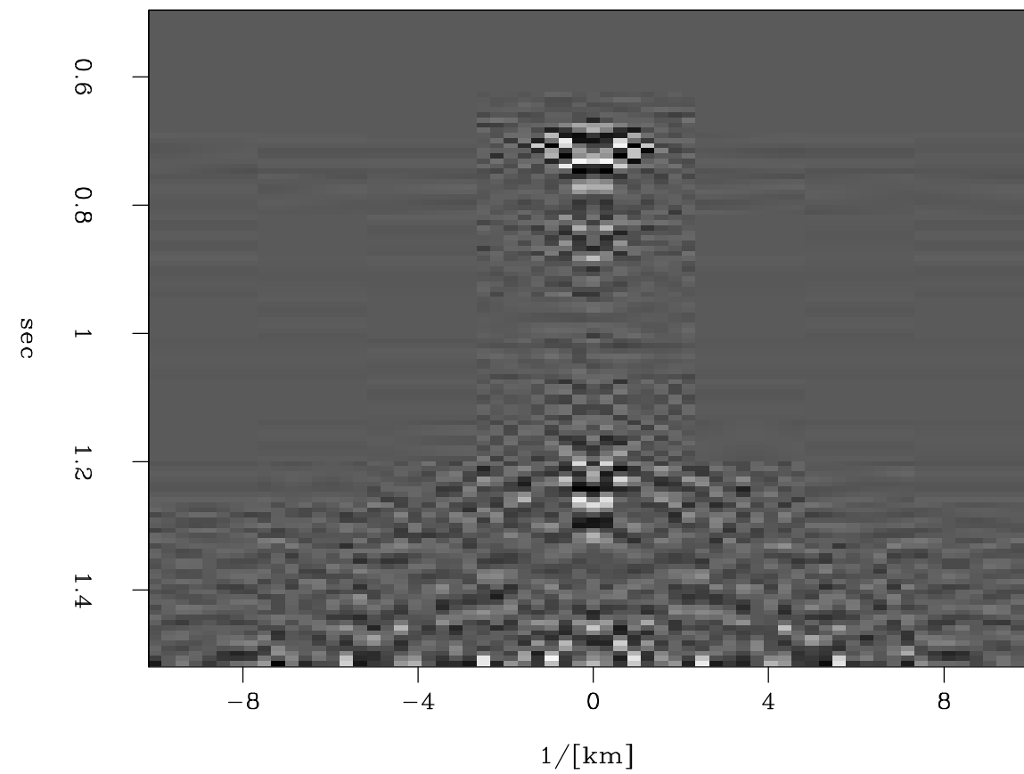
P(t,k_x)
