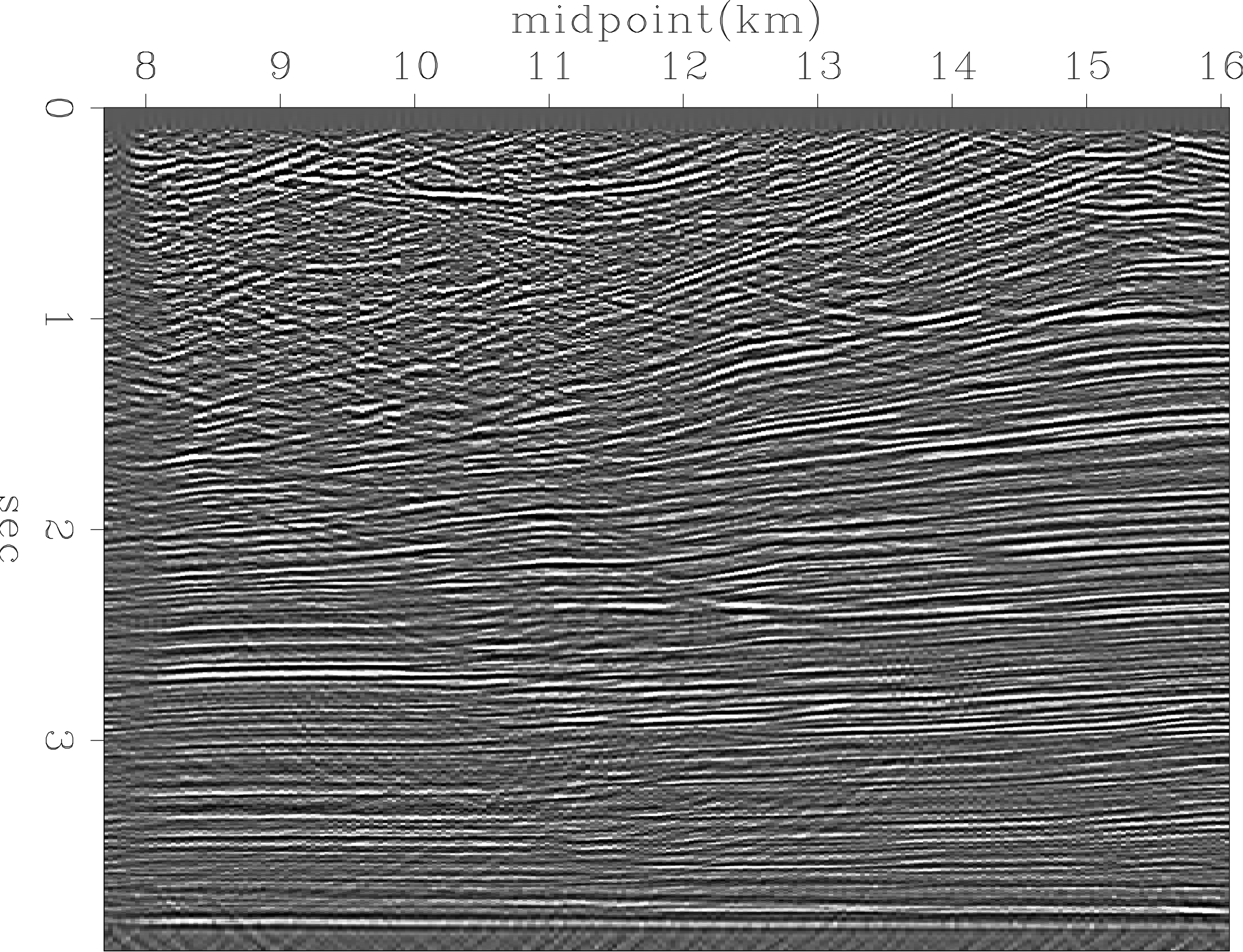
Phase-shift migration
