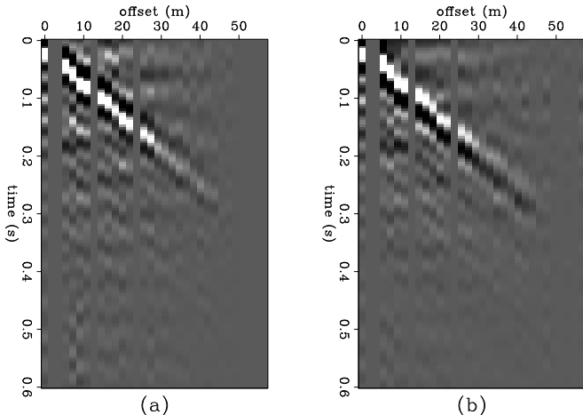
Figure 2: 3-D impulse response summed over azimuth calculated by two methods, (a) 3-D autocorrelation, and (b) spectral factorization. (James Rickett) longimp [NR,M]
