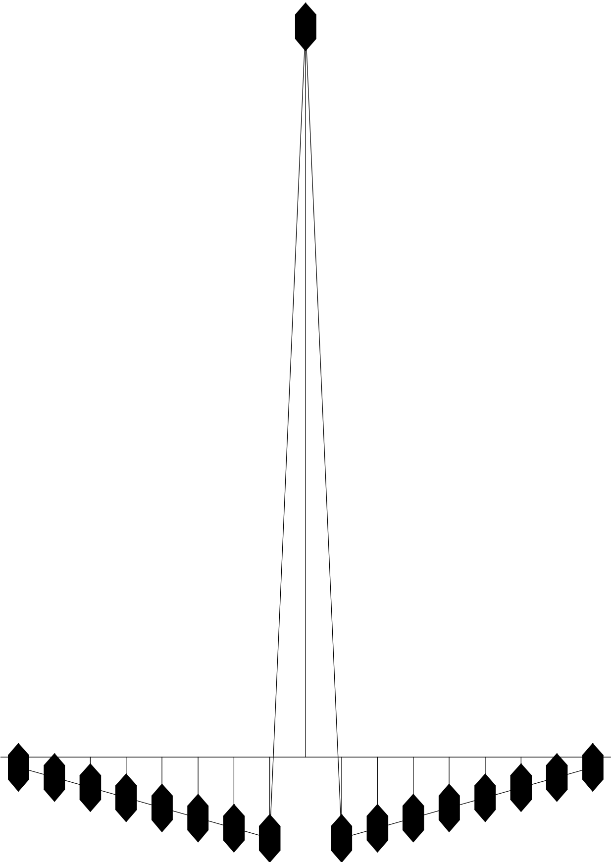
1-D Laplace operator
