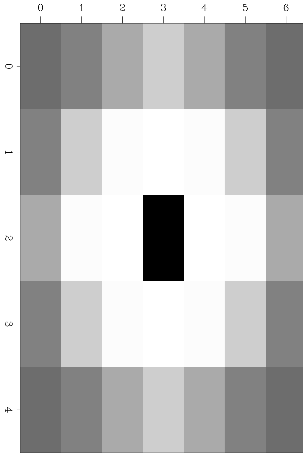
2-D Laplace operator
