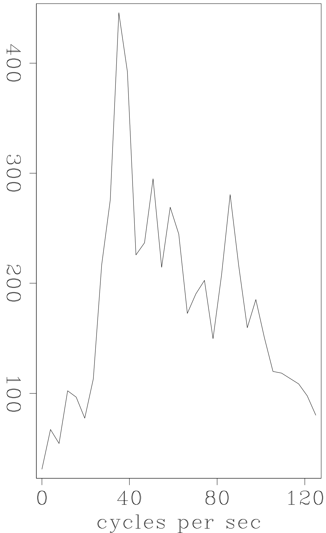
Amplitude Spectrum
