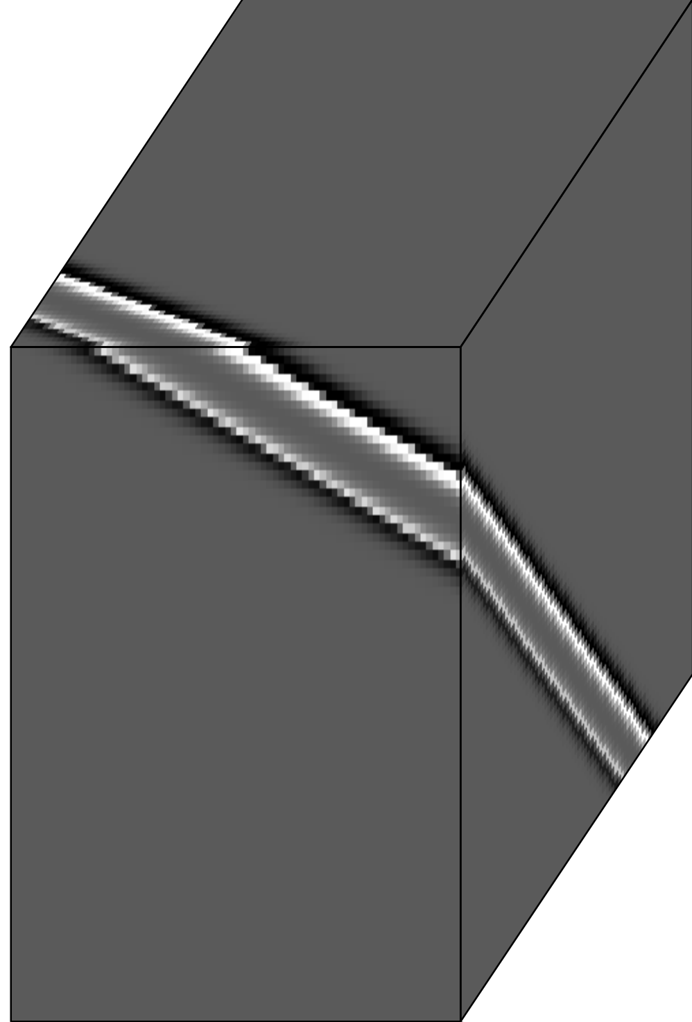
Laplace operator
