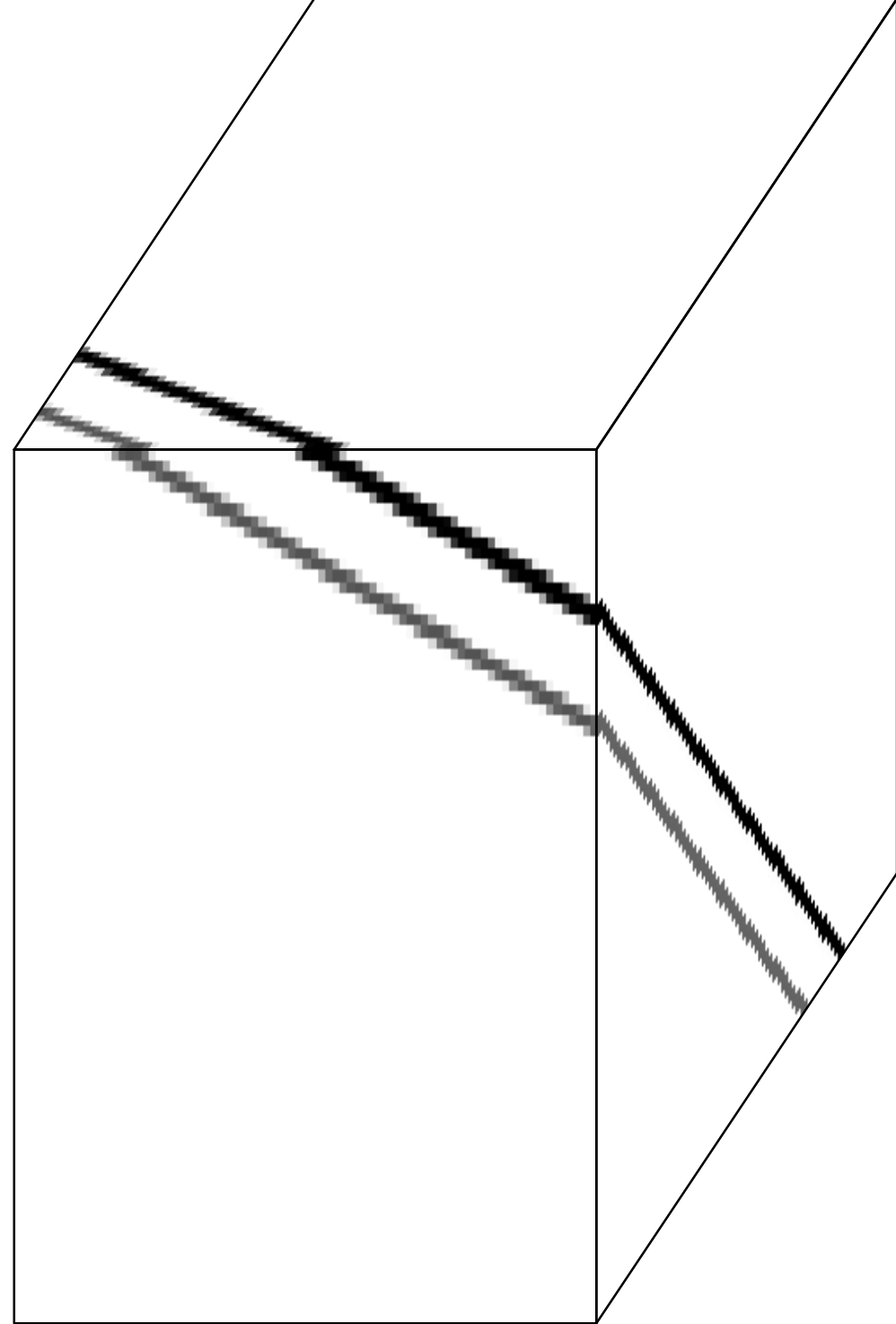
Gradient operator
