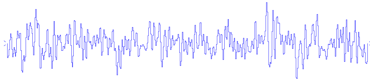
Squared FT
