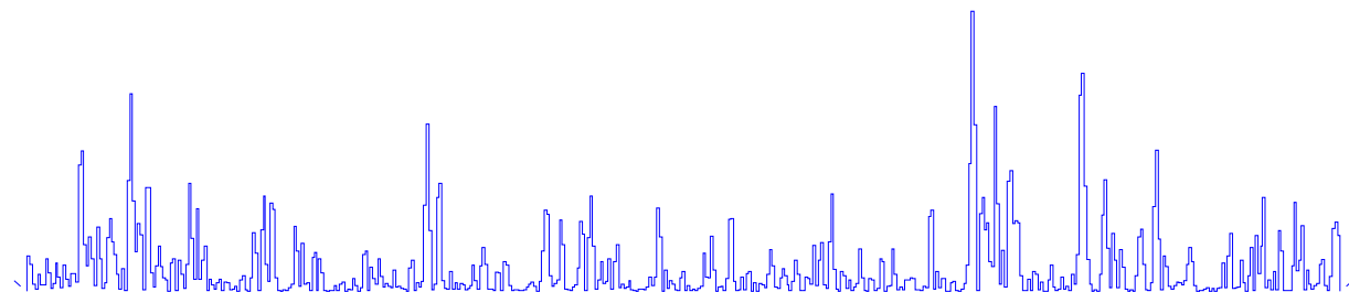
Squared FT
