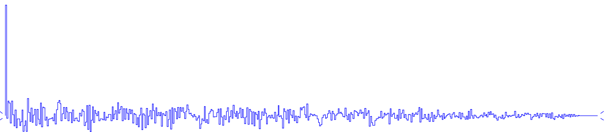
Autocorrelation
