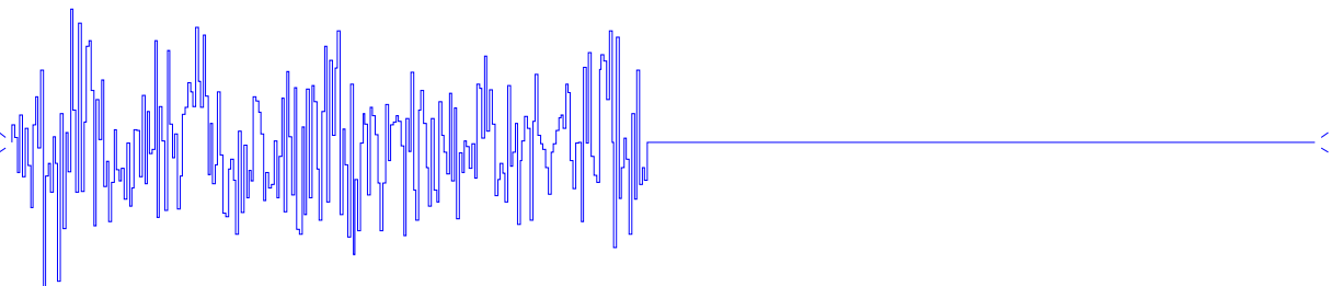
Autocorrelation
