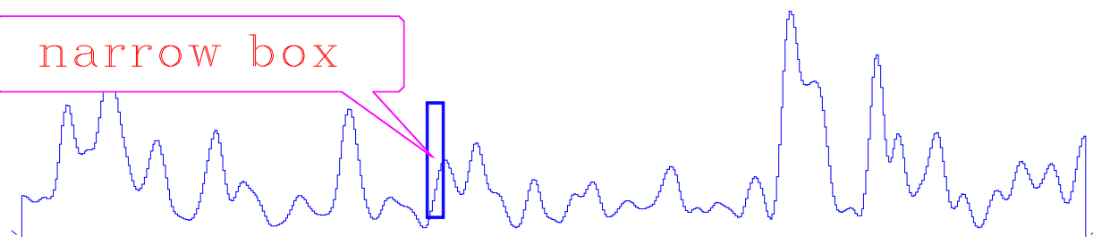
Smother spectrum
