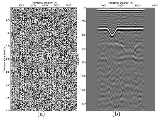
Fig. 10: (a) Simulated reflection shot panel from 20 seconds long noise recordings with a simulated shot position at x_1 = 4000 m. (b) Result from direct migration of 20 seconds long noise recordings.
