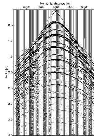
Fig. 11: Directly modelled reflection response for the double syncline model from figure 2 (a) with a shot at x = (4000, 0) m.
