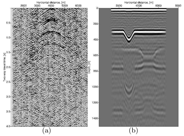
Fig. 3: (a) Simulated reflection shot panel from 6 minutes long noise recordings with 113 regularly distributed subsurface sources with a simulated shot position at x_1 = 4000 m. (b) Result from direct migration of 6 minutes long noise recordings with 113 regularly distributed subsurface sources.
