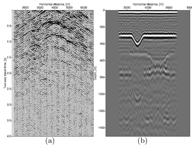
Fig. 5: (a) Simulated reflection shot panel from 6 minutes long noise recordings with 11 regularly distributed subsurface sources with a simulated shot position at x_1 = 4000 m. (b) Result from direct migration of 6 minutes long noise recordings with 11 regularly distributed subsurface sources.
