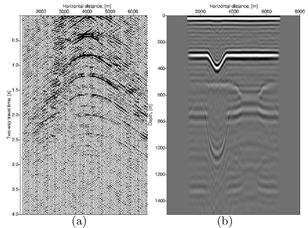
Fig. 7: (a) Simulated reflection shot panel from 33 minutes long noise recordings with a simulated shot position at x_1 = 4000 m. (b) Result from direct migration of 33 minutes long noise recordings.
