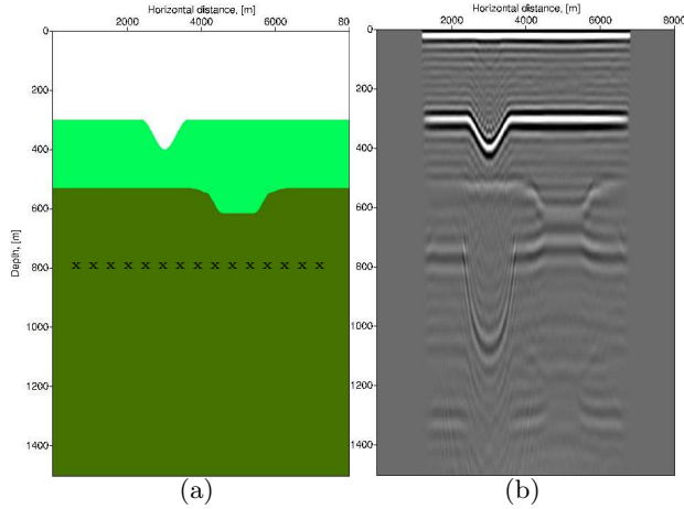
Fig. 2: (a) Double syncline model with white-noise sources at depth level x_3 = 800 m; the sources are regularly distributed; the receivers at the surface are distributed between x_1 = 1200 and x_1 = 6800 m every 20 m; (b) The migrated image from the direct migration and from the migration of the simulated reflection shot panels are identical; the transmission responses used here were 66 minutes long recordings in the presence of subsurface sources placed every 25 m between x_1 = 1200 and x_1 = 6800 m.
