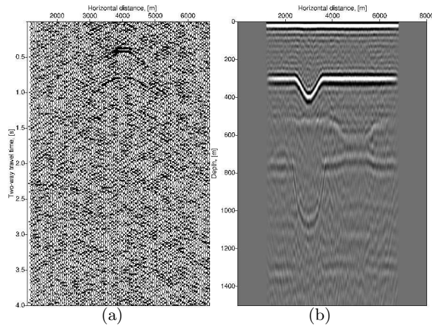
Fig. 9: (a) Simulated reflection shot panel from 1 minute long noise recordings with a simulated shot position at x_1 = 4000 m. (b) Result from direct migration of 1 minute long noise recordings.
