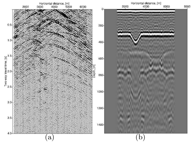
Fig. 6: (a) Simulated reflection shot panel from 6 minutes long noise recordings with 6 regularly distributed subsurface sources with a simulated shot position at x_1 = 4000 m. (b) Result from direct migration of 6 minutes long noise recordings with 6 regularly distributed subsurface sources.
