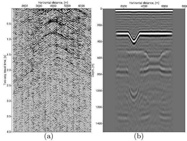
Fig. 4: (a) Simulated reflection shot panel from 6 minutes long noise recordings with 57 regularly distributed subsurface sources with a simulated shot position at x_1 = 4000 m. (b) Result from direct migration of 6 minutes long noise recordings with 57 regularly distributed subsurface sources.
