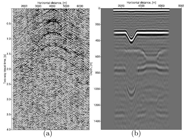
Fig. 8: (a) Simulated reflection shot panel from 6 minutes long noise recordings with a simulated shot position at x_1 = 4000 m. (b) Result from direct migration of 6 minutes long noise recordings.
