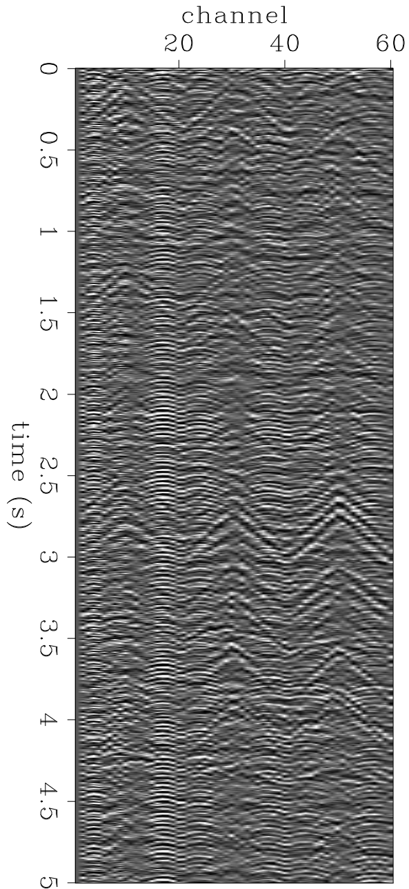
Figure 1: Noise record. Raw data. Data was laid out as parallel lines, alternate lines in reverse direction (i.e. one long line folded back upon itself). (Bryan Kerr) strip [NR]
