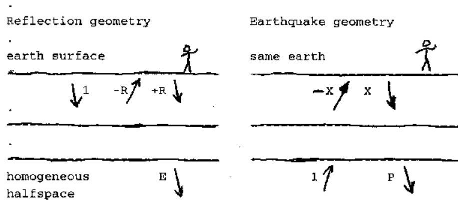
Figure 3: Pancake earth with prospector’s boundary conditions (left) and earthquake boundary conditions (right) eqcor [NR]
