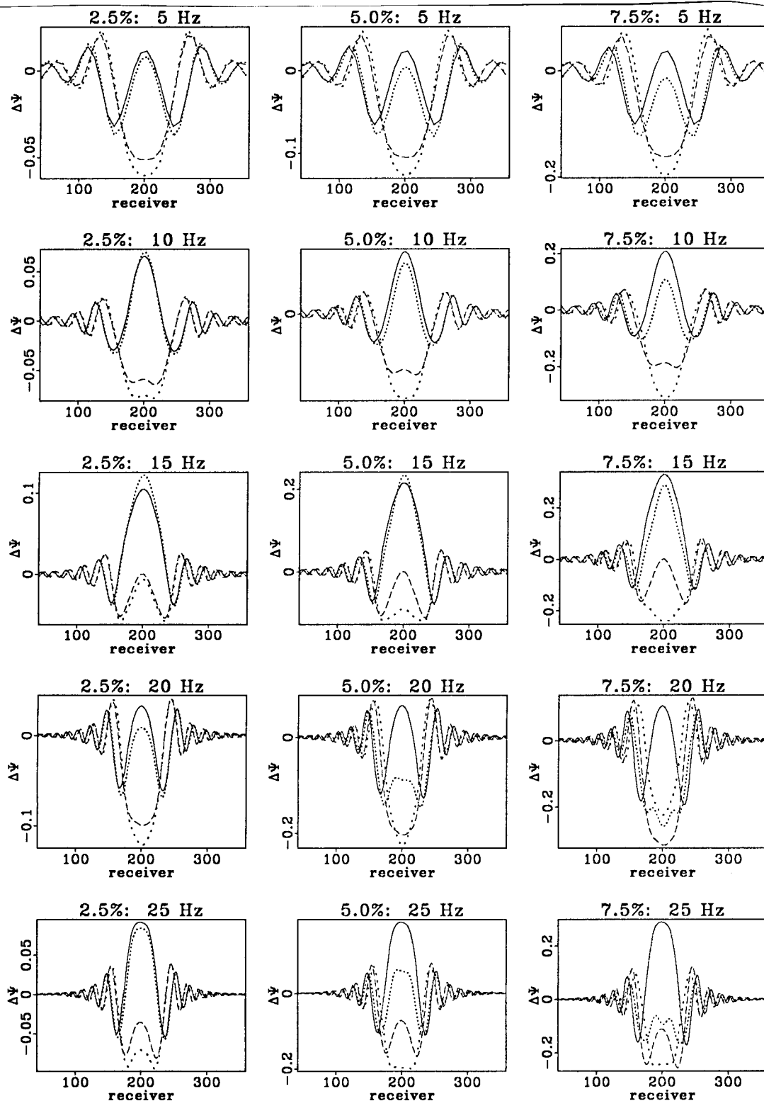
FIG. 1. (a) Born data: the solid and dashed lines correspond to the imaginary and real parts of \Delta\psi predicted by the Born approximation; the finely and coarsely dotted lines correspond to the imaginary and real parts of \Delta\psi in the finite-difference generated data.
