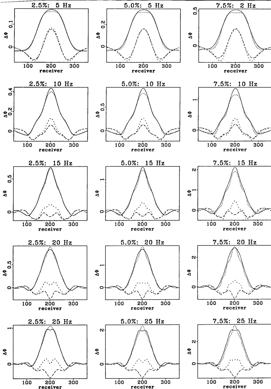
FIG. 1. (b) Rytov data: the solid and dashed lines correspond to the imaginary and real parts of \Delta\phi predicted by the Rytov approximation; the finely and coarsely dotted lines correspond to the imaginary and real parts of \Delta\phi in the finite-difference generated data.
