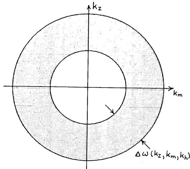
FIG. 2. The shaded ring shows the region of resolution of the bulk modulus and density variations. Here k_z , k_m , and k_h are respectively the vertical, the midpoint, and the offset wavenumbers. The width and radius of the ring depend on the passband \Delta\omega of the source time function. As the ratio k_h/k_z is increased, the radius of the ring shrinks. This corresponds in the physical domain to increasing the source-receiver offset relative to the depth to the reflector.
