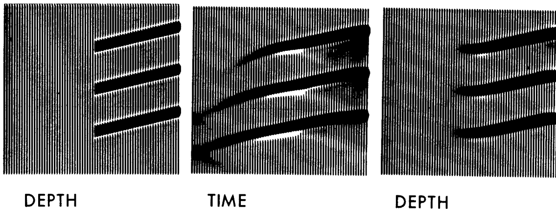
FIG. 12. Like Figure 11 except that the beds have dip. Note that the hyperbolas stay in place but in the time data the interfaces slide down and to the left. (They migrate.) The hyperbolas in the time data would become far more dominant if data were recorded with automatic gain control.
