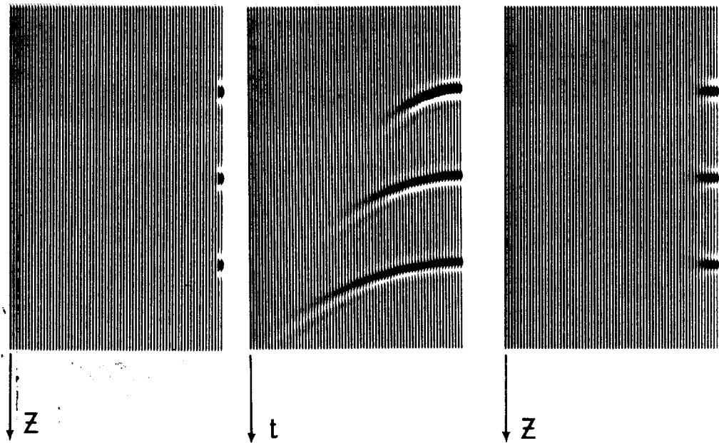
FIG. 10. This is like Figure 8 but the computer grid was not quite fine enough. Note "tails" on the ends of the hyperbolas. The resulting error is explained in the frequency domain in Figure 6. Note that the reconstruction is unaffected. Thus, the ability to reconstruct does not assure a high-quality migration.
