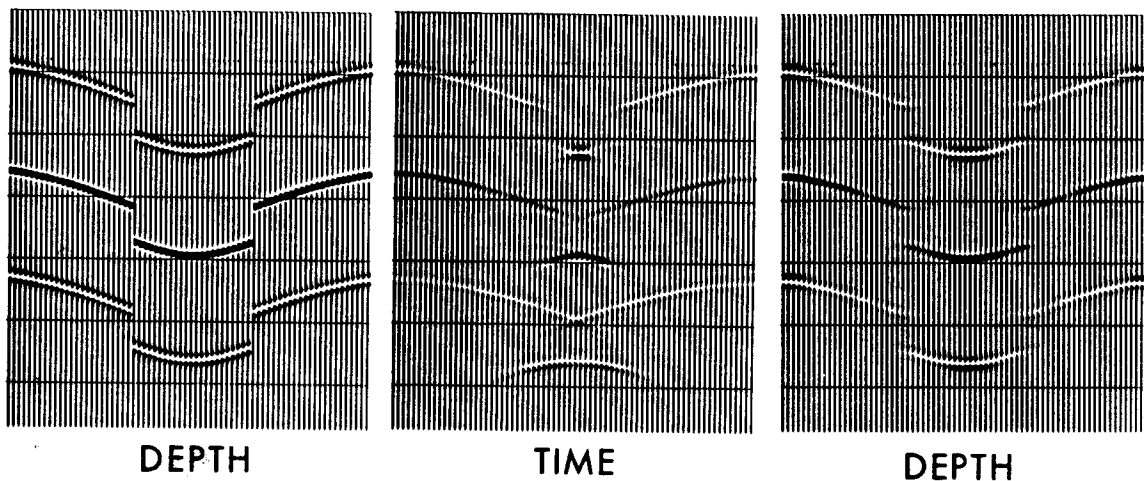
FIG. 13. The classical graben or buried-channel model. Each discontinuity in the depth section gives rise to a faint hyperbola in time.
