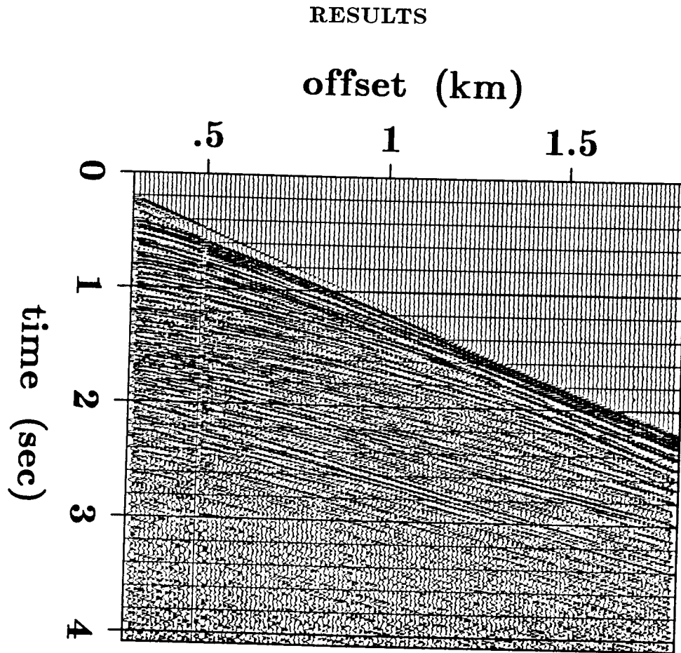
FIG. 1. A typical marine shot gather used for migration velocity analysis.
