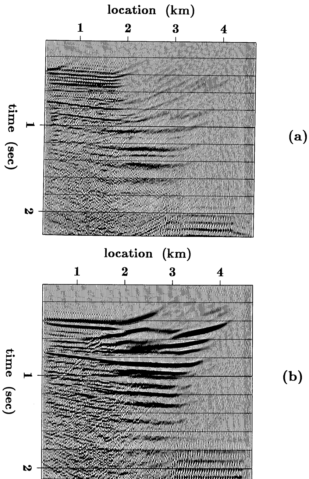
FIG. 8. Stacks of migrated profiles. (a) Migration velocity=1.4 km/sec. (b) Migration velocity=1.5 km/sec.
