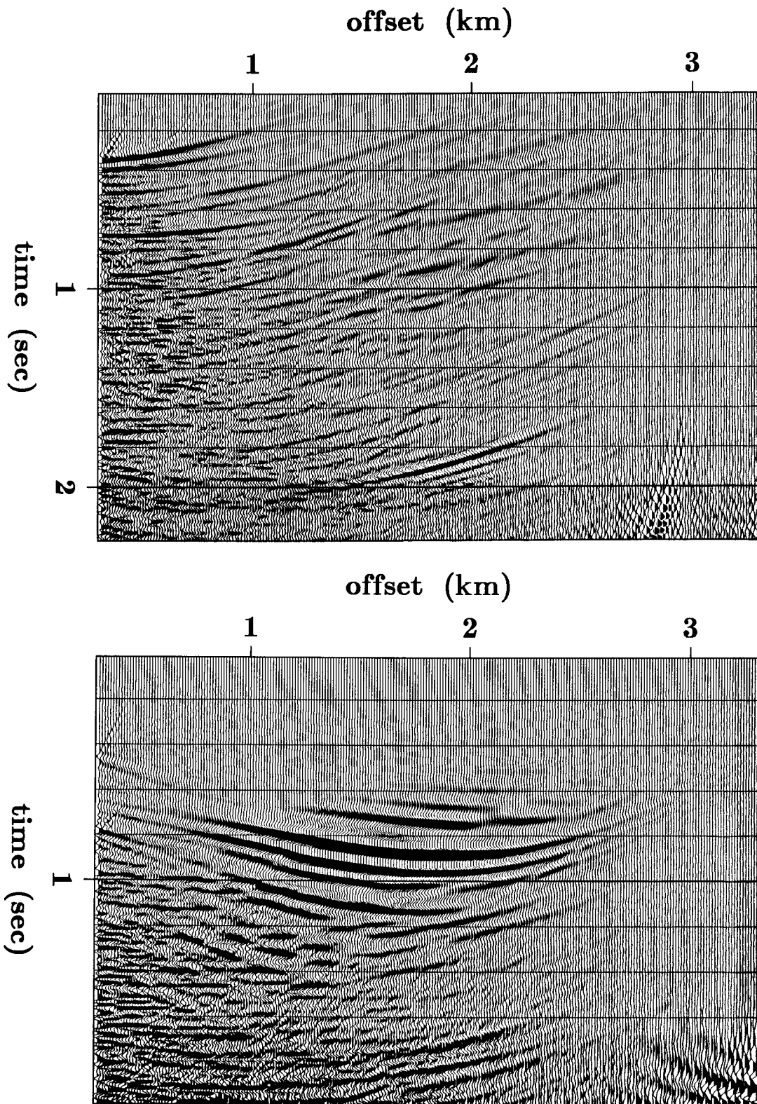
FIG. 5. The result of migrating the gather in Figure 1 with a velocity of 1.4 km/sec (top) and 1.6 km/sec (bottom).
