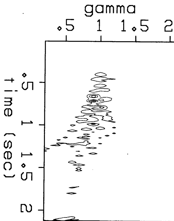
FIG. 4. A velocity panel showing coherency as a function of \gamma and travel-time depth for a migration velocity of 1.5 km/sec.
