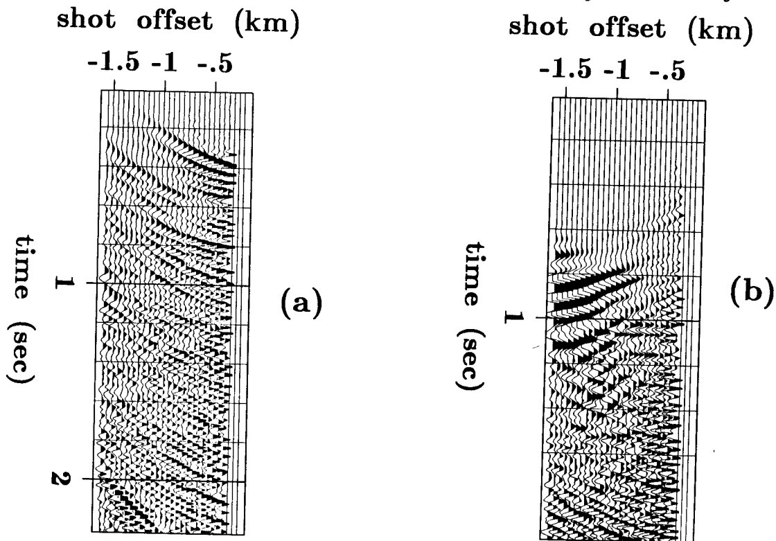
FIG. 6. (a) A CRG obtained at migration velocity of 1.4 km/sec. (b) A CRG obtained at migration velocity of 1.6 km/sec.
