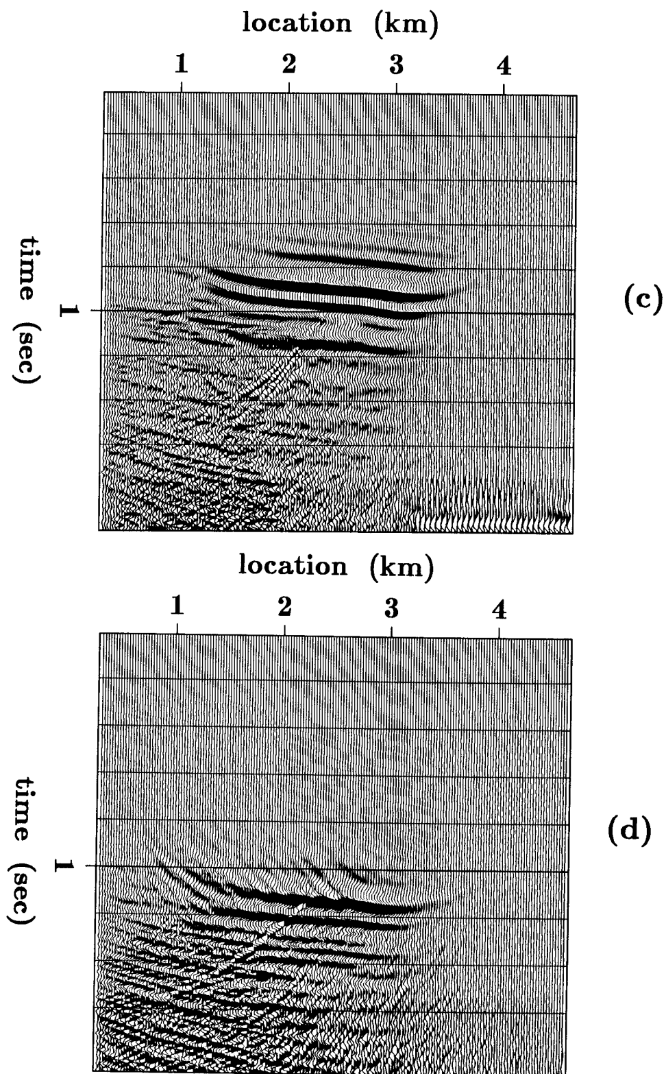
FIG. 8 (continued). Stacks of migrated profiles. (c) Migration velocity=1.6 km/sec. (d) Migration velocity=1.7 km/sec.
