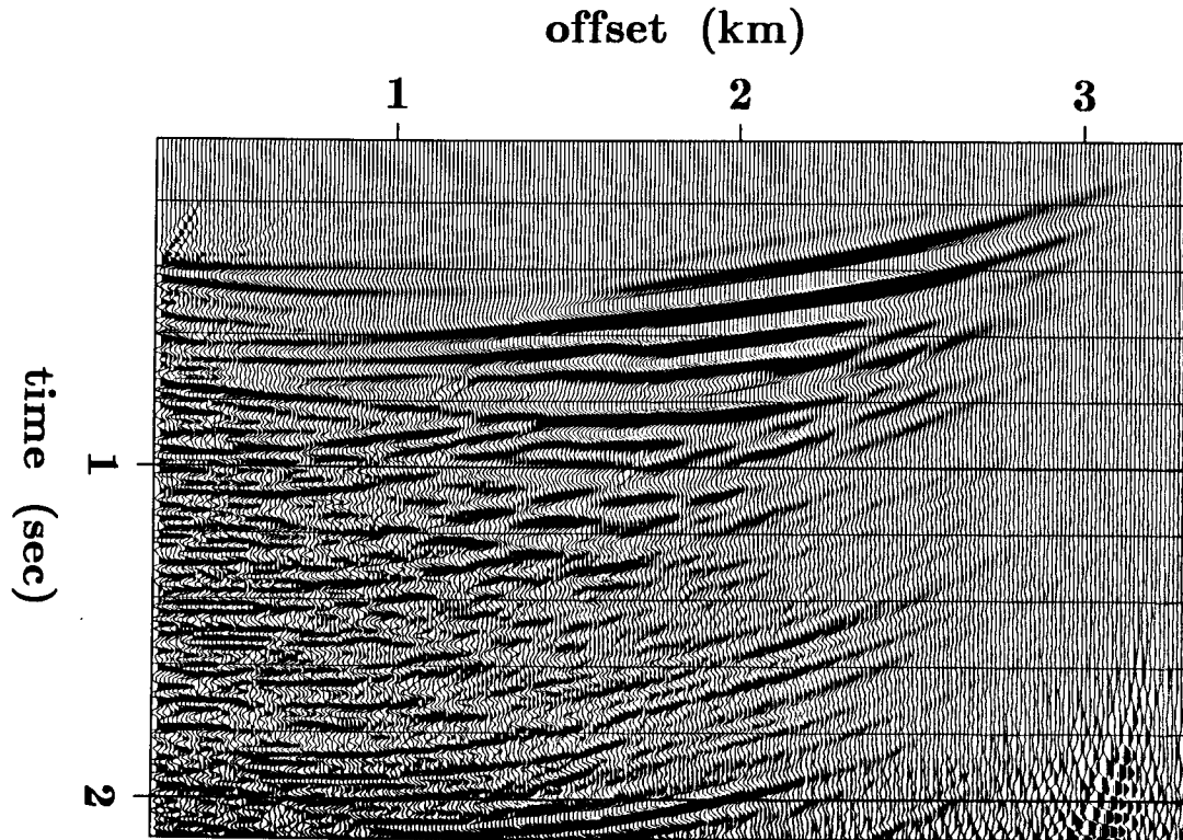
FIG. 2. The result of migrating the gather in Figure 1 with a velocity of 1.5 km/sec.
