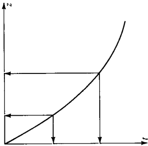
FIGURE 11-13 Plane for migration with depth-variable velocity. The curve in this plane is chosen to be the curve of two-way vertical travel time. The midpoint axis y comes out of the page. Section data along the curve may be projected to either the z axis or the t axis creating a migrated depth section or a migrated time section.
