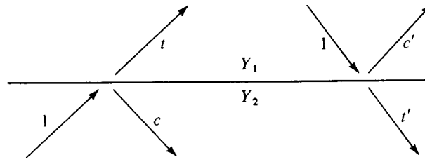
FIGURE 8-1 Waves incident, reflected c , and transmitted t at an interface.
