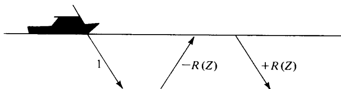
FIGURE 8-3 An initial downgoing disturbance 1 results in a later upgoing reflected wave -R(Z) which reflects back down as R(Z) . The pressure at the surface is D + U = 1 + R - R = 1 .
