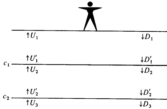
FIGURE 8-6 Goupillaud-type layered medium (layers have equal travel time).
