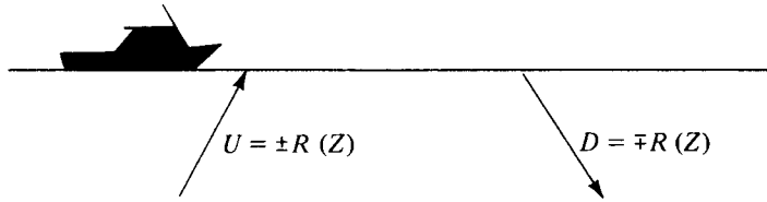
FIGURE 8-2 A waveform R(Z) reflecting at the surface of the sea. Pressure equal to U + D vanishes at the surface. The vertical velocity of the surface is proportional to D - U . Theoretically, waves are observed by measuring W at the surface; however, as a practical matter P is often observed a fraction of a wavelength below the surface.
