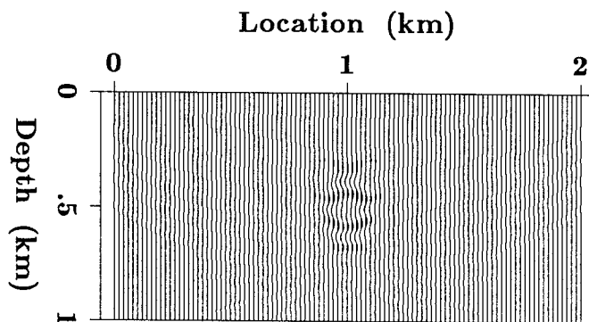
FIG. 9. (b) One-iteration inversion result plotted as the perturbation relative to the homogeneous starting model.
