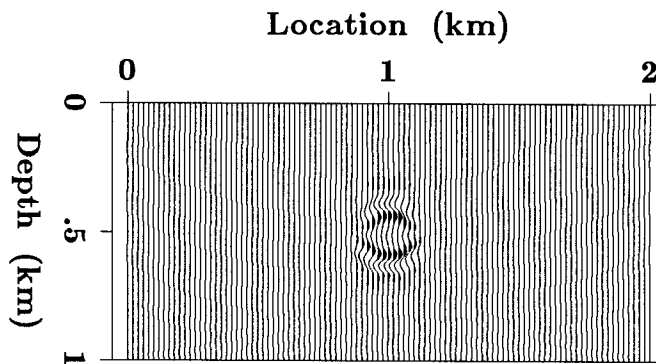
FIG. 9. (c) Fifteen-iteration inversion result plotted as the perturbation relative to the homogeneous starting model.
