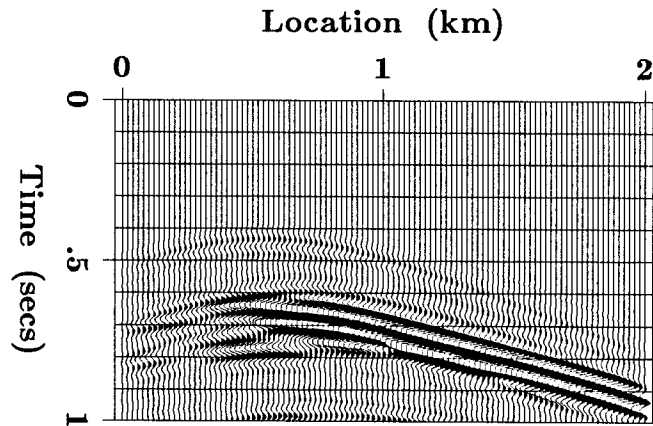
FIG. 6. Shot gather generated from the model shown in Figure 7 (a).
