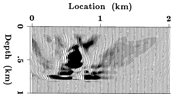
FIG. 7. (b) Ten iteration inversion result. The starting model was a layer over a halfspace that was identical to the true model except that that the circular velocity anomaly was not present.
