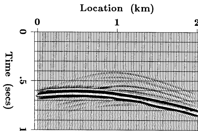
FIG. 10. Shot gather generated from the model shown in Figure 11 (a).
