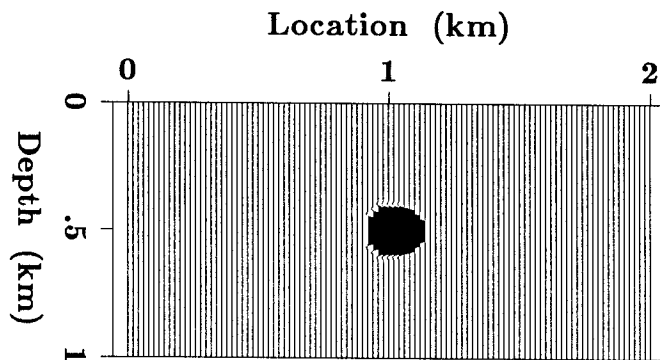
FIG. 9. (a) True model corresponding to the synthetic data shown in Figure 8. Black indicates a negative perturbation and white a positive perturbation relative to the acoustic impedance in the upper layer. The velocity perturbation of the circular region relative to the layer velocity was 10%.
