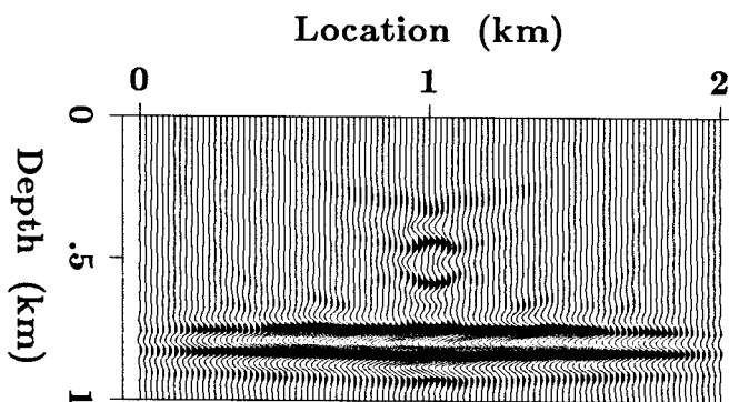
FIG. 11. (b) One-iteration inversion result plotted as the perturbation relative to the homogeneous starting model.
