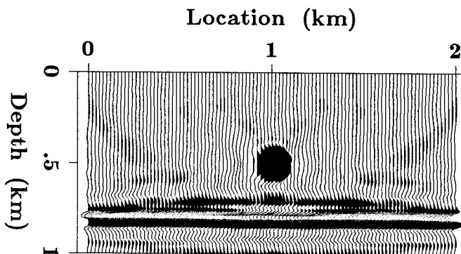
FIG. 11. (c) Fifteen-iteration inversion result plotted as the perturbation relative to the homogeneous starting model.
