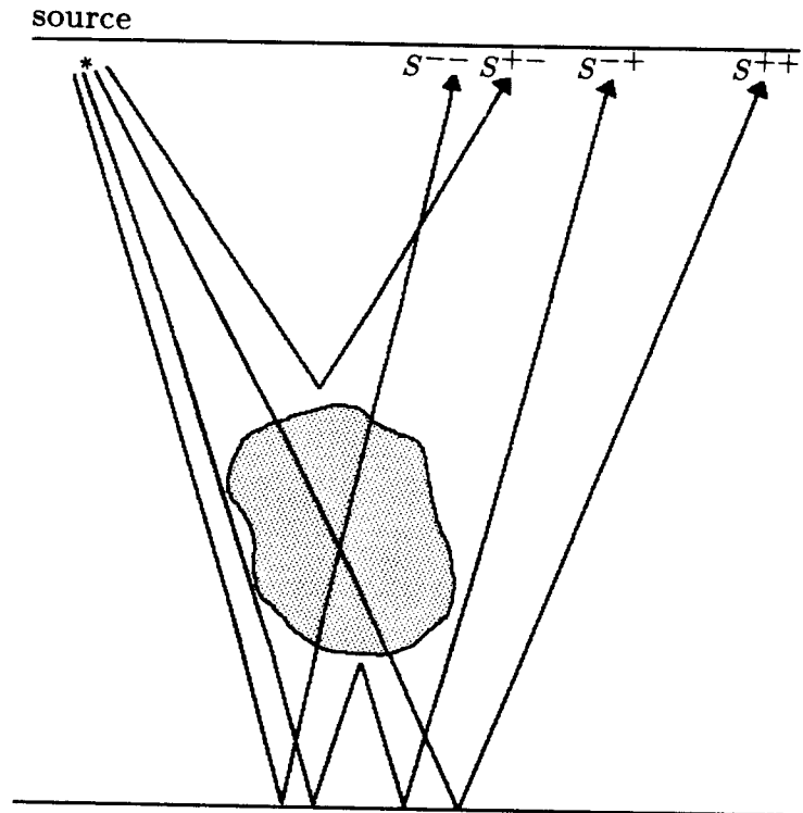
FIG. 2. Raypaths corresponding to the four different scattering terms. The first superscript refers to the incident ray direction while the second superscript refers to the scattered ray direction (+ is downward and - is upward). For example, S^{+-} has a downgoing incident ray and an upgoing scattered ray.
