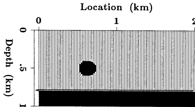
FIG. 7. (a) The true model corresponding to the synthetic data shown in Figure 6. Black indicates a negative perturbation and white a positive perturbation relative to the acoustic impedance in the upper layer. The velocity perturbation of the circular region relative to the layer velocity was 10%.
