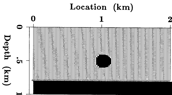
FIG. 11. (a) True model corresponding to the synthetic data shown in Figure 10. Black indicates a negative perturbation and white a positive perturbation relative to the velocity in the upper layer. The velocity perturbation of the circular region relative to the layer velocity was 10%.
