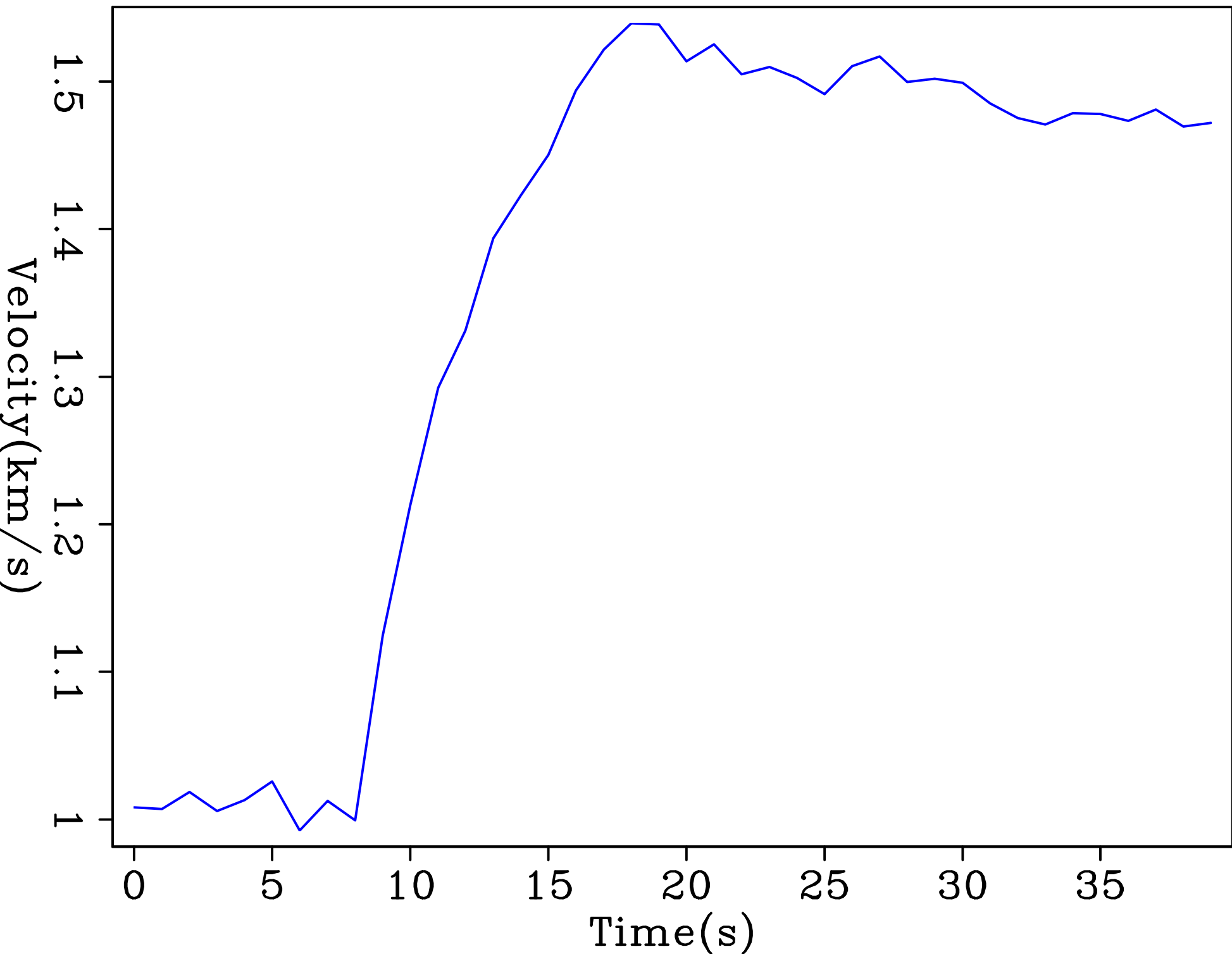
Input RMS velocity with noise
