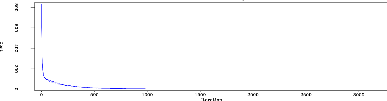
Smoothness: Residual of Laplacian
