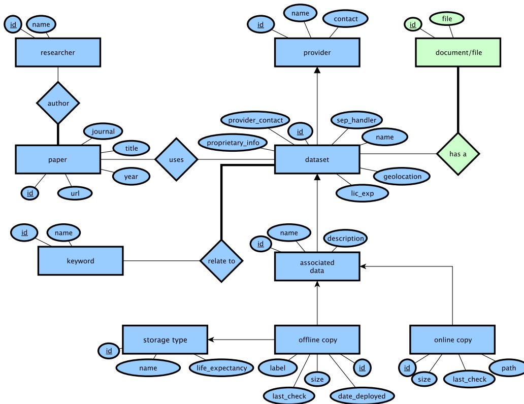
Figure 2: Entity-relation diagram of the SEP data catalog database. [NR]
