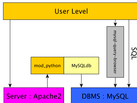
Figure 1: Software elements for the SEP data catalog. [NR]
