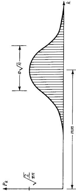
FIGURE 4-9 Coefficients of [Z^m(Z^\sigma + Z^{-\sigma})/2]^n .
