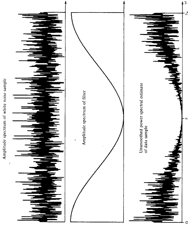
FIGURE 4-5 Spectral estimation.
